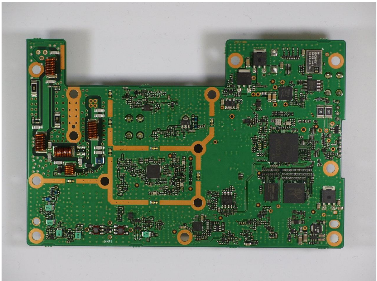
IC-F5400D/DS MAIN-A BOARD SIDE-B
