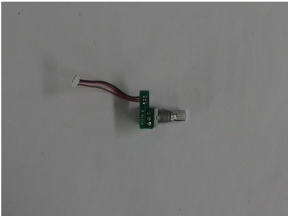
IC-F5400D/DS VR-C/D BOARD SIDE-B
