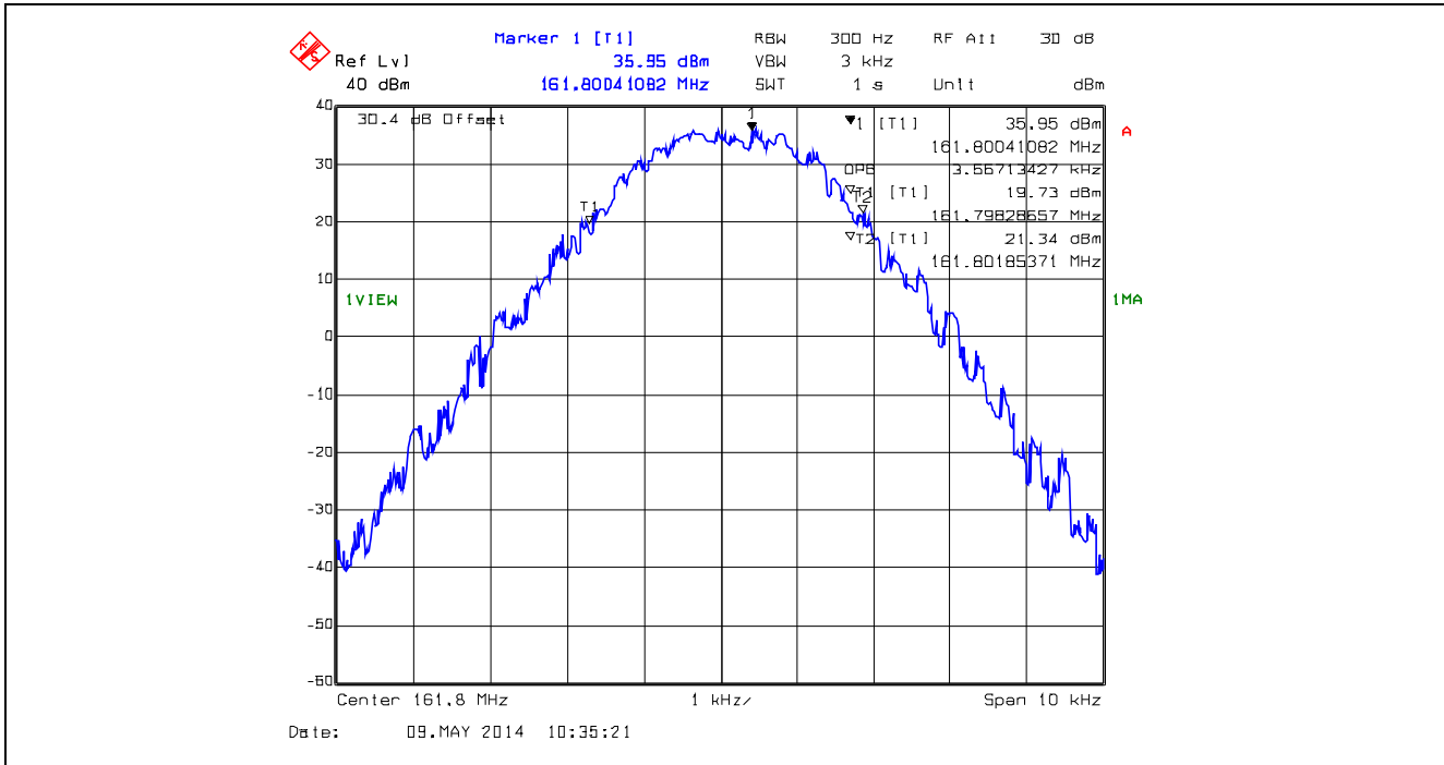
Plot 5.4.4.1.15. 99% Occupied Bandwidth for 6.25 kHz Channel Spacing, Digital 161.8 MHz, High Power
