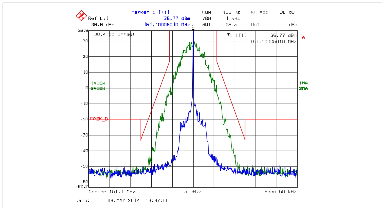
Plot 5.4.4.3.11. Emission Mask D, 151.1 MHz, Digital, High Power
