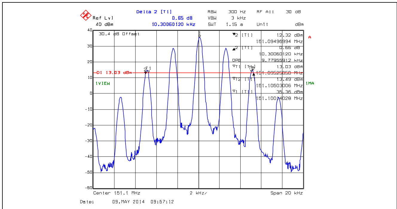
Plot 5.4.4.1.6. 99% Occupied Bandwidth for 12.5 kHz Channel Spacing, Analog 151.1 MHz, High Power, FM with 2.5 kHz sine wave signal
