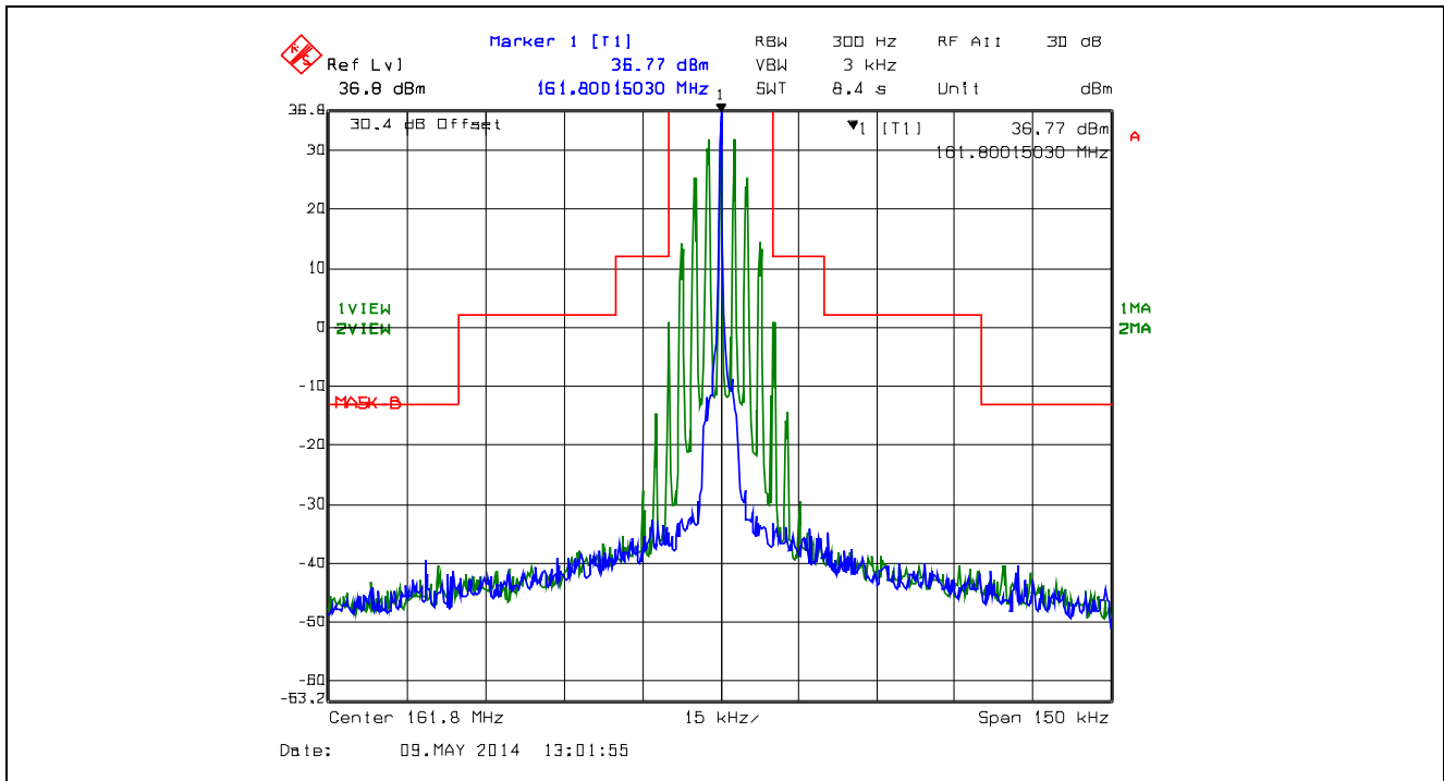
Plot 5.4.4.2.5. Emission Mask B, 161.8 MHz, Analog, High Power
