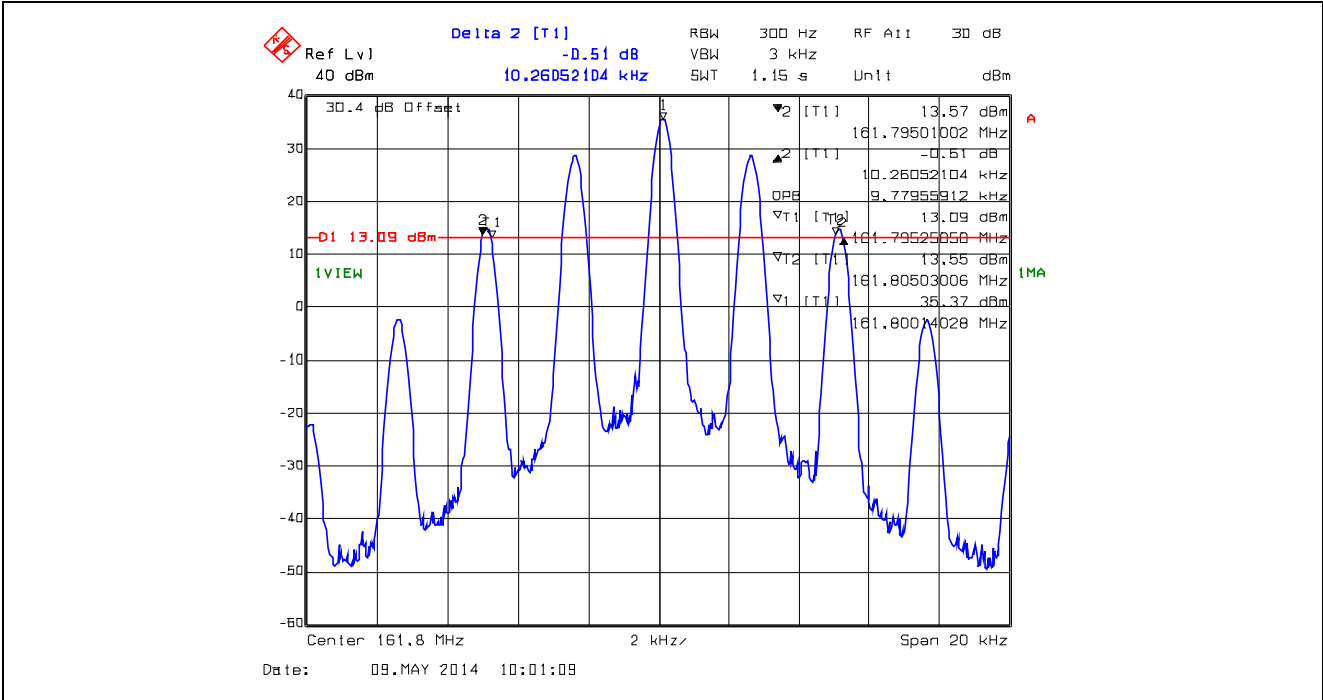
Plot 5.4.4.1.7. 99% Occupied Bandwidth for 12.5 kHz Channel Spacing, Analog 161.8 MHz, High Power, FM with 2.5 kHz sine wave signal
