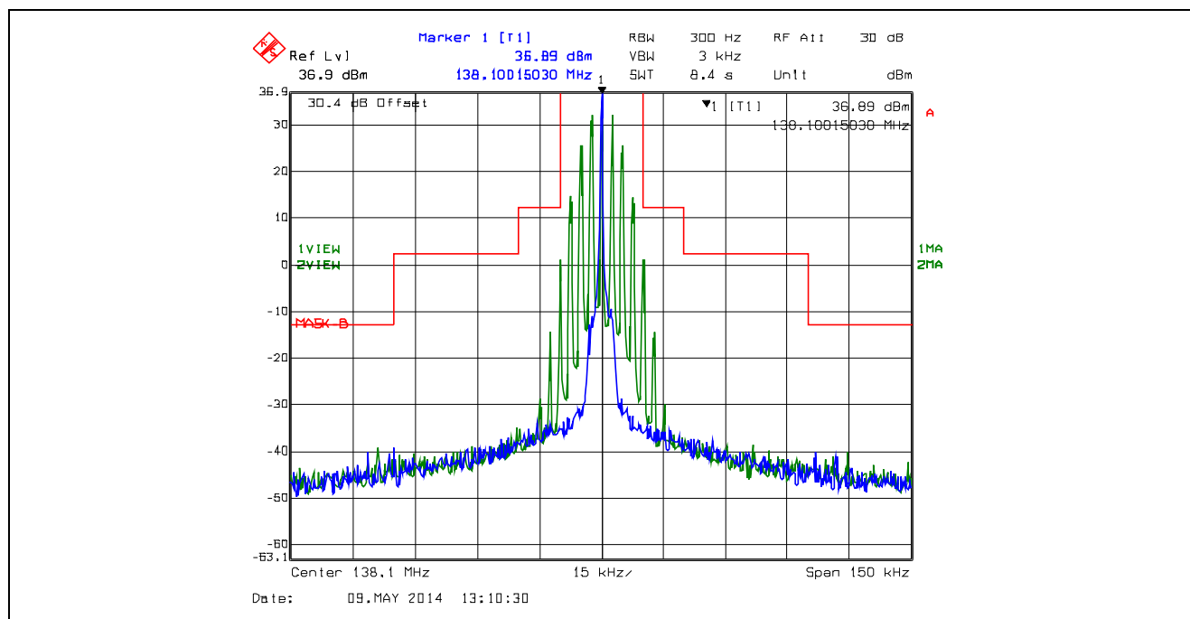
Plot 5.4.4.2.1. Emission Mask B, 138.1 MHz, Analog, High Power
