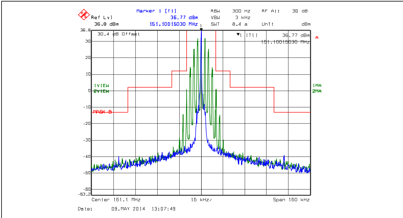
Plot 5.4.4.2.3. Emission Mask B, 151.1 MHz, Analog, High Power
