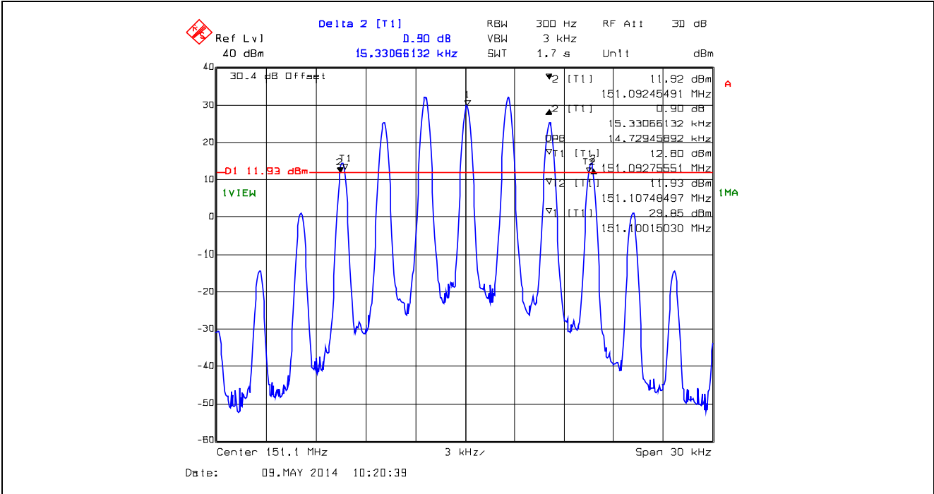
Plot 5.4.4.1.2. 99% Occupied Bandwidth for 25 kHz Channel Spacing, Analog 151.1 MHz, High Power, FM with 2.5 kHz sine wave signal
