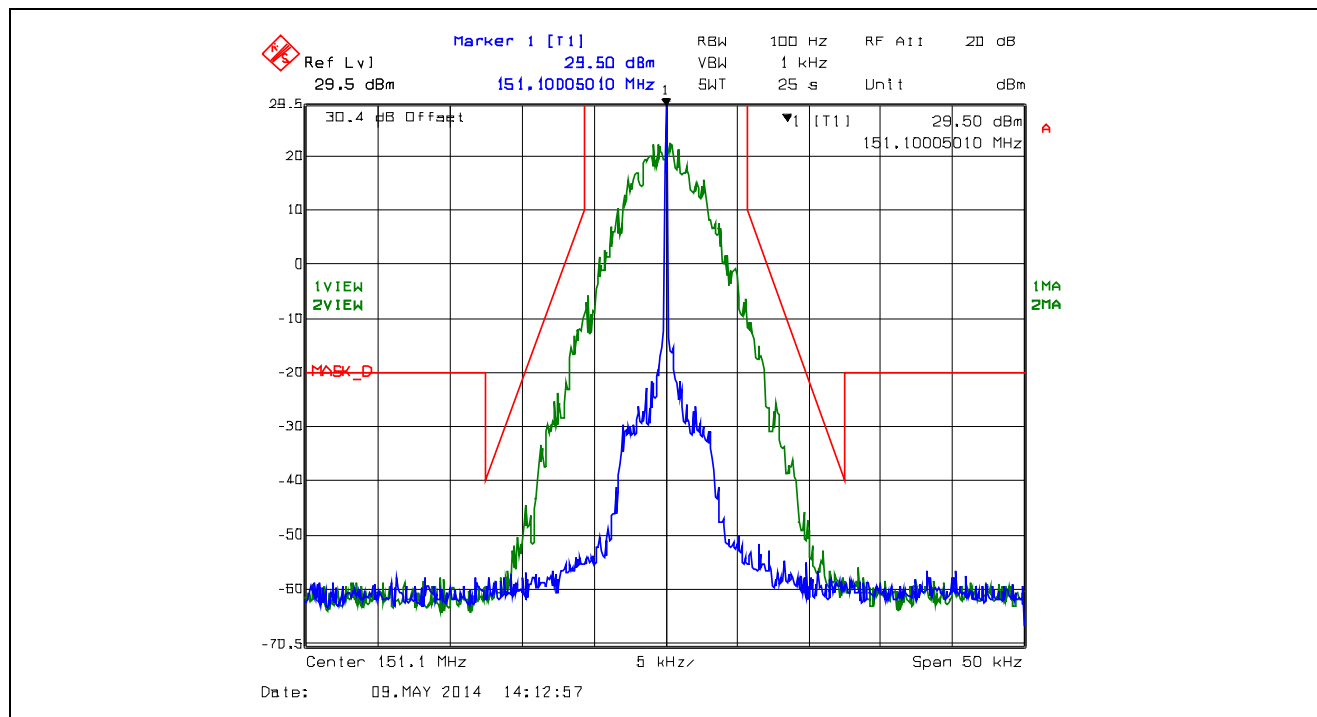
Plot 5.4.4.3.12. Emission Mask D, 151.1 MHz, Digital, Low Power
