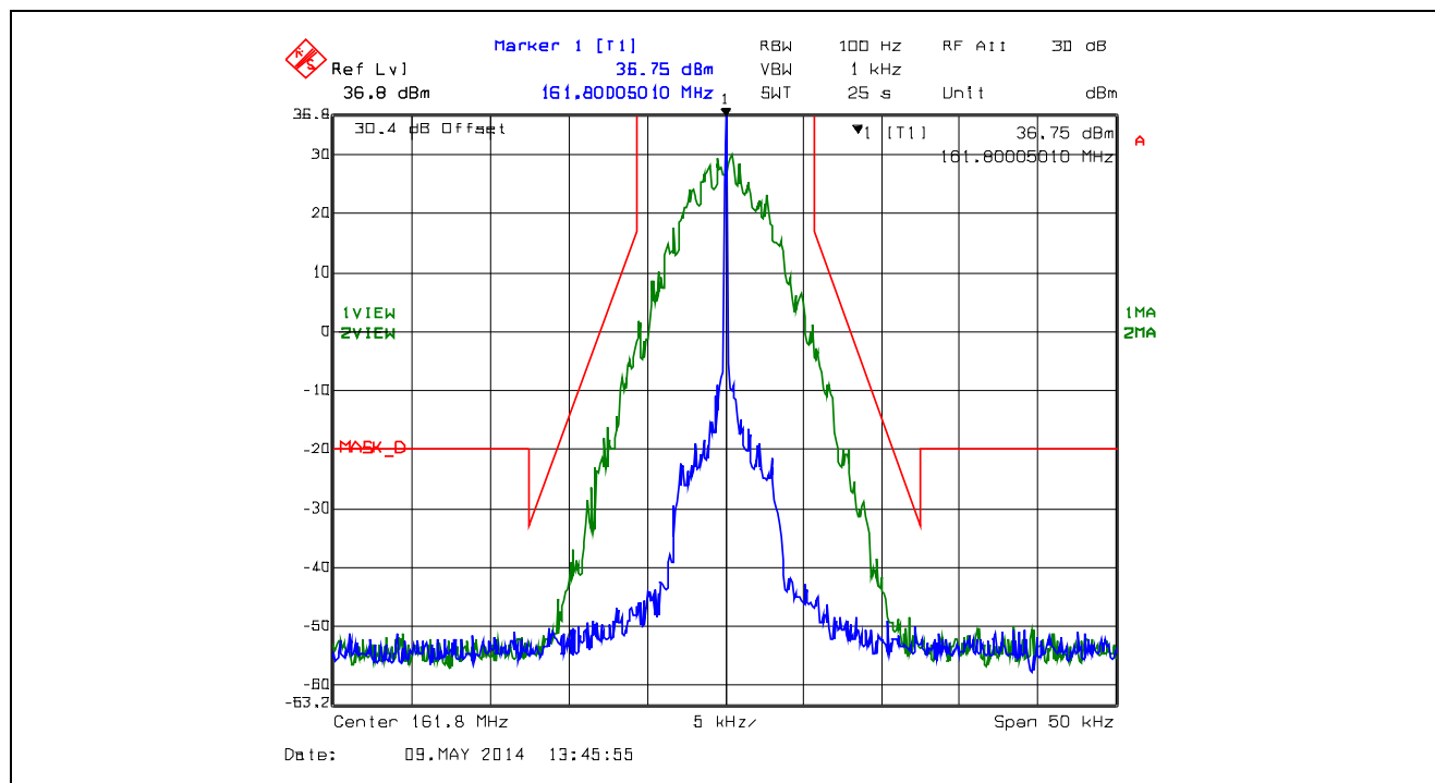
Plot 5.4.4.3.13. Emission Mask D, 161.8 MHz, Digital, High Power
