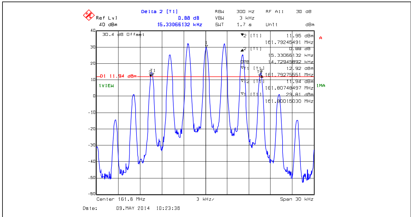
Plot 5.4.4.1.3. 99% Occupied Bandwidth for 25 kHz Channel Spacing, Analog 161.8 MHz, High Power, FM with 2.5 kHz sine wave signal
