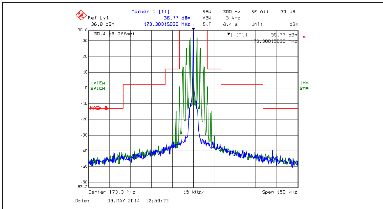
Plot 5.4.4.2.7. Emission Mask B, 173.3 MHz, Analog, High Power
