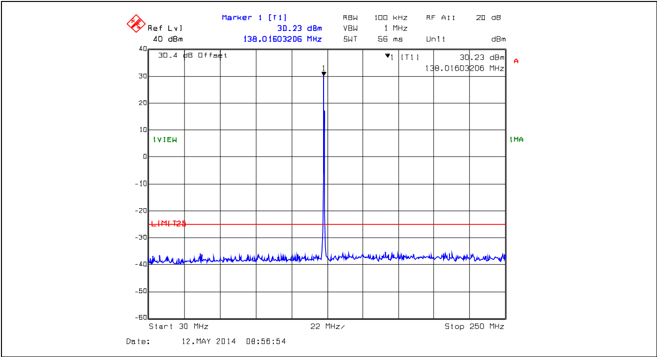
Plot 5.5.4.3. Conducted Transmitter Spurious Emissions, 138.1 MHz, Low Power, 30 MHz – 250 MHz
