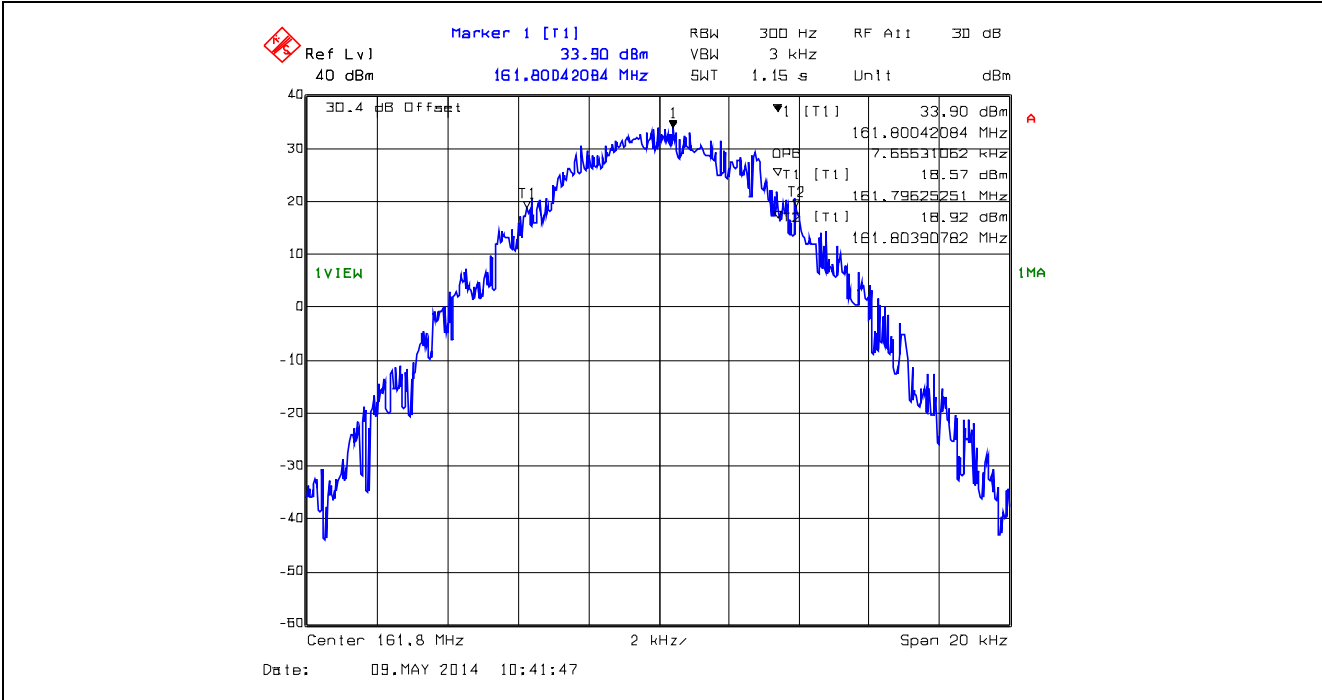
Plot 5.4.4.1.11. 99% Occupied Bandwidth for 12.5 kHz Channel Spacing, Digital 161.8 MHz, High Power
