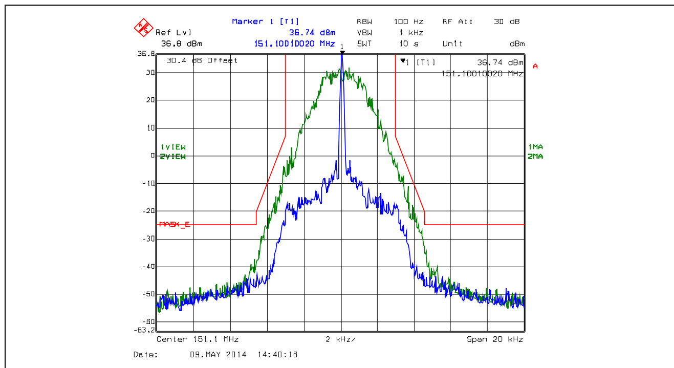
Plot 5.4.4.4.3. Emission Mask E, 151.1 MHz, Digital, High Power
