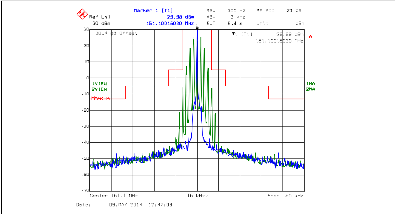
Plot 5.4.4.2.4. Emission Mask B, 151.1 MHz, Analog, Low Power
