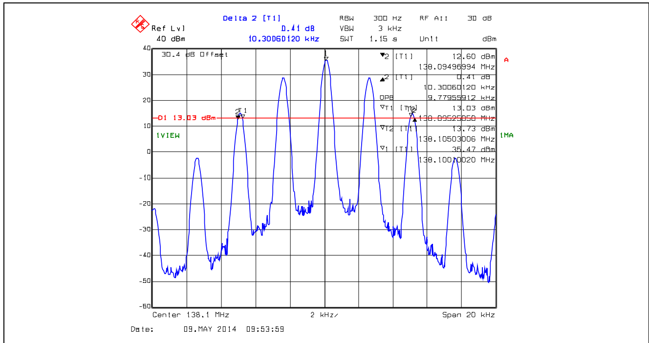
Plot 5.4.4.1.5. 99% Occupied Bandwidth for 12.5 kHz Channel Spacing, Analog 138.1 MHz, High Power, FM with 2.5 kHz sine wave signal
