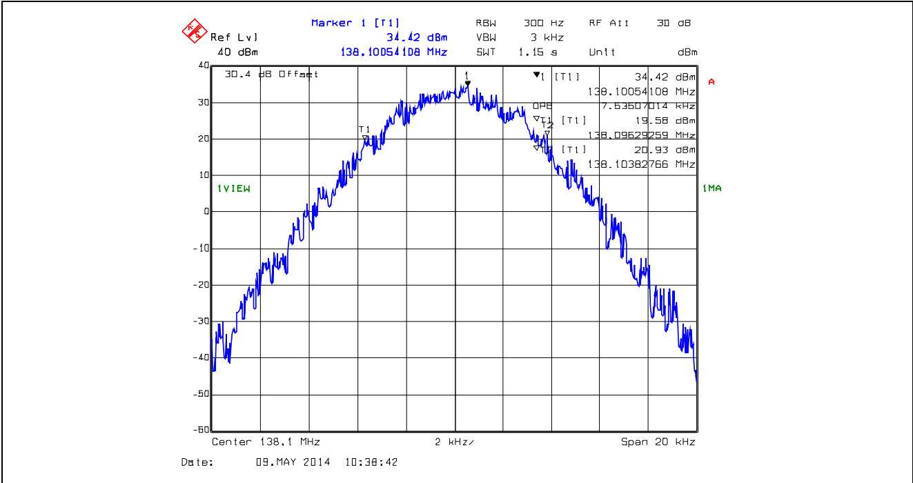
Plot 5.4.4.1.9. 99% Occupied Bandwidth for 12.5 kHz Channel Spacing, Digital 138.1 MHz, High Power
