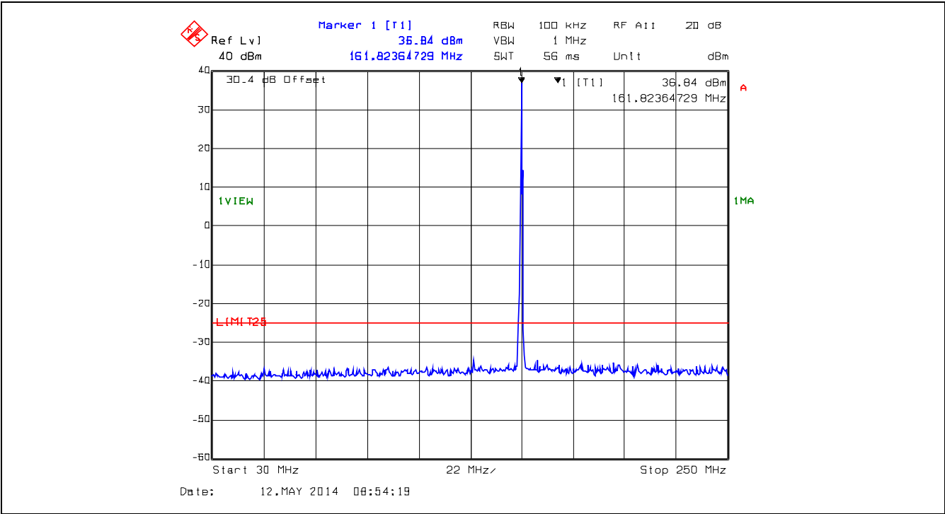
Plot 5.5.4.9. Conducted Transmitter Spurious Emissions, 161.8 MHz, High Power, 30 MHz – 250 MHz
