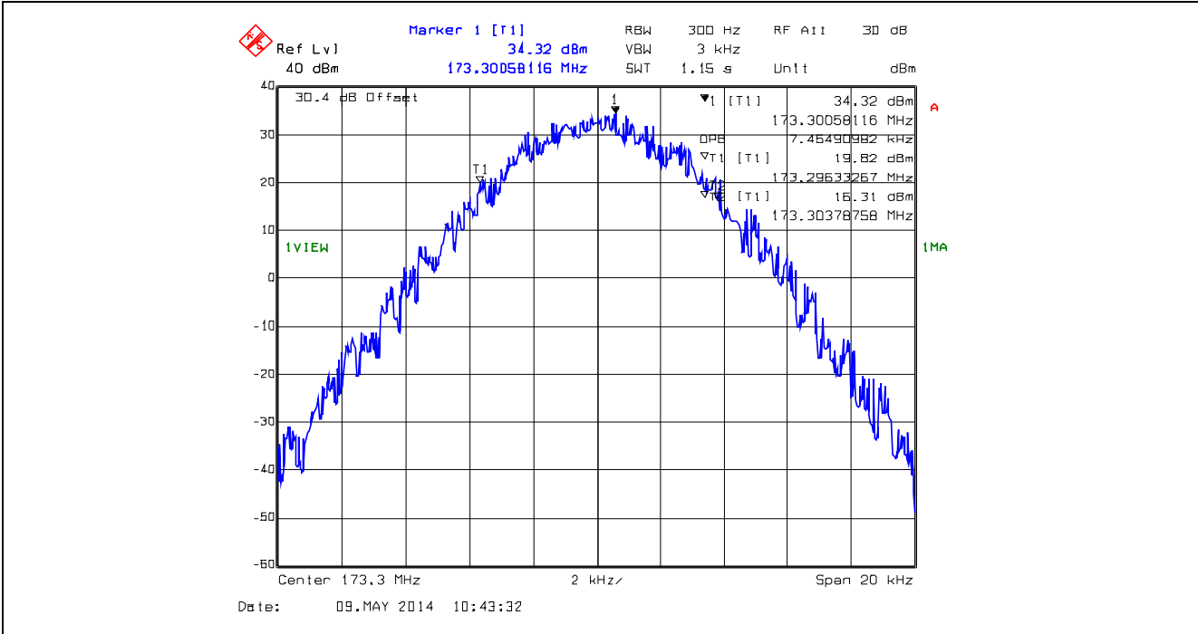
Plot 5.4.4.1.12. 99% Occupied Bandwidth for 12.5 kHz Channel Spacing, Digital 173.3 MHz, High Power
