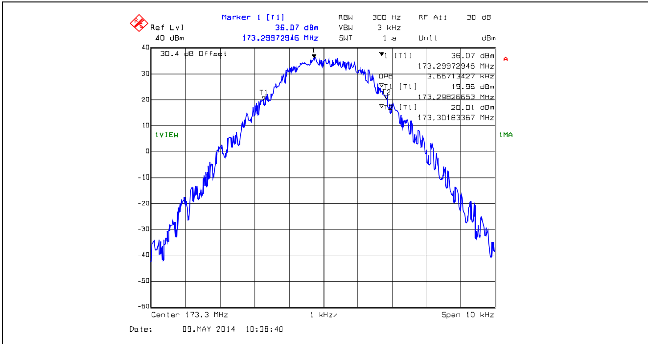
Plot 5.4.4.1.16. 99% Occupied Bandwidth for 6.25 kHz Channel Spacing, Digital 173.3 MHz, High Power
