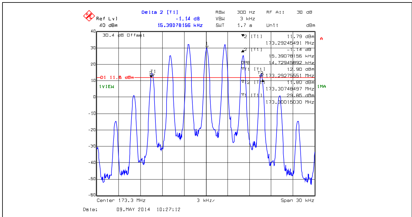
Plot 5.4.4.1.4. 99% Occupied Bandwidth for 25 kHz Channel Spacing, Analog 173.3 MHz, High Power, FM with 2.5 kHz sine wave signal
