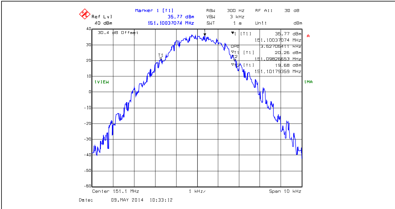
Plot 5.4.4.1.14. 99% Occupied Bandwidth for 6.25 kHz Channel Spacing, Digital 151.1 MHz, High Power
