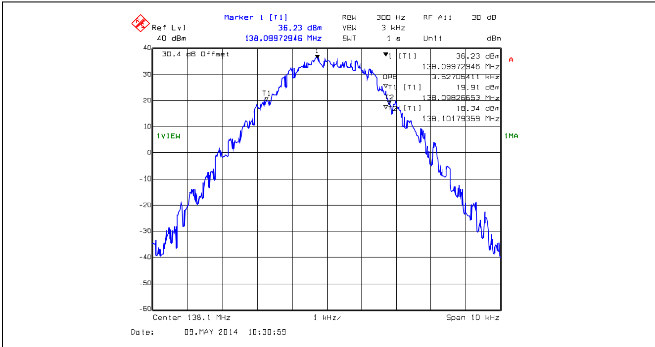
Plot 5.4.4.1.13. 99% Occupied Bandwidth for 6.25 kHz Channel Spacing, Digital 138.1 MHz, High Power
