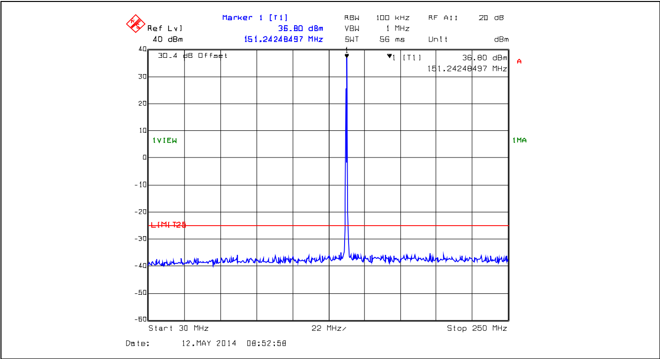
Plot 5.5.4.5. Conducted Transmitter Spurious Emissions, 151.1 MHz, High Power, 30 MHz – 250 MHz
