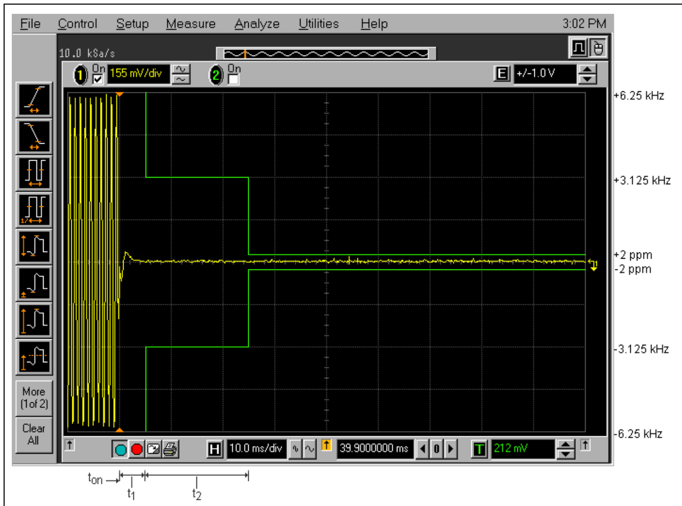
Plot 5.8.4.5. Transient Frequency Behavior for 6.25 kHz Channel Spacing 138.1 MHz, High Power Setting, Switch on condition t_{on} , t_1 , and t_2
