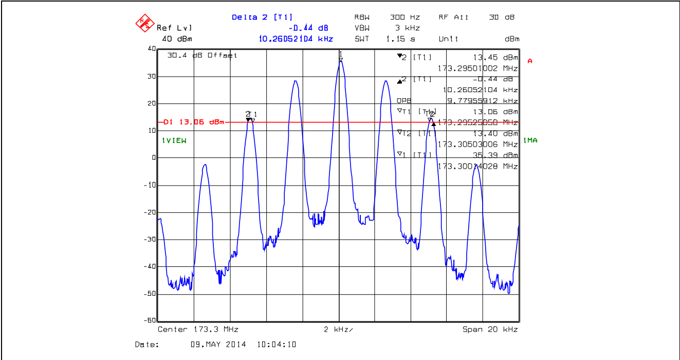
Plot 5.4.4.1.8. 99% Occupied Bandwidth for 12.5 kHz Channel Spacing, Analog 173.3 MHz, High Power, FM with 2.5 kHz sine wave signal
