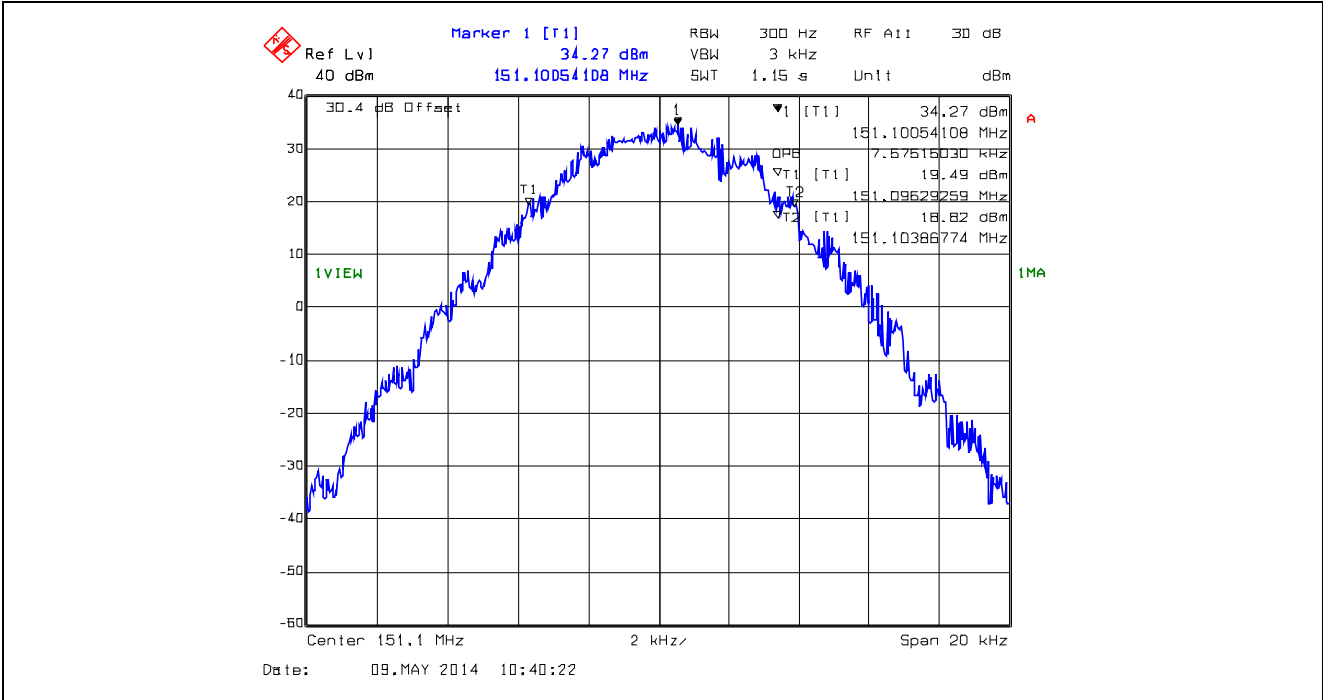
Plot 5.4.4.1.10. 99% Occupied Bandwidth for 12.5 kHz Channel Spacing, Digital 151.1 MHz, High Power
