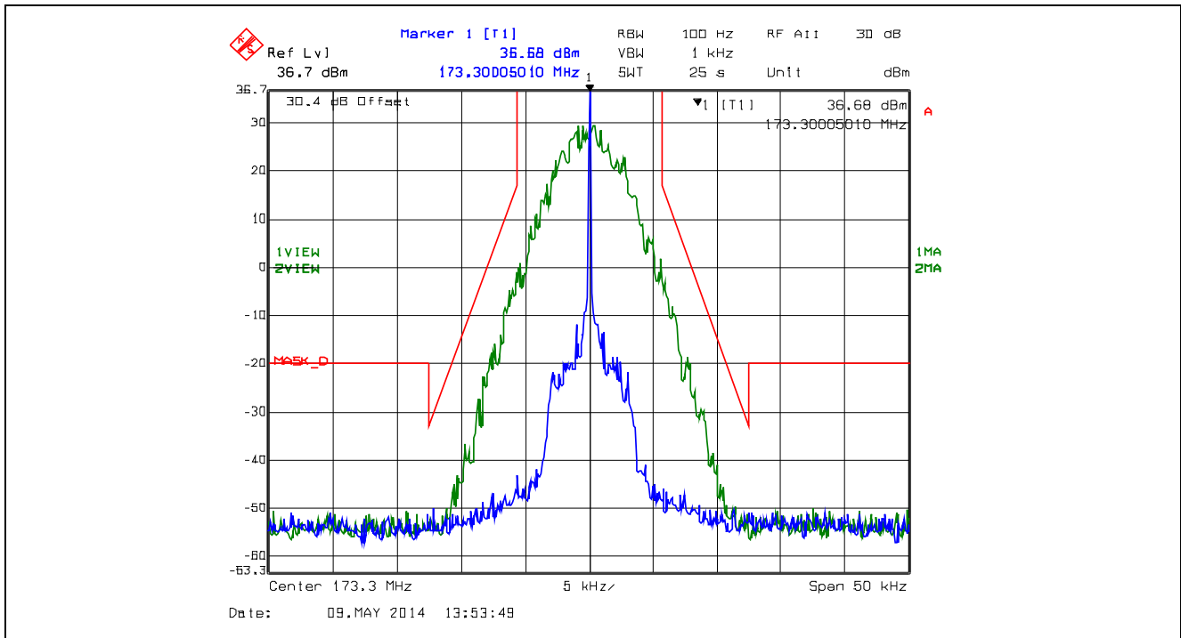
Plot 5.4.4.3.15. Emission Mask D, 173.3 MHz, Digital, High Power
