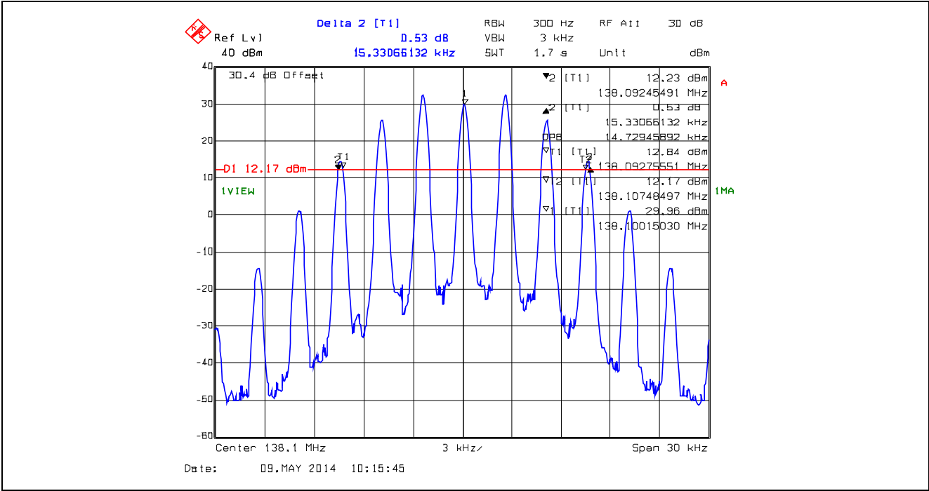
Plot 5.4.4.1.1. 99% Occupied Bandwidth for 25 kHz Channel Spacing, Analog 138.1 MHz, High Power, FM with 2.5 kHz sine wave signal
