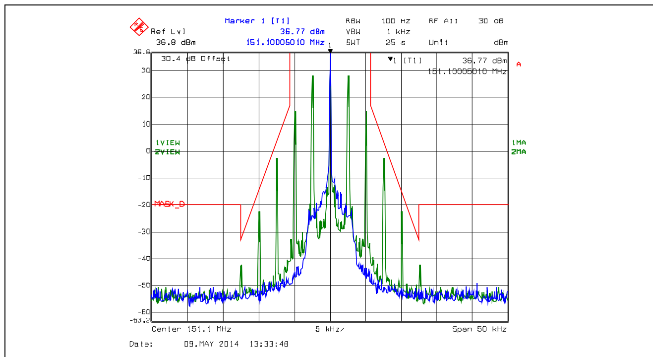
Plot 5.4.4.3.3. Emission Mask D, 151.1 MHz, Analog, High Power
