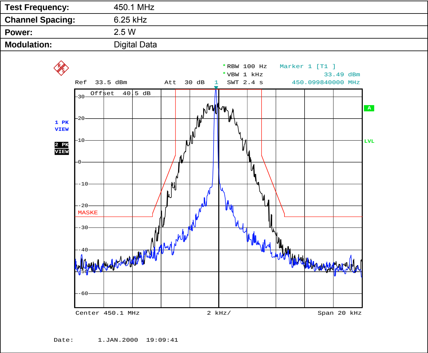
Plot 5.7.4.3.5. Emission Mask E, Low Power
