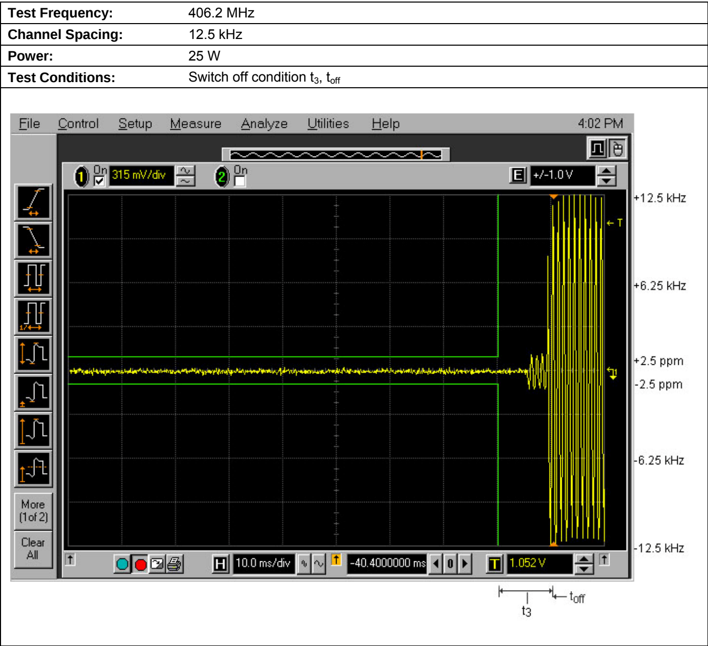
Plot 5.11.4.2. Transient Frequency Behavior for 12.5 kHz Channel Spacing
