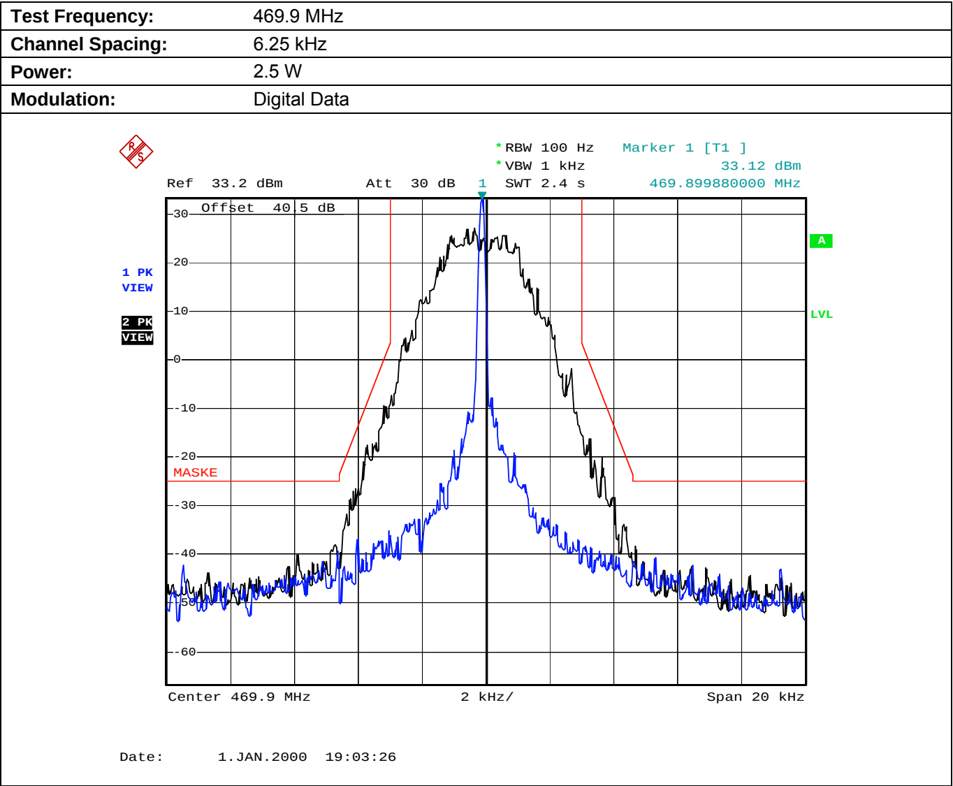
Plot 5.7.4.3.6. Emission Mask E, Low Power
