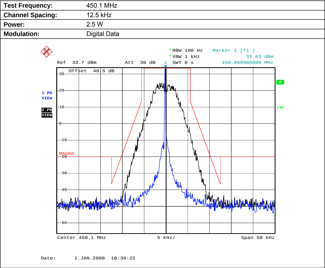
Plot 5.7.4.2.5. Emission Mask D, Low Power
