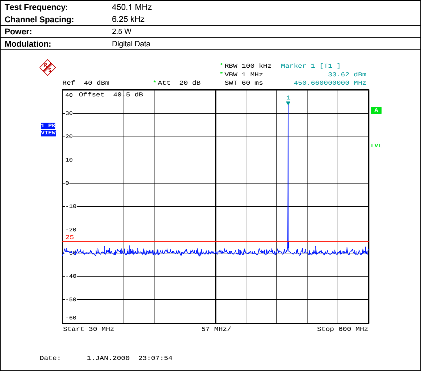
Plot 5.8.4.2.3. Conducted Transmitter Spurious Emissions for 450.1 MHz, Low Power, 30 MHz - 600 MHz
