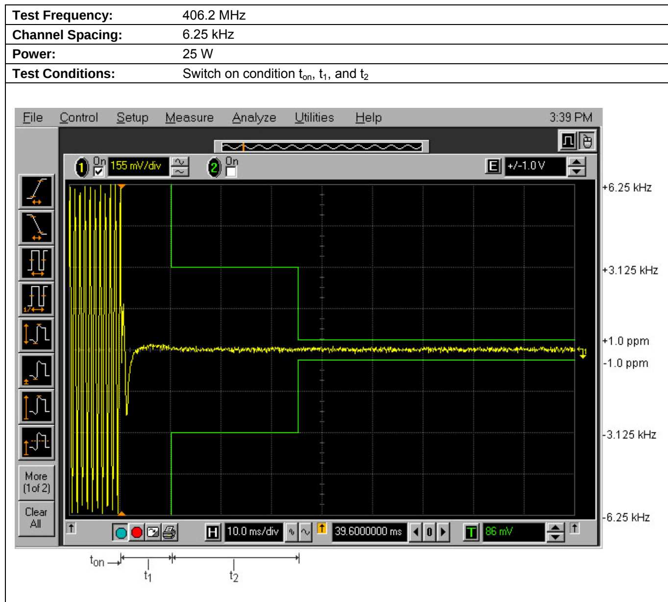
Plot 5.11.4.3. Transient Frequency Behavior for 6.25 kHz Channel Spacing
