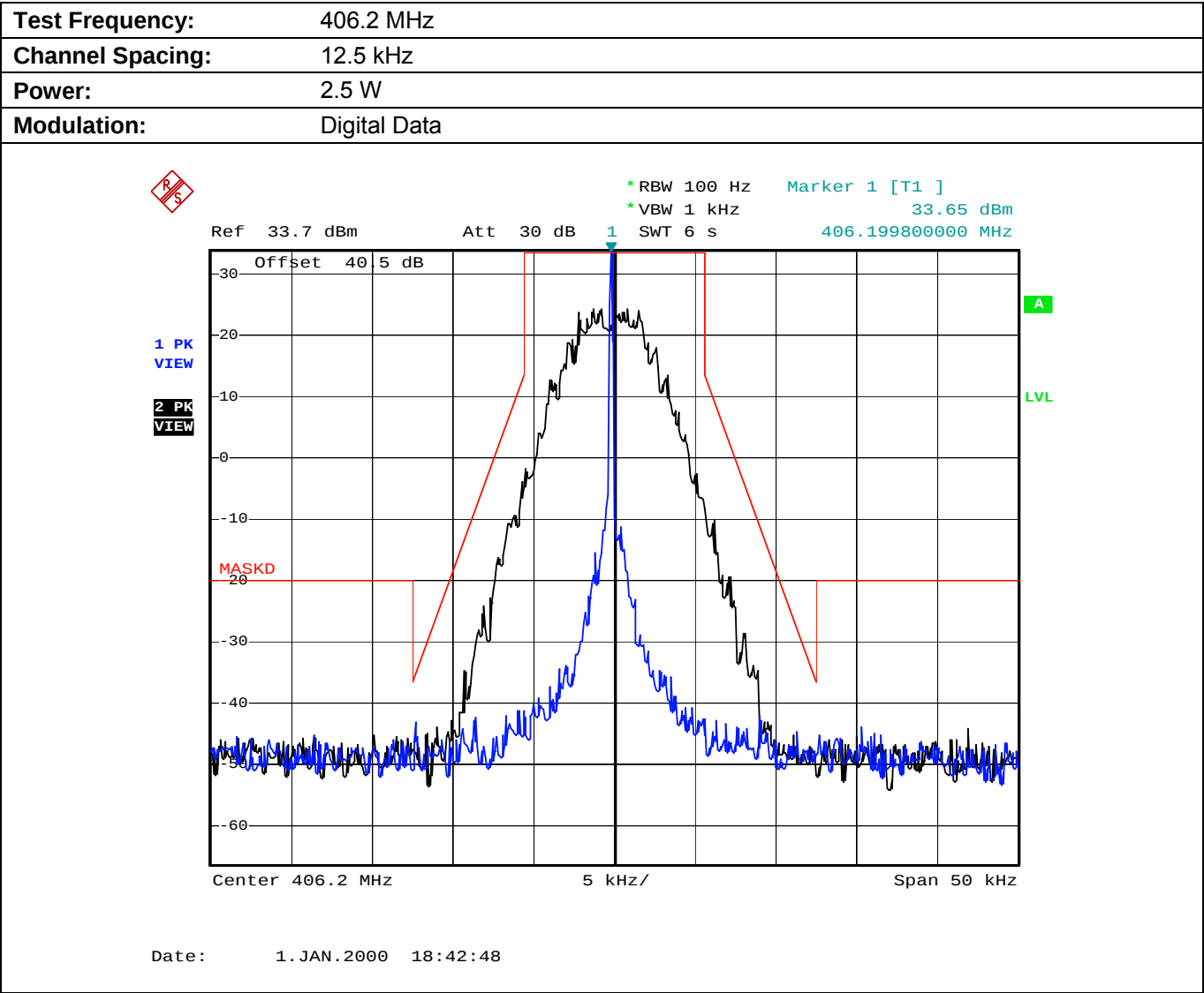
Plot 5.7.4.2.4. Emission Mask D, Low Power
