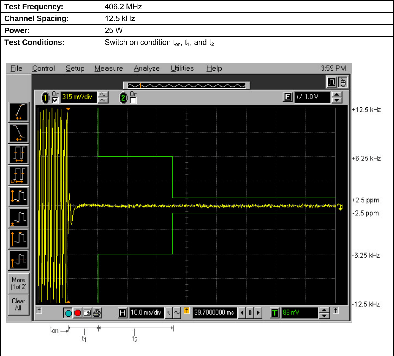
Plot 5.11.4.1. Transient Frequency Behavior for 12.5 kHz Channel Spacing
