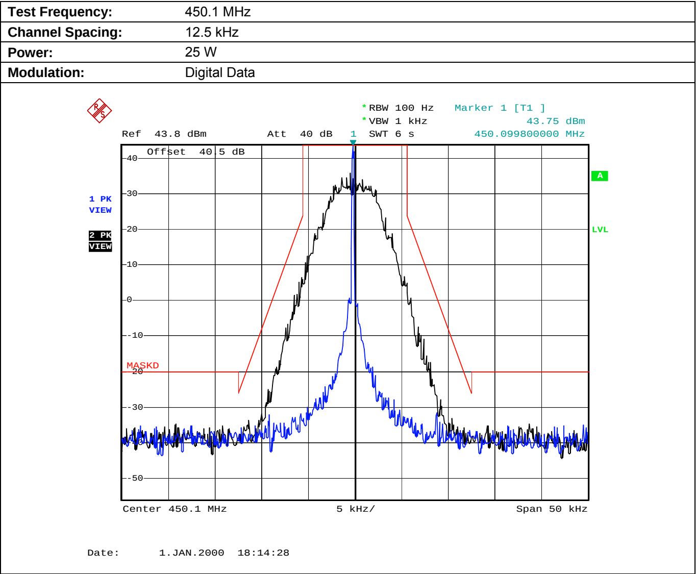
Plot 5.7.4.2.2. Emission Mask D, High Power
