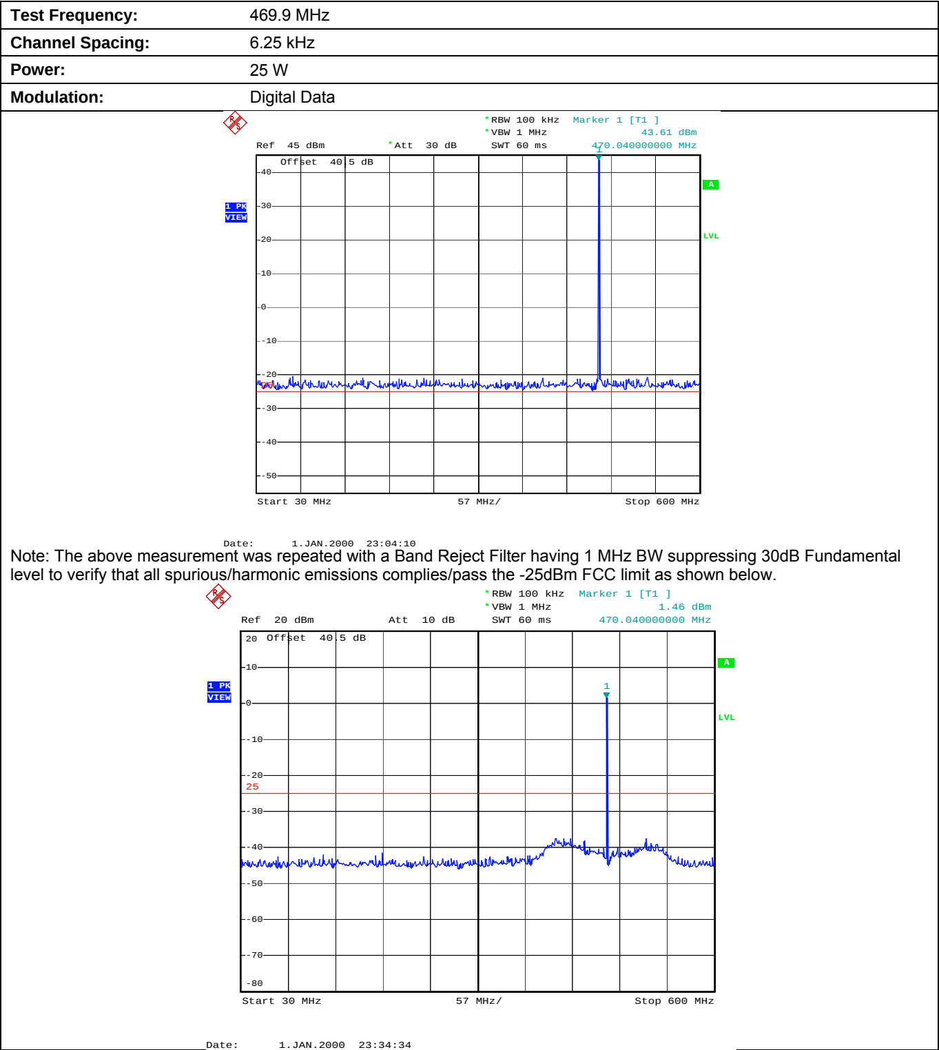
Plot 5.8.4.3.1. Conducted Transmitter Spurious Emissions for 469.9 MHz, High Power, 30 MHz - 600 MHz
