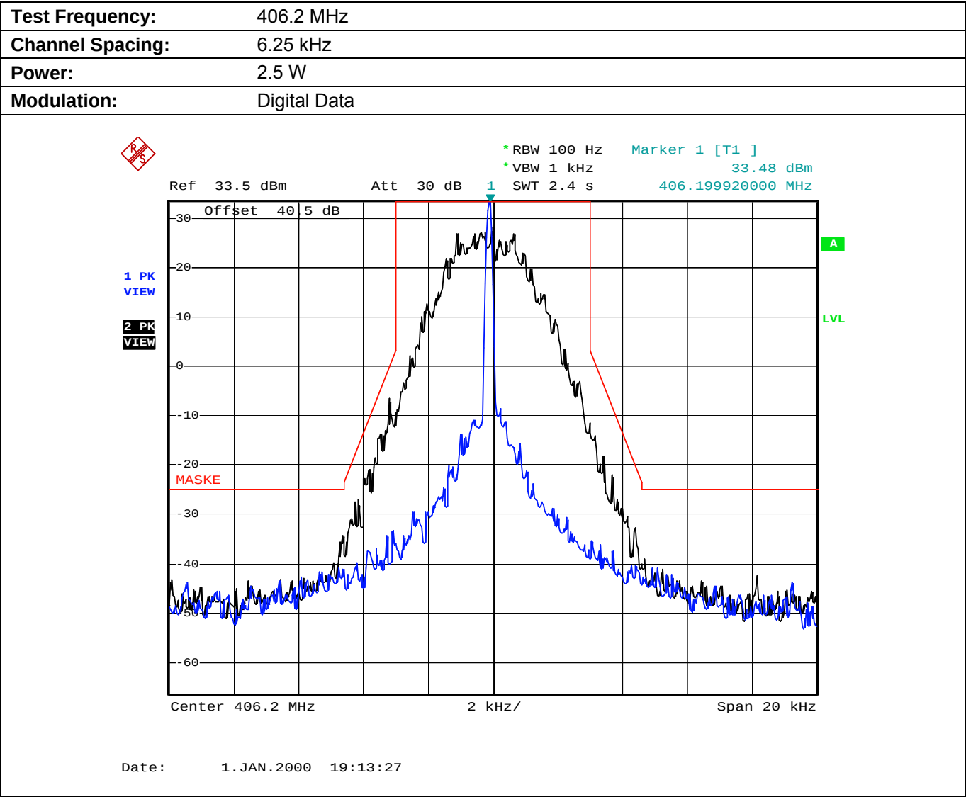
Plot 5.7.4.3.4. Emission Mask E, Low Power
