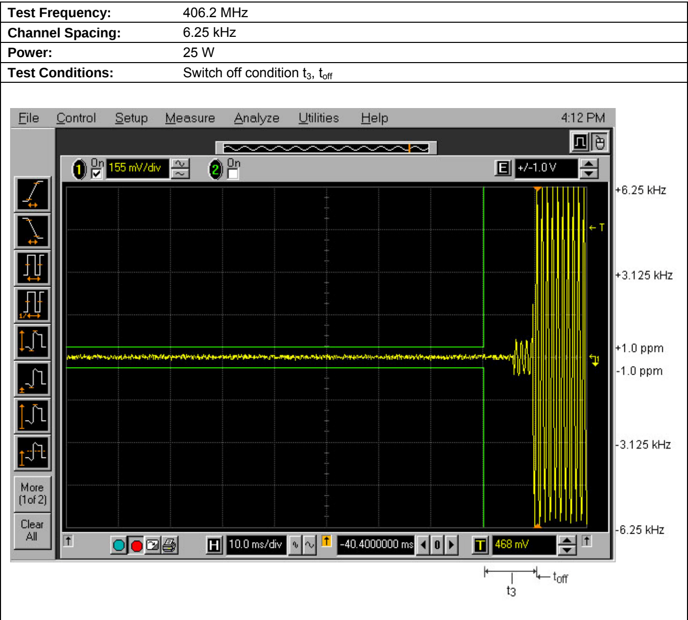
Plot 5.11.4.4. Transient Frequency Behavior for 6.25 kHz Channel Spacing
