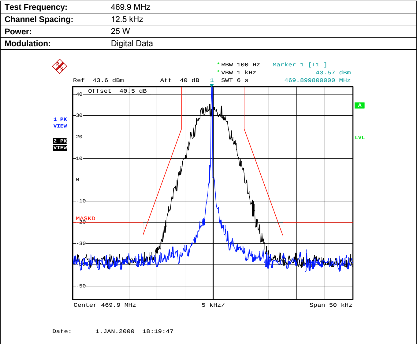
Plot 5.7.4.2.3. Emission Mask D, High Power
