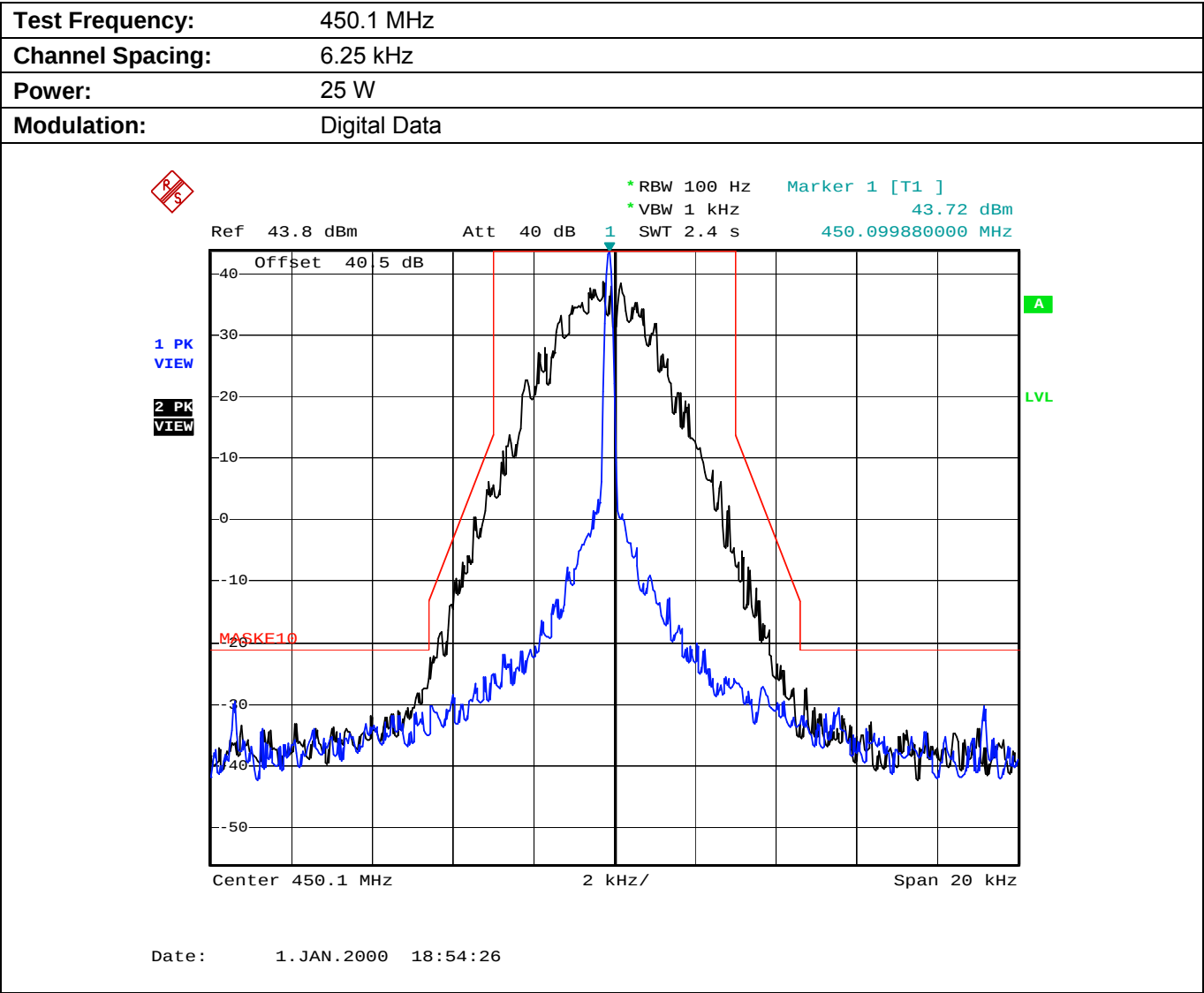
Plot 5.7.4.3.2. Emission Mask E, High Power
