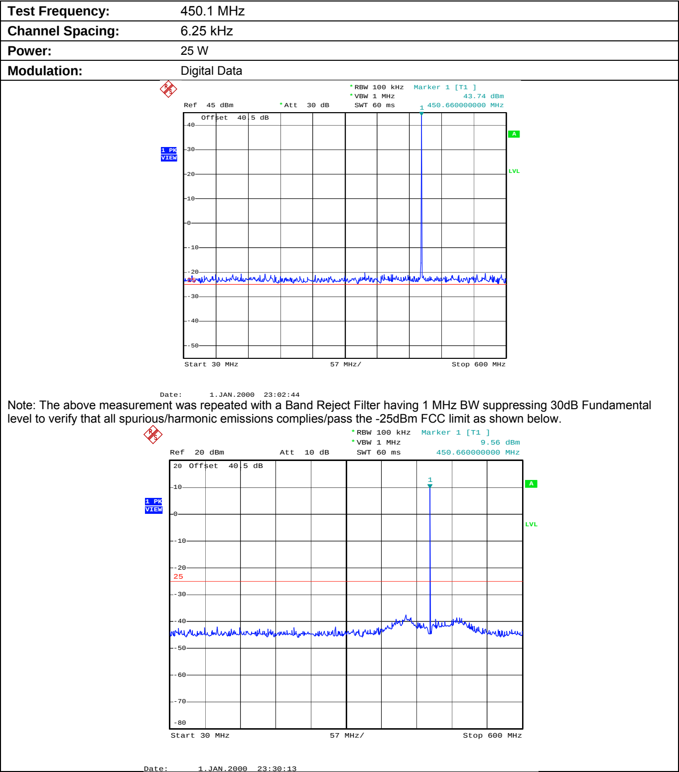
Plot 5.8.4.2.1. Conducted Transmitter Spurious Emissions for 450.1 MHz, High Power, 30 MHz - 600 MHz
