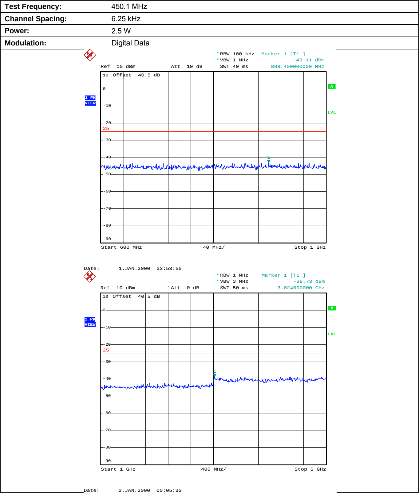
Plot 5.8.4.2.4. Conducted Transmitter Spurious Emissions for 450.1 MHz, Low Power, 600 MHz - 5 GHz
