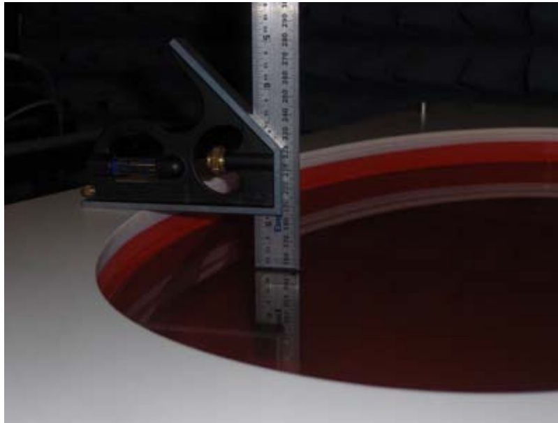
< Phantom filled with head tissue: liquid level = 150\text{mm} \pm 5\text{mm} >
