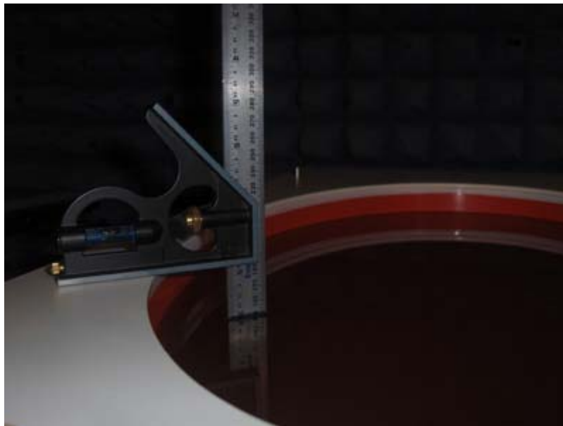
< Phantom filled with body tissue liquid: liquid level = 150\text{mm} \pm 5\text{mm} >
