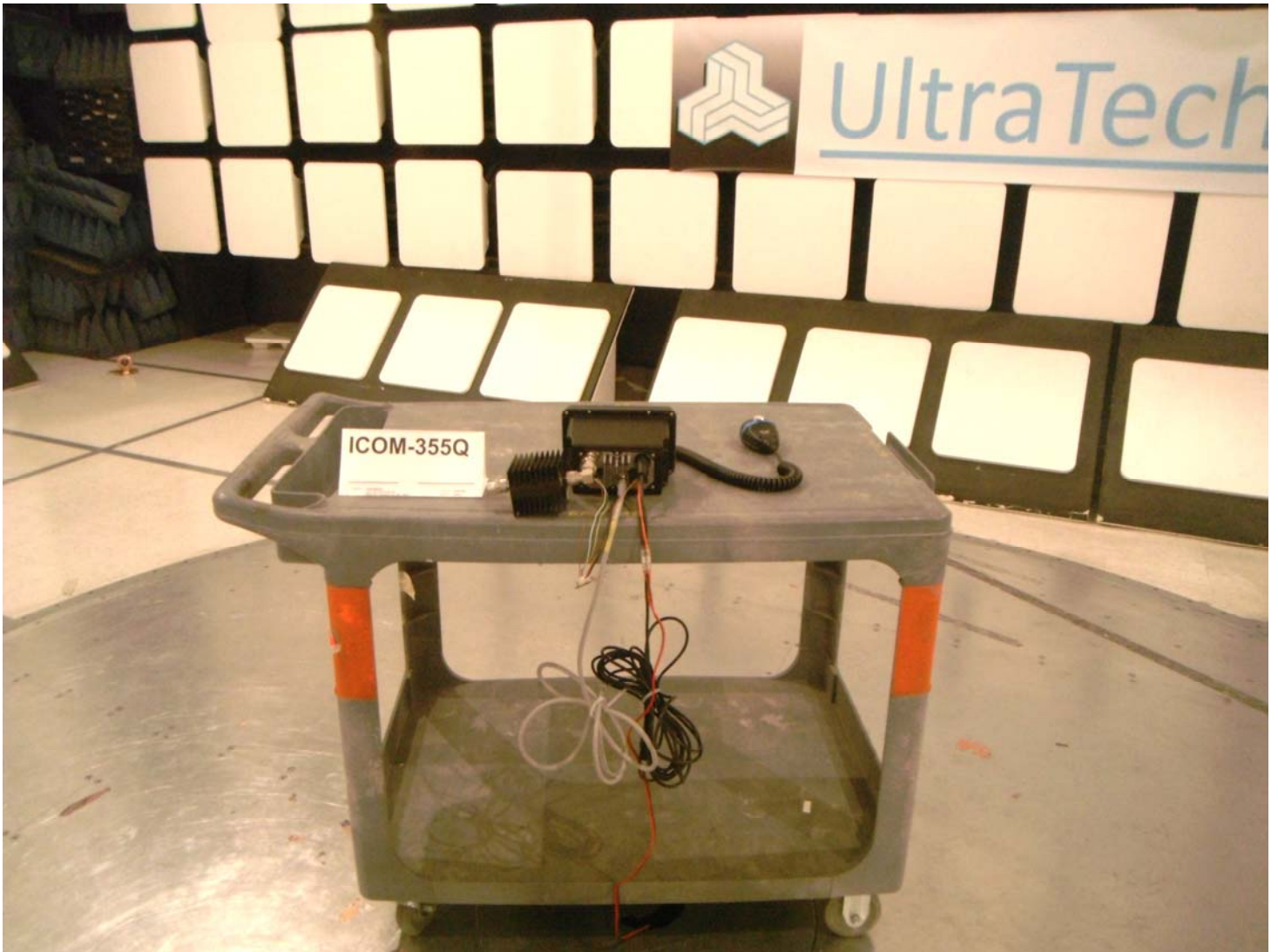
Radiated Emission at 3m
