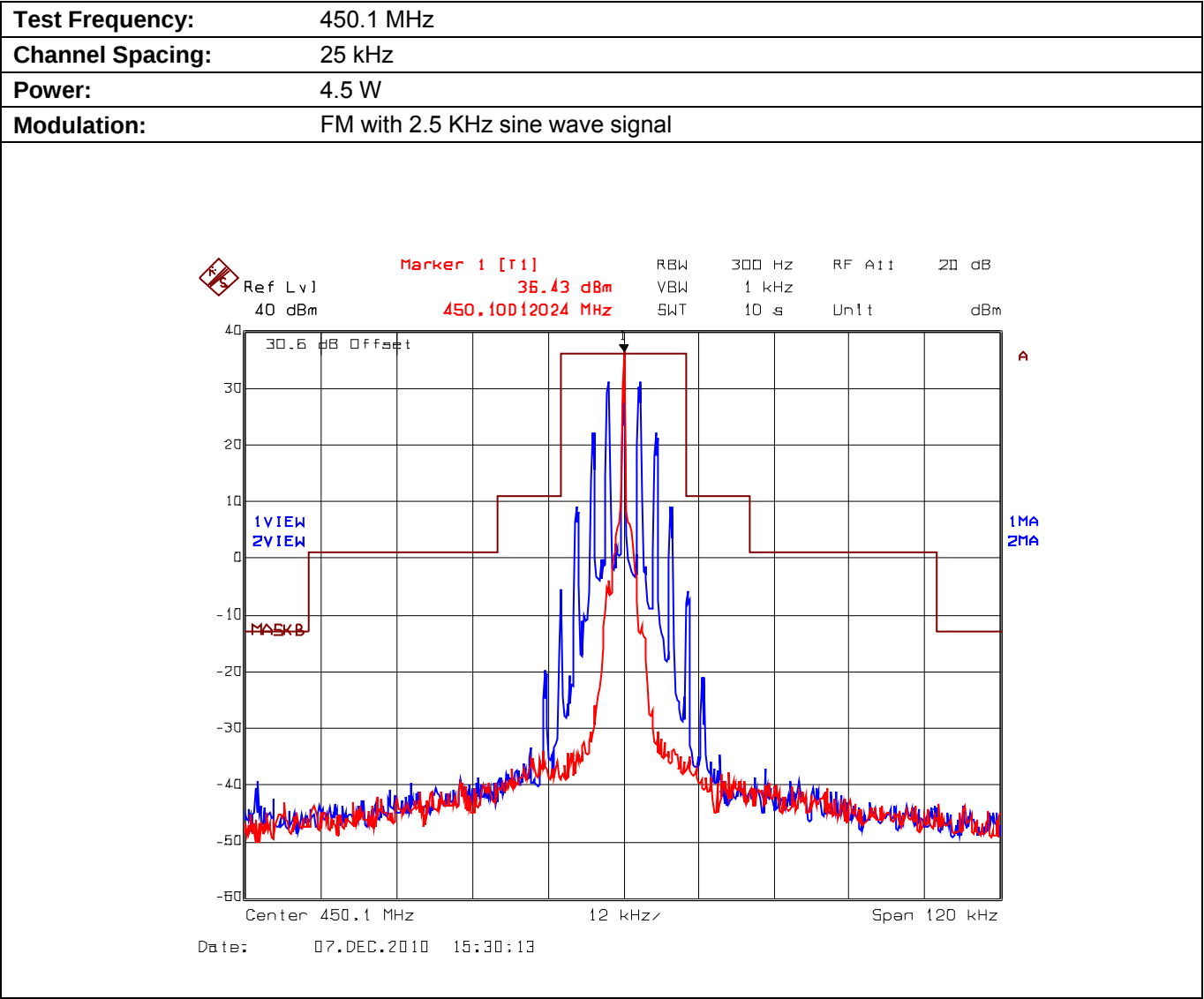
Plot 5.9.4.2.4. Emission Mask B, Low Power
