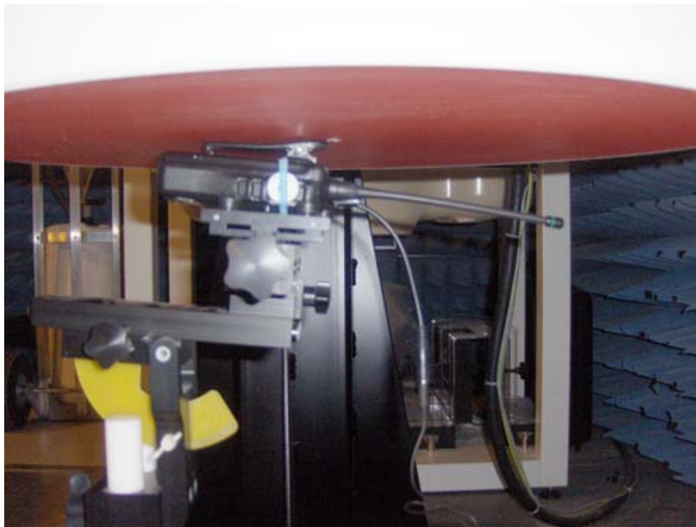
Back side of EUT in parallel to the phantom with the belt-clip (M/N: MB-124) in contact, attached 3 different- type Speaker-microphone separately
