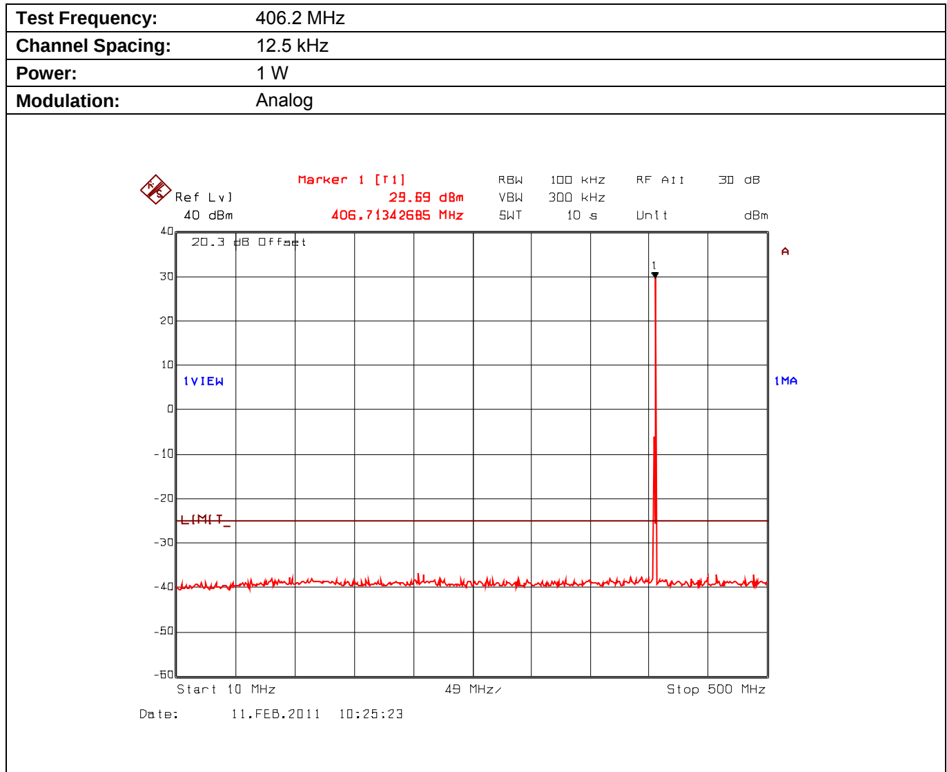
Plot 5.9.4.1.3. Conducted Transmitter Spurious Emissions for 406.2 MHz, Low Power, 10 MHz - 500 MHz
