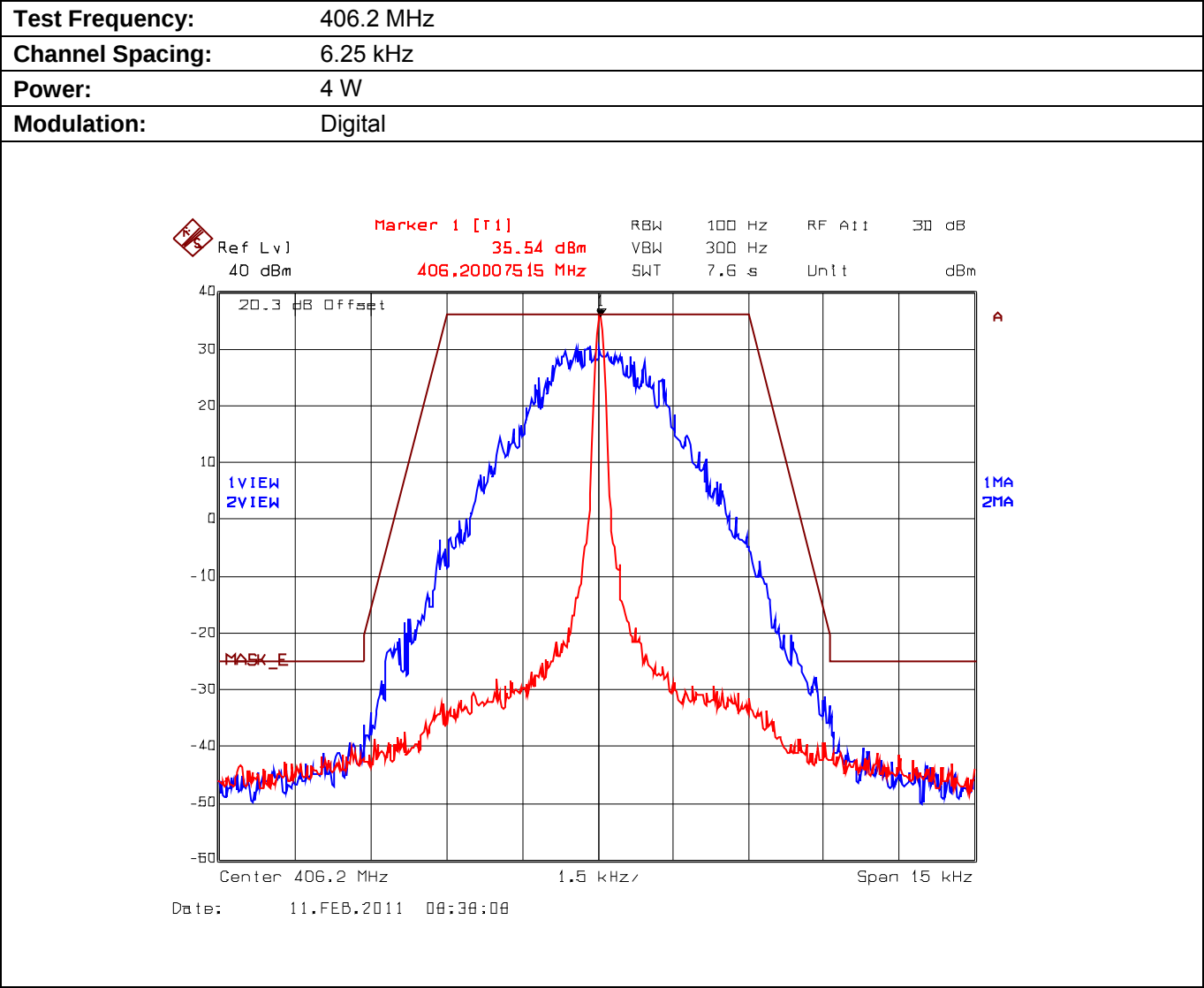
Plot 5.8.4.3.1. Emission Mask E, High Power
