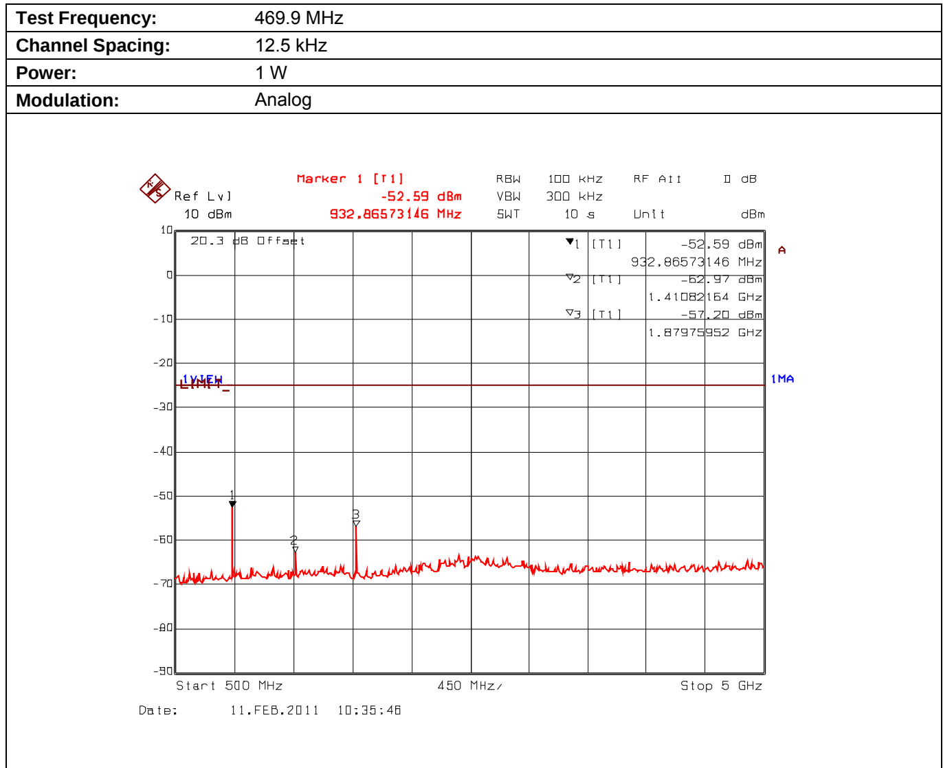
Plot 5.9.4.3.4. Conducted Transmitter Spurious Emissions for 469.9 MHz, Low Power, 500 MHz - 5 GHz
