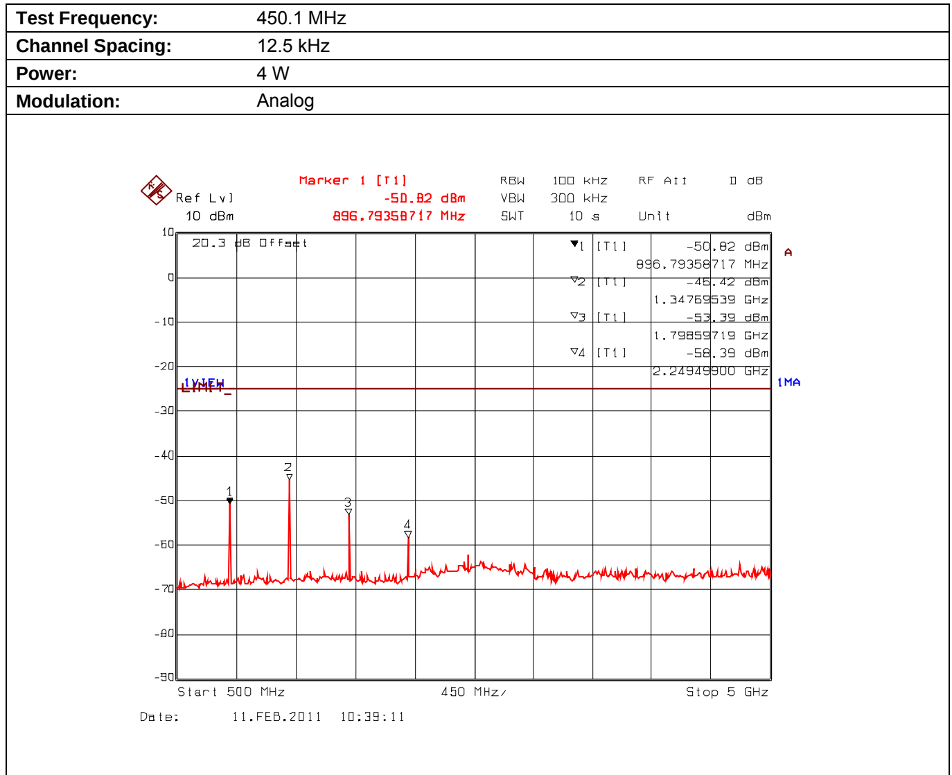
Plot 5.9.4.2.2. Conducted Transmitter Spurious Emissions for 450.1 MHz, High Power, 500 MHz - 5 GHz
