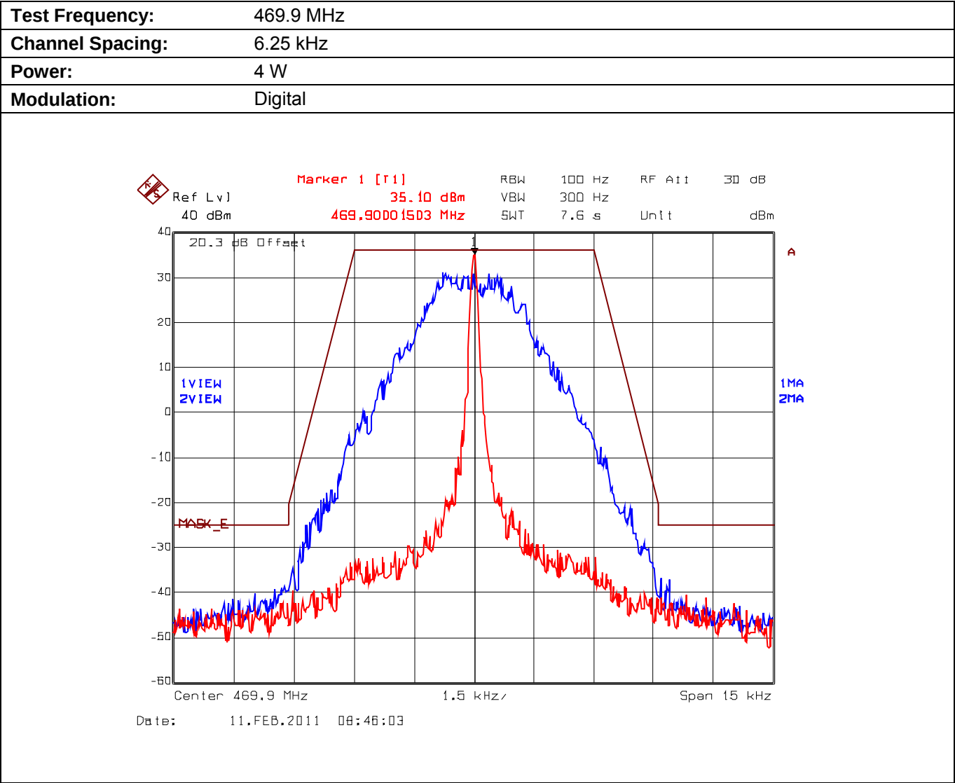
Plot 5.8.4.3.3. Emission Mask E, High Power
