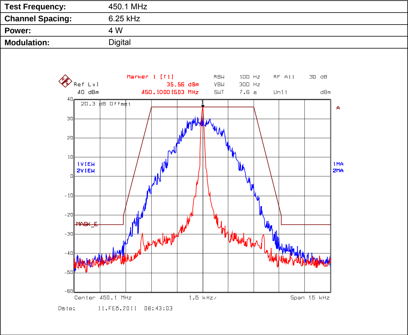
Plot 5.8.4.3.2. Emission Mask E, High Power
