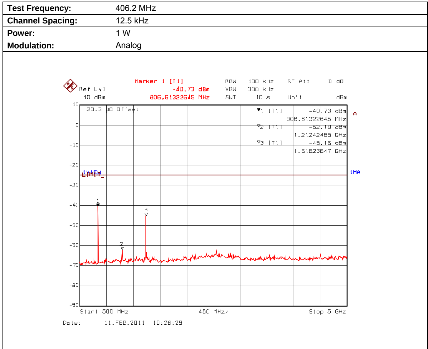
Plot 5.9.4.1.4. Conducted Transmitter Spurious Emissions for 406.2 MHz, Low Power, 500 MHz - 5 GHz
