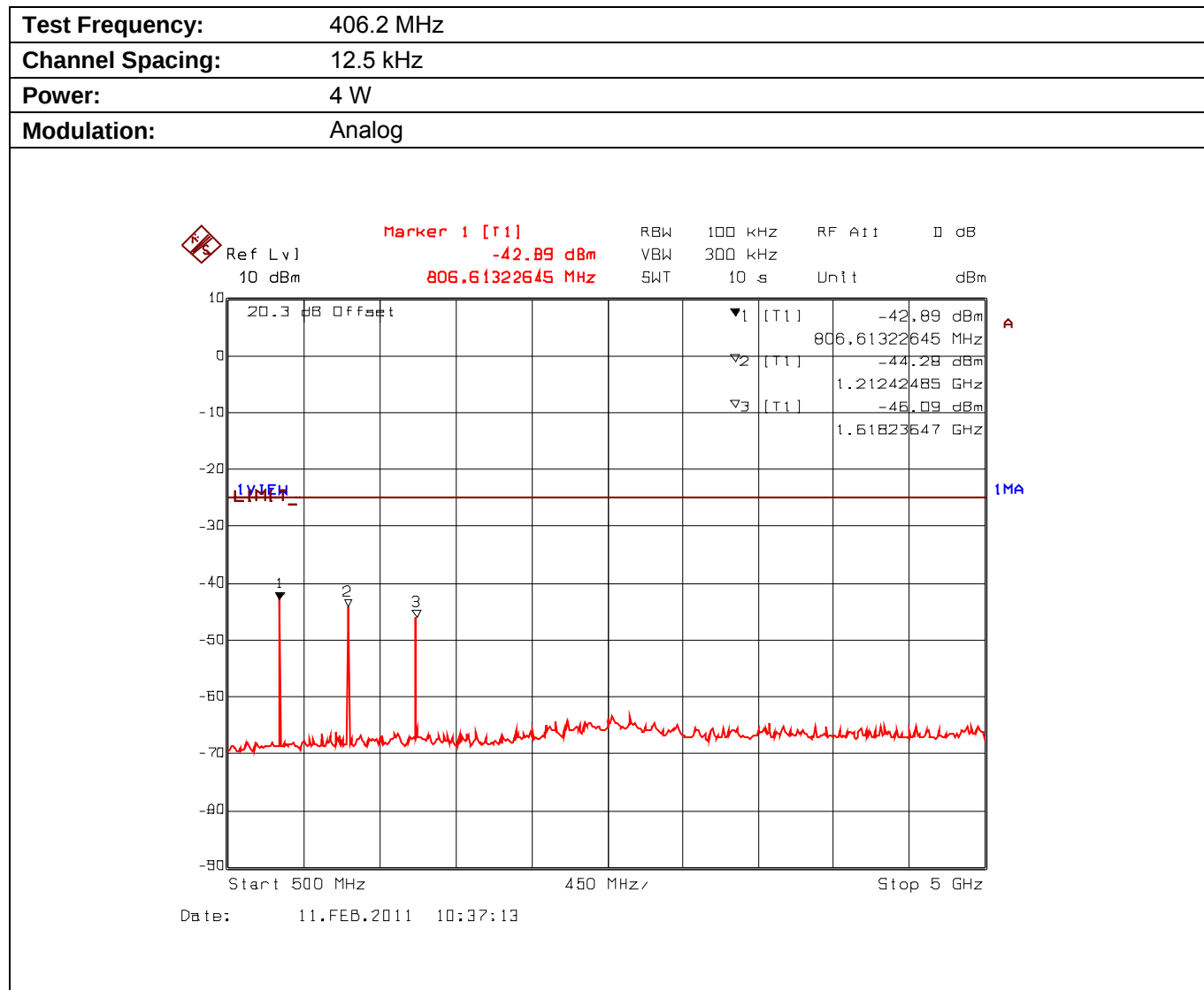
Plot 5.9.4.1.2. Conducted Transmitter Spurious Emissions for 406.2 MHz, High Power, 500 MHz - 5 GHz
