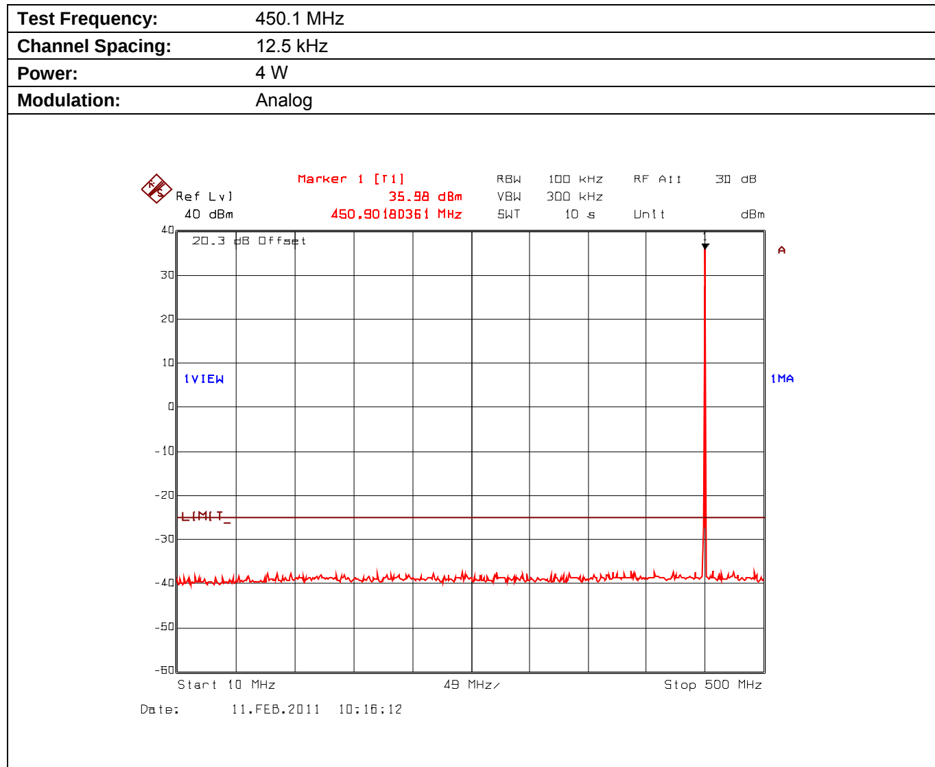
Plot 5.9.4.2.1. Conducted Transmitter Spurious Emissions for 450.1 MHz, High Power, 10 MHz - 500 MHz
