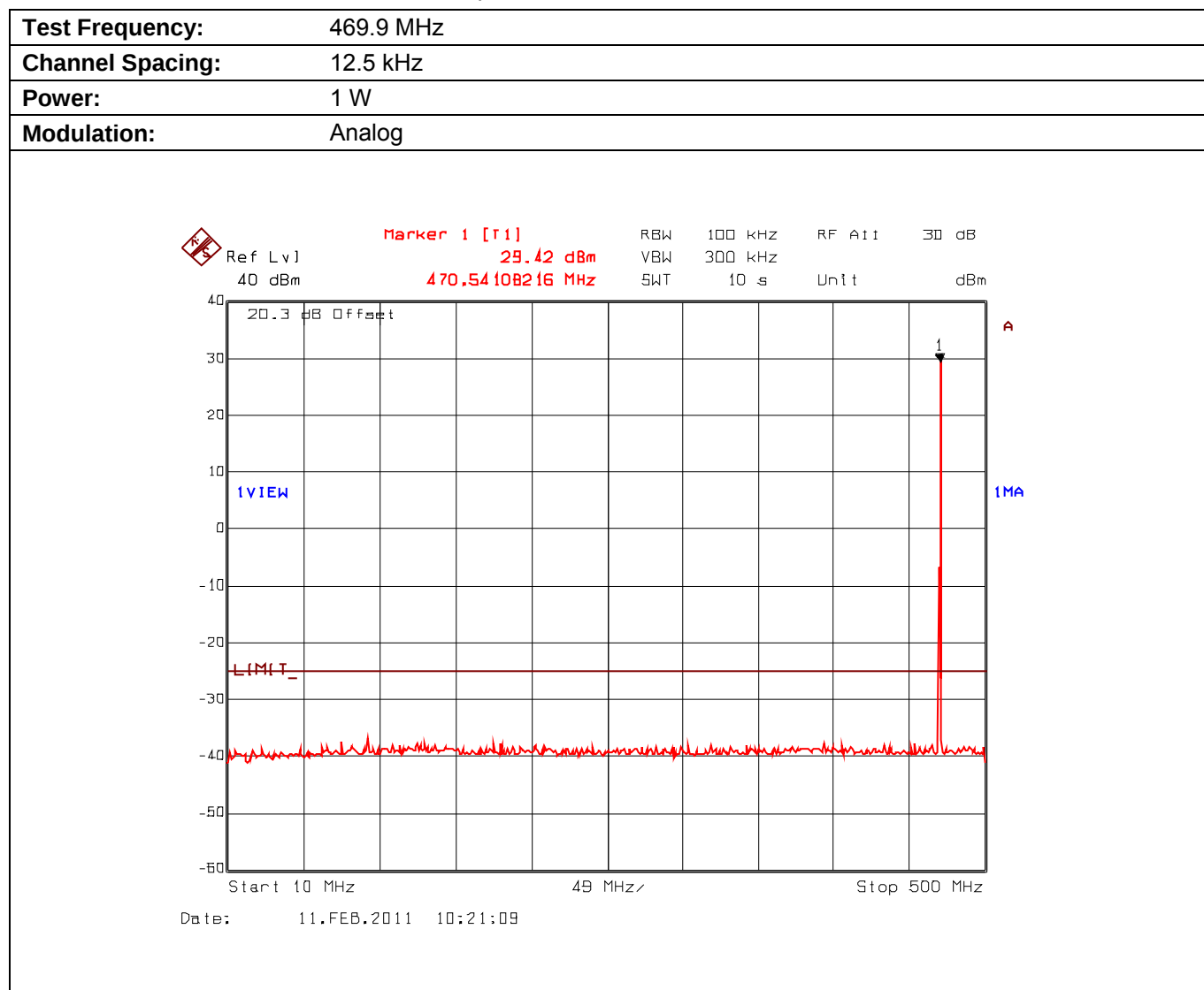
Plot 5.9.4.3.3. Conducted Transmitter Spurious Emissions for 469.9 MHz, Low Power, 10 MHz - 500 MHz
