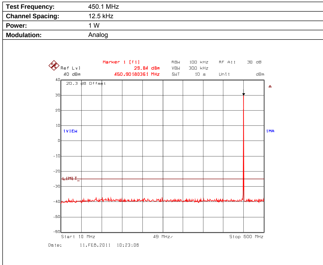
Plot 5.9.4.2.3. Conducted Transmitter Spurious Emissions for 450.1 MHz, Low Power, 10 MHz - 500 MHz
