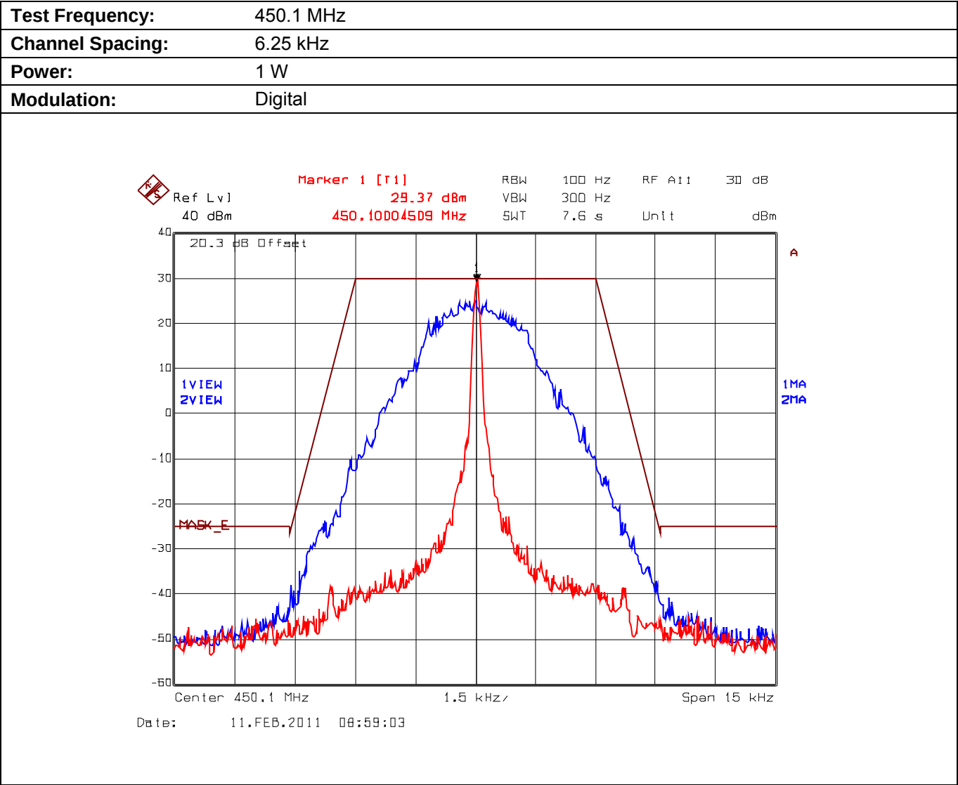
Plot 5.8.4.3.5. Emission Mask E, Low Power
