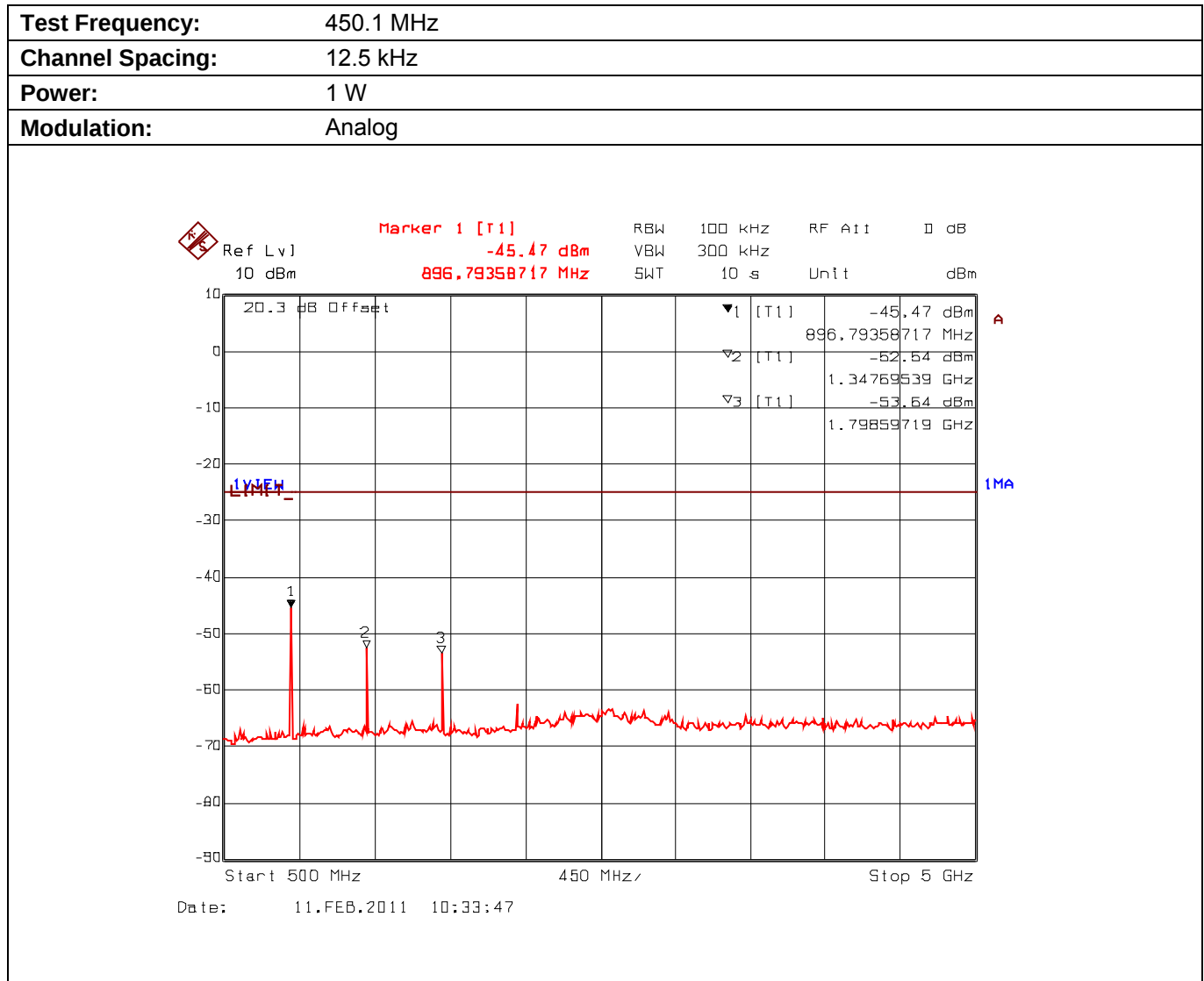
Plot 5.9.4.2.4. Conducted Transmitter Spurious Emissions for 450.1 MHz, Low Power, 500 MHz – 5 GHz
