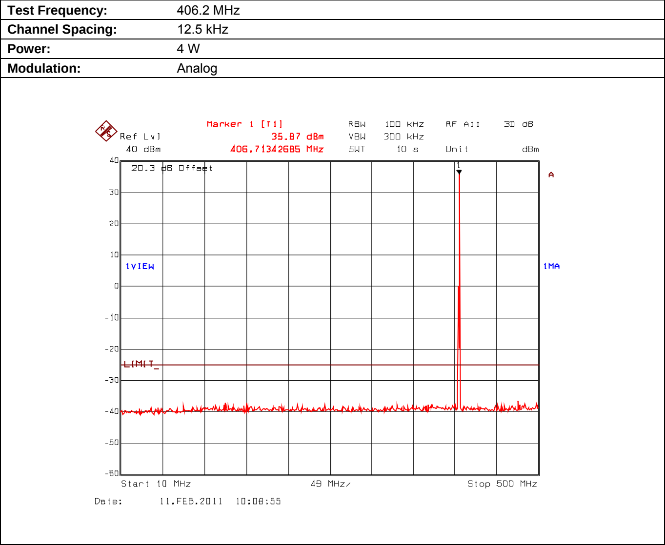
Plot 5.9.4.1.1. Conducted Transmitter Spurious Emissions for 406.2 MHz, High Power, 10 MHz - 500 MHz
