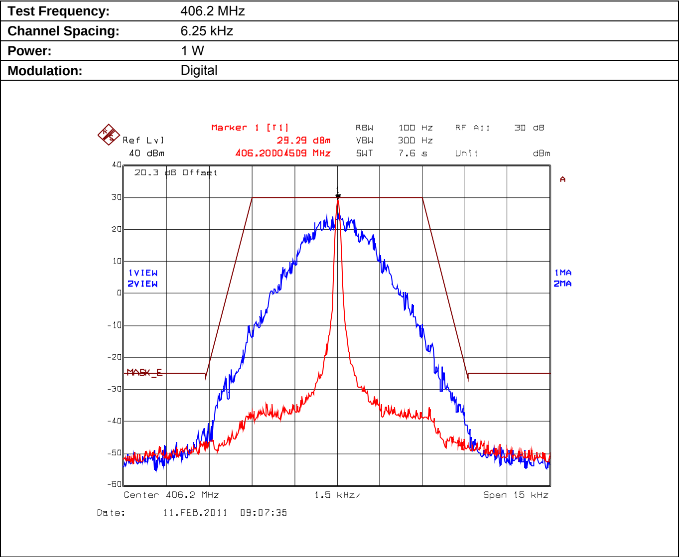
Plot 5.8.4.3.4. Emission Mask E, Low Power
