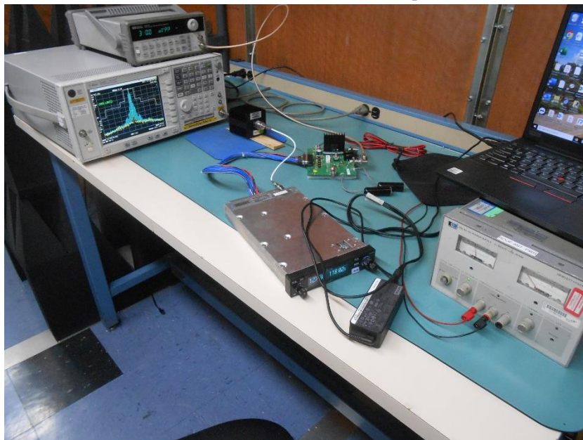
Conducted Test Bench Setup 2
