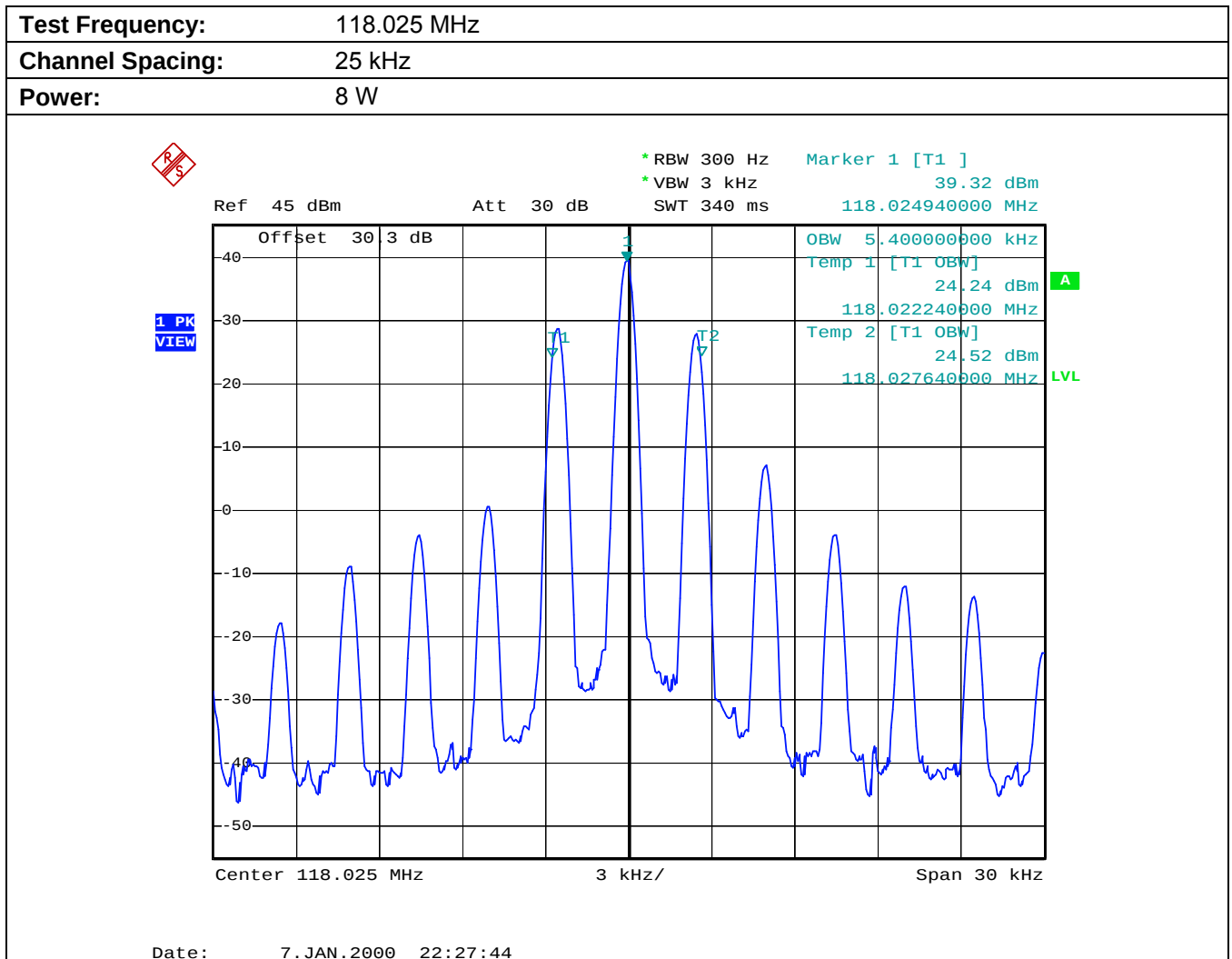
Plot 5.6.4.1.4. 99% Occupied Bandwidth
