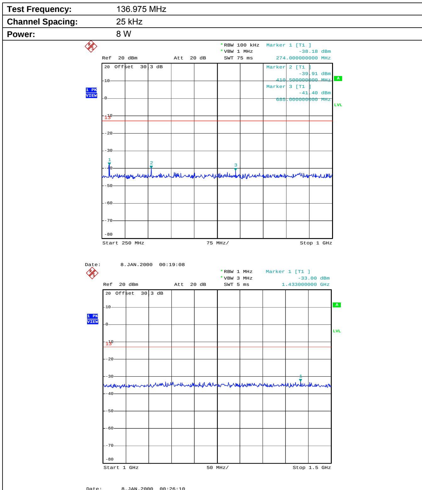
Plot 5.10.4.6. Conducted Transmitter Spurious Emissions 250 MHz – 1.5 GHz
