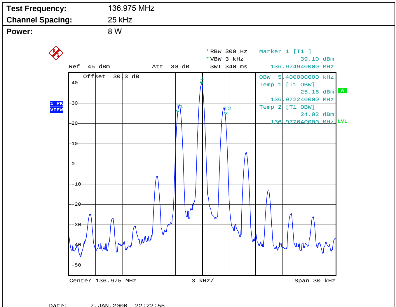
Plot 5.6.4.1.6. 99% Occupied Bandwidth
