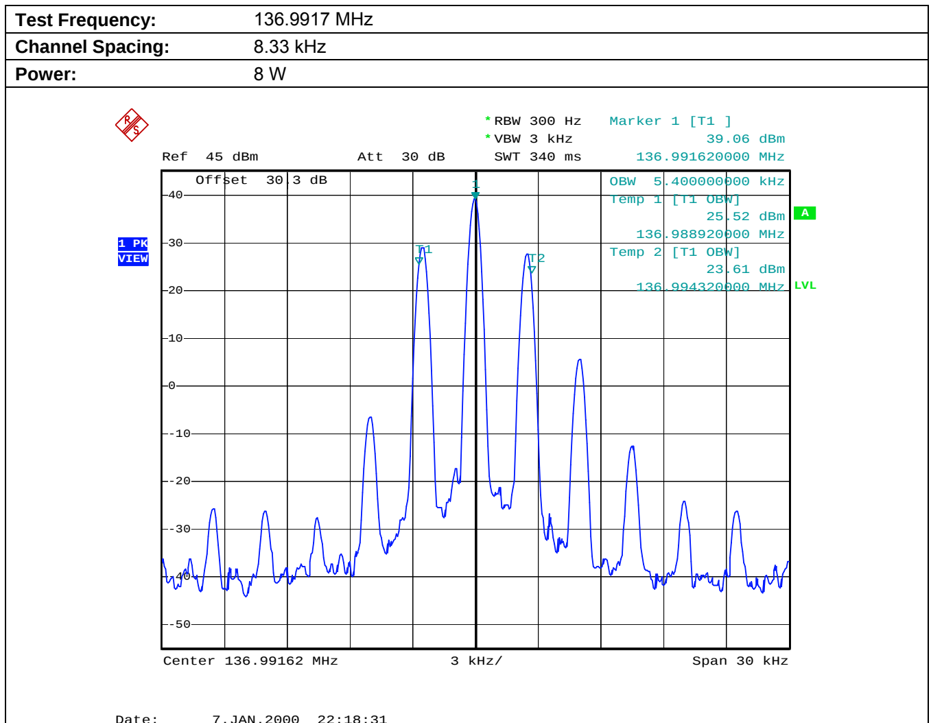
Plot 5.6.4.1.3. 99% Occupied Bandwidth
