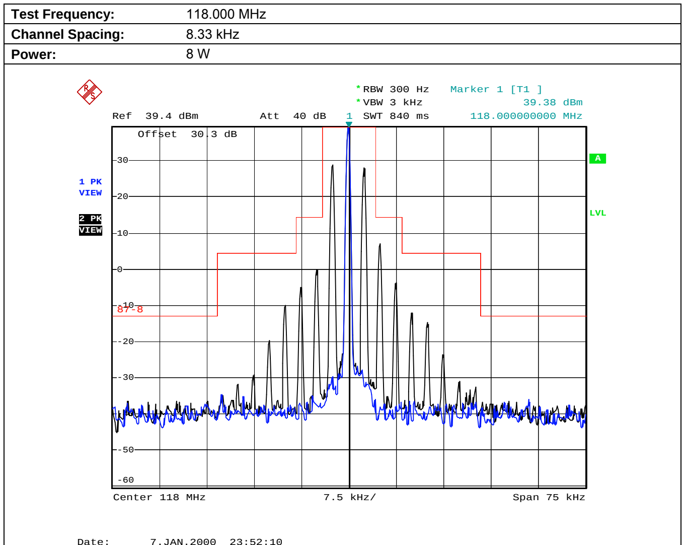
Plot 5.6.4.2.1. Emissions Limitation
