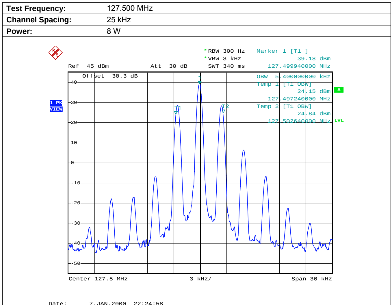
Plot 5.6.4.1.5. 99% Occupied Bandwidth
