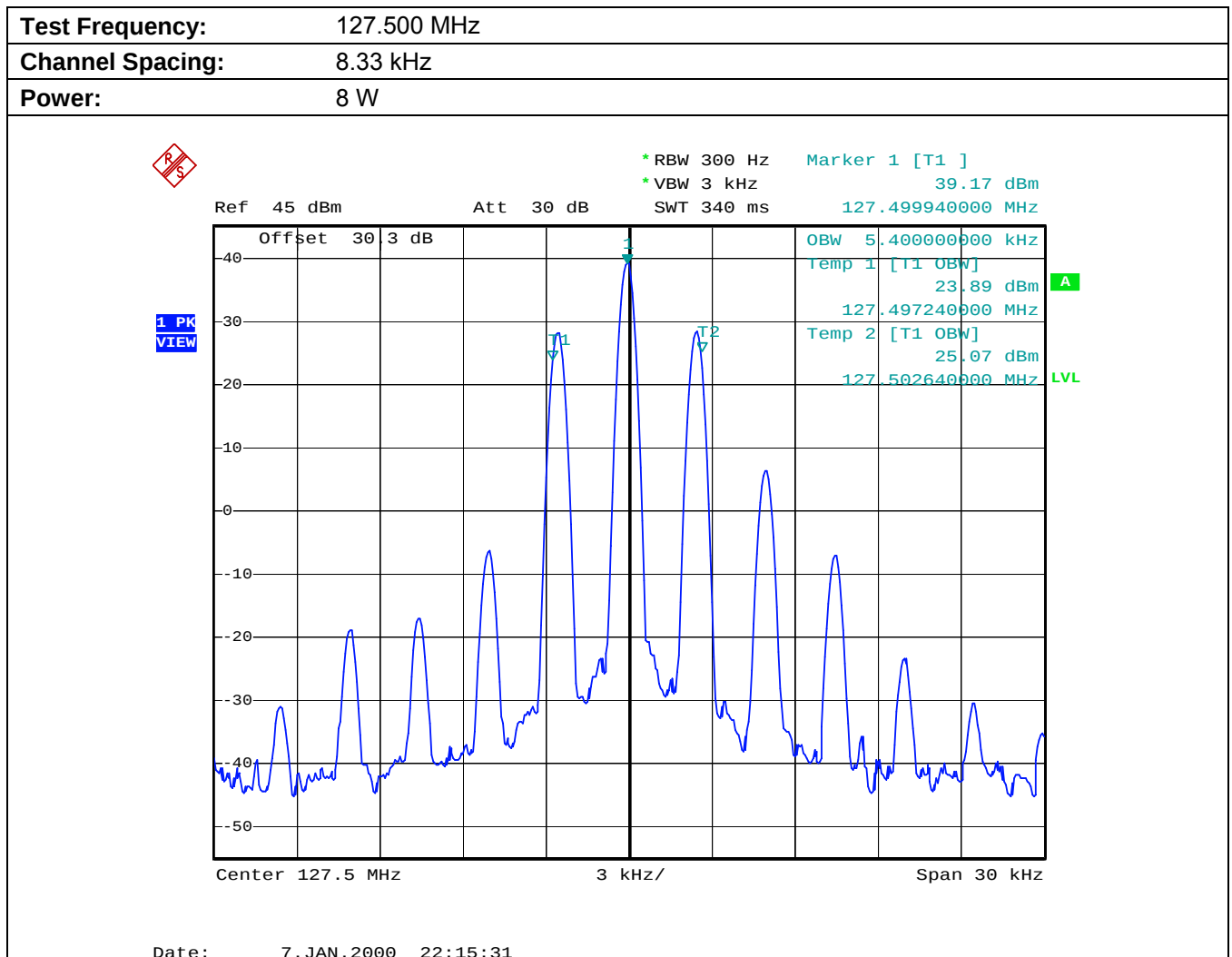
Plot 5.6.4.1.2. 99% Occupied Bandwidth
