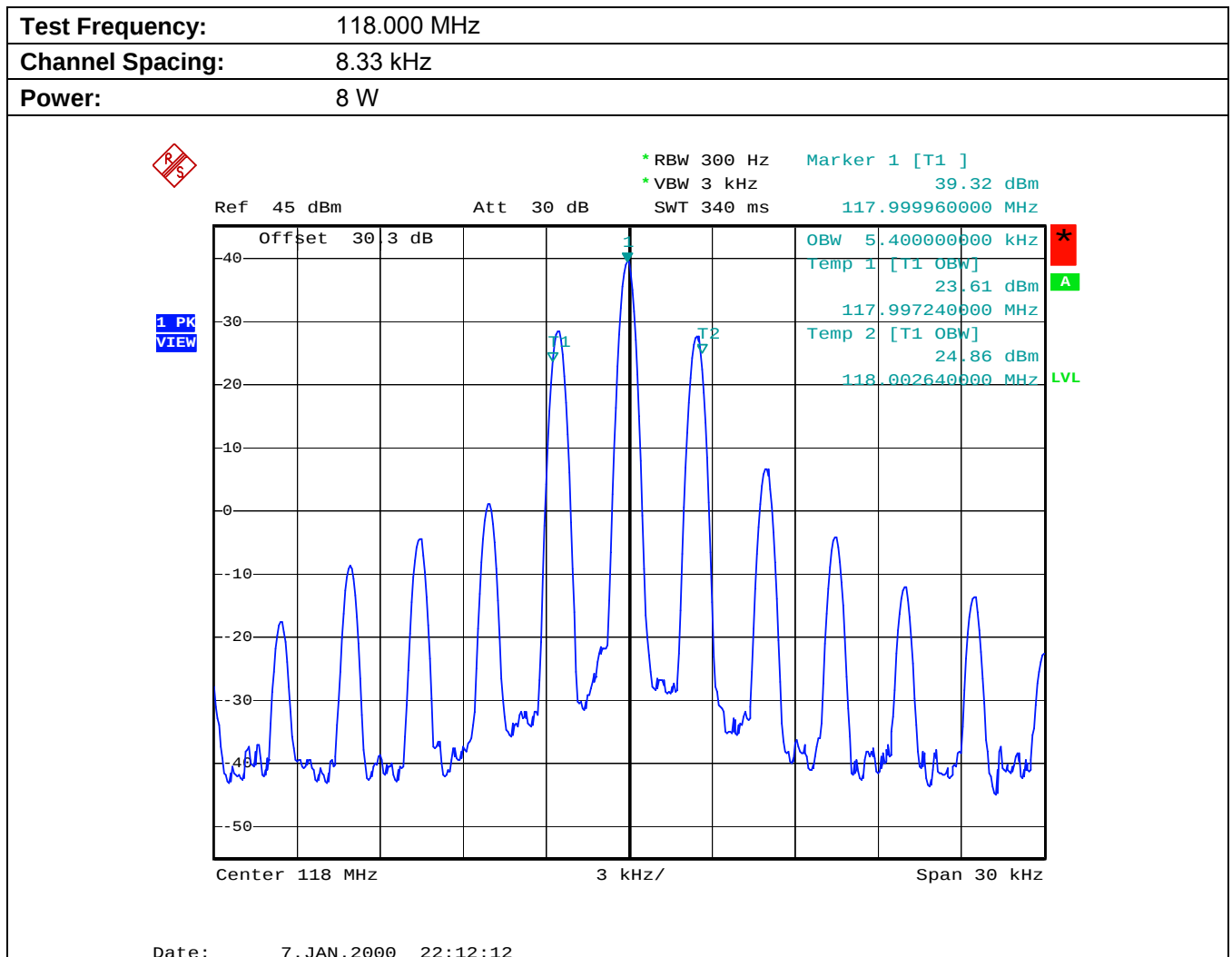
Plot 5.6.4.1.1. 99% Occupied Bandwidth
