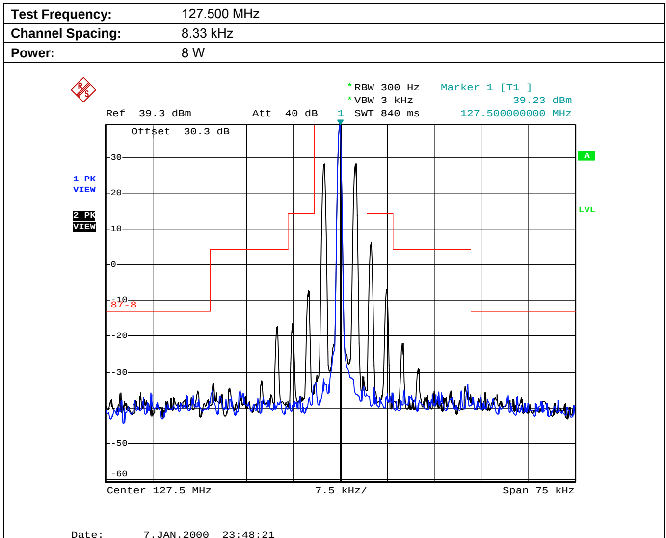
Plot 5.6.4.2.2. Emissions Limitation
