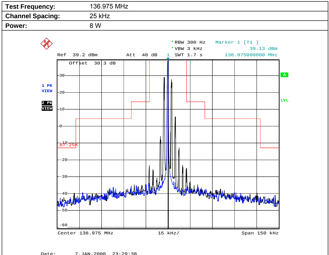
Plot 5.6.4.2.6. Emissions Limitation
