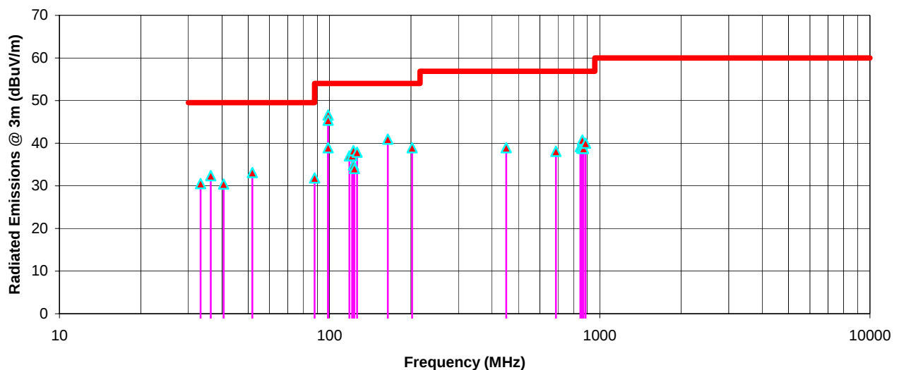
Radiated Emissions Measurements @ 3m OFTS
