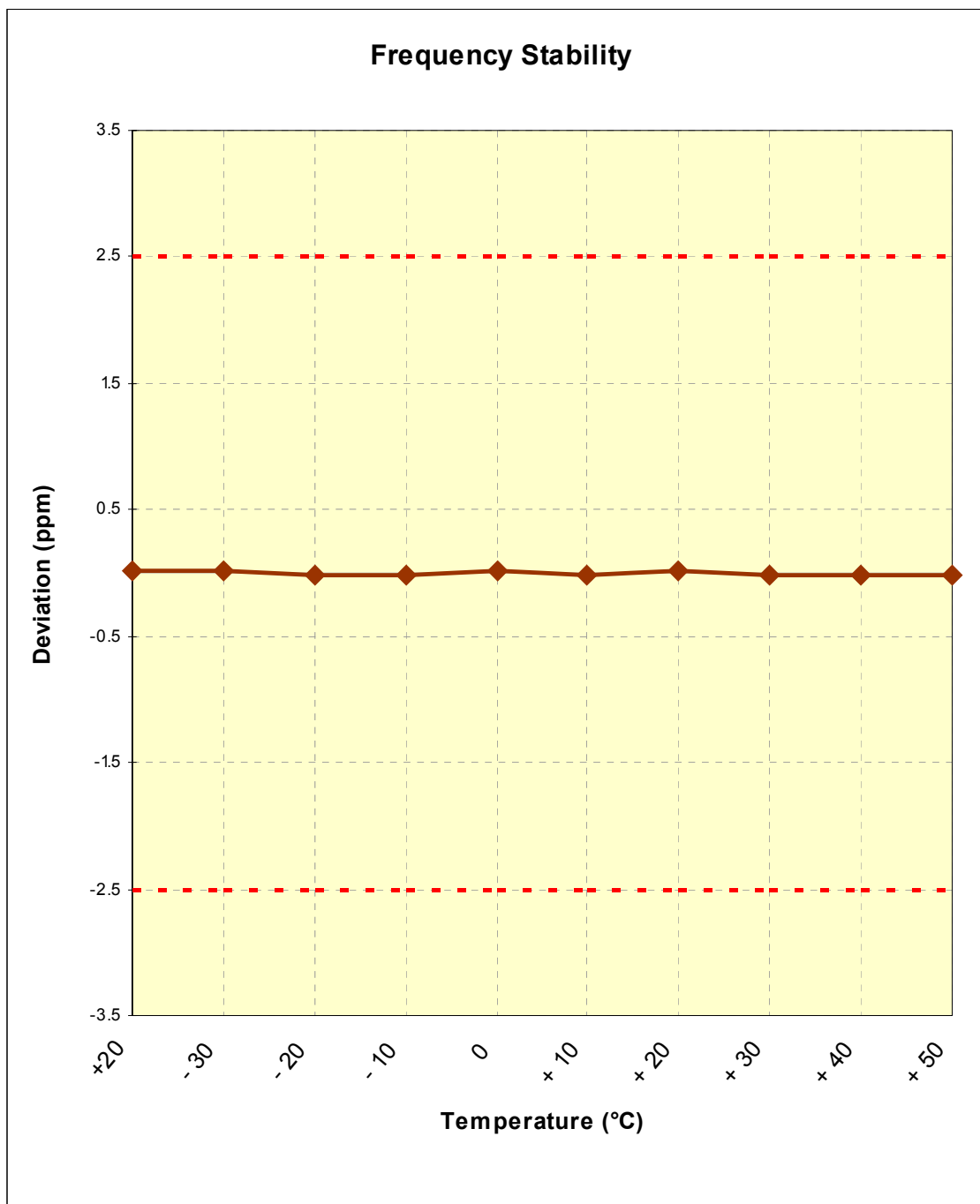
Figure 6-1. Frequency Stability Graph (Cellular CDMA Mode – Ch.383)
