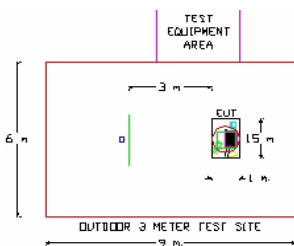
Figure 3-2. Dimensions of Outdoor Test Site
