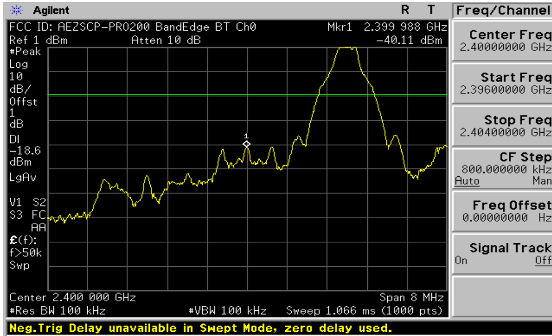
Plot 6-4. Band Edge Plot (Bluetooth – Ch. 0)
