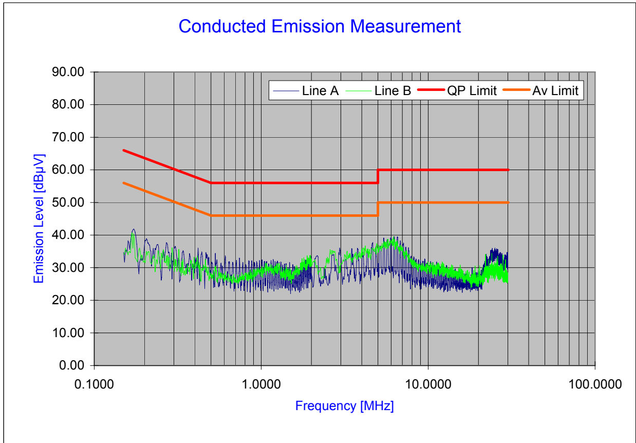
Plot 6-1. Line Conducted Plot with Bluetooth
