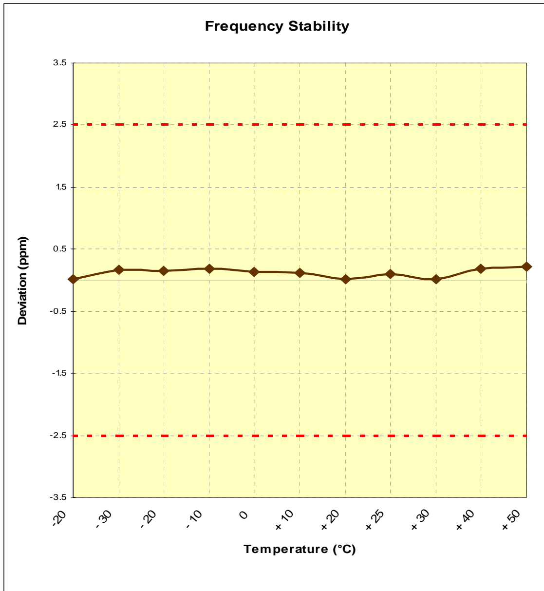
Figure 6-1. Frequency Stability Graph (Cellular CDMA Mode – Ch. 383)
