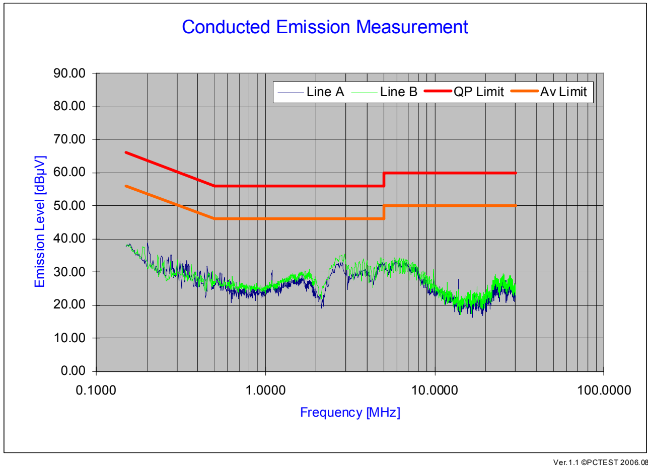
Plot 6-16. Line Conducted Plot with Bluetooth
