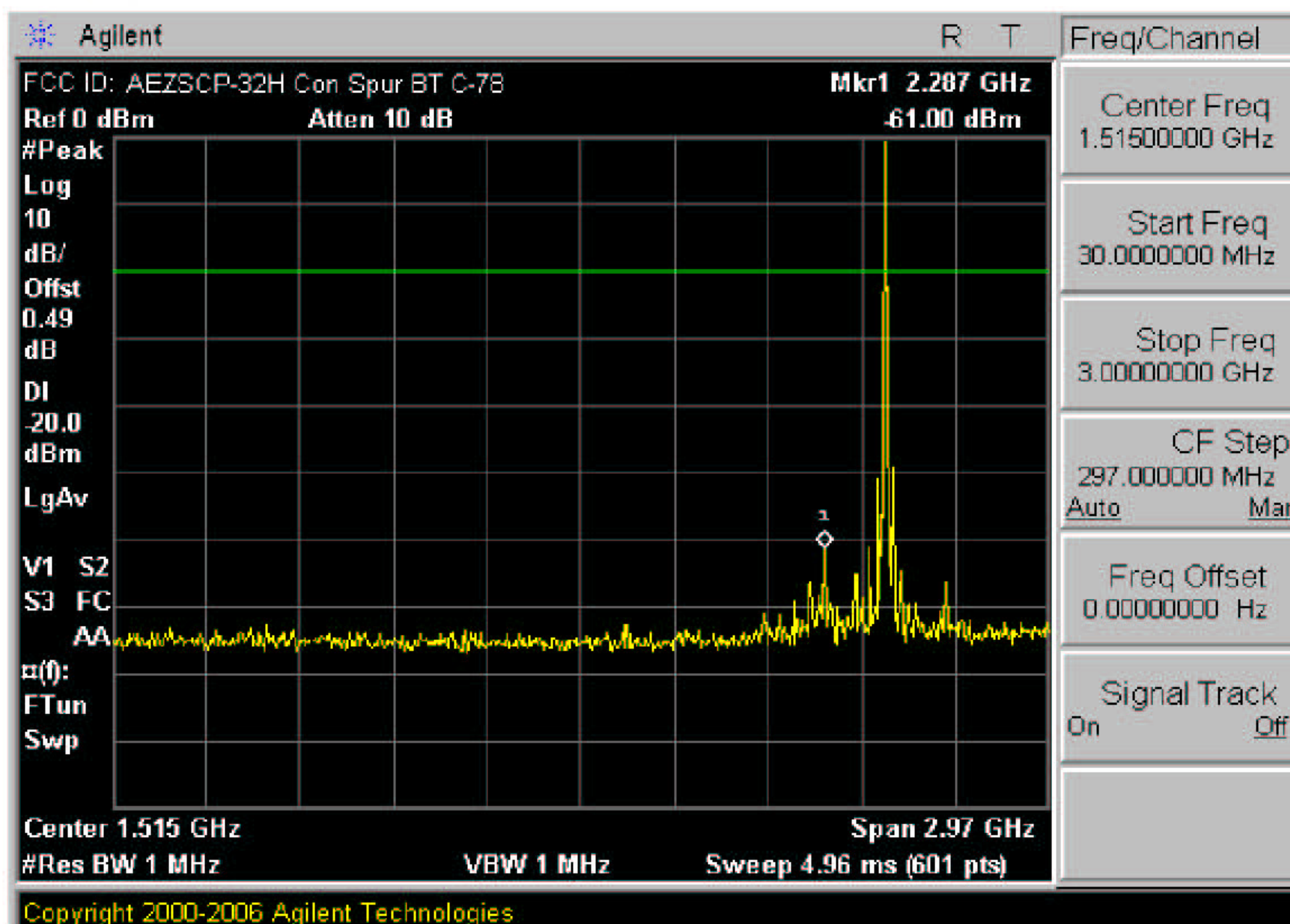
Plot 6-14. Conducted Spurious Plot (Bluetooth – Ch. 78)
