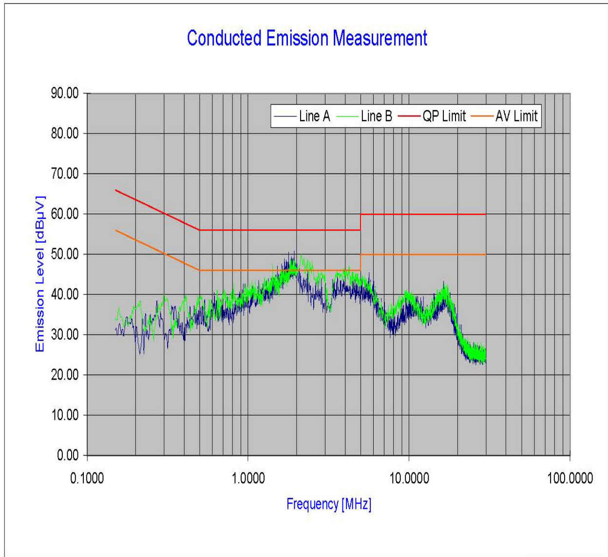
Plot 6-16. Line Conducted Plot with Bluetooth
