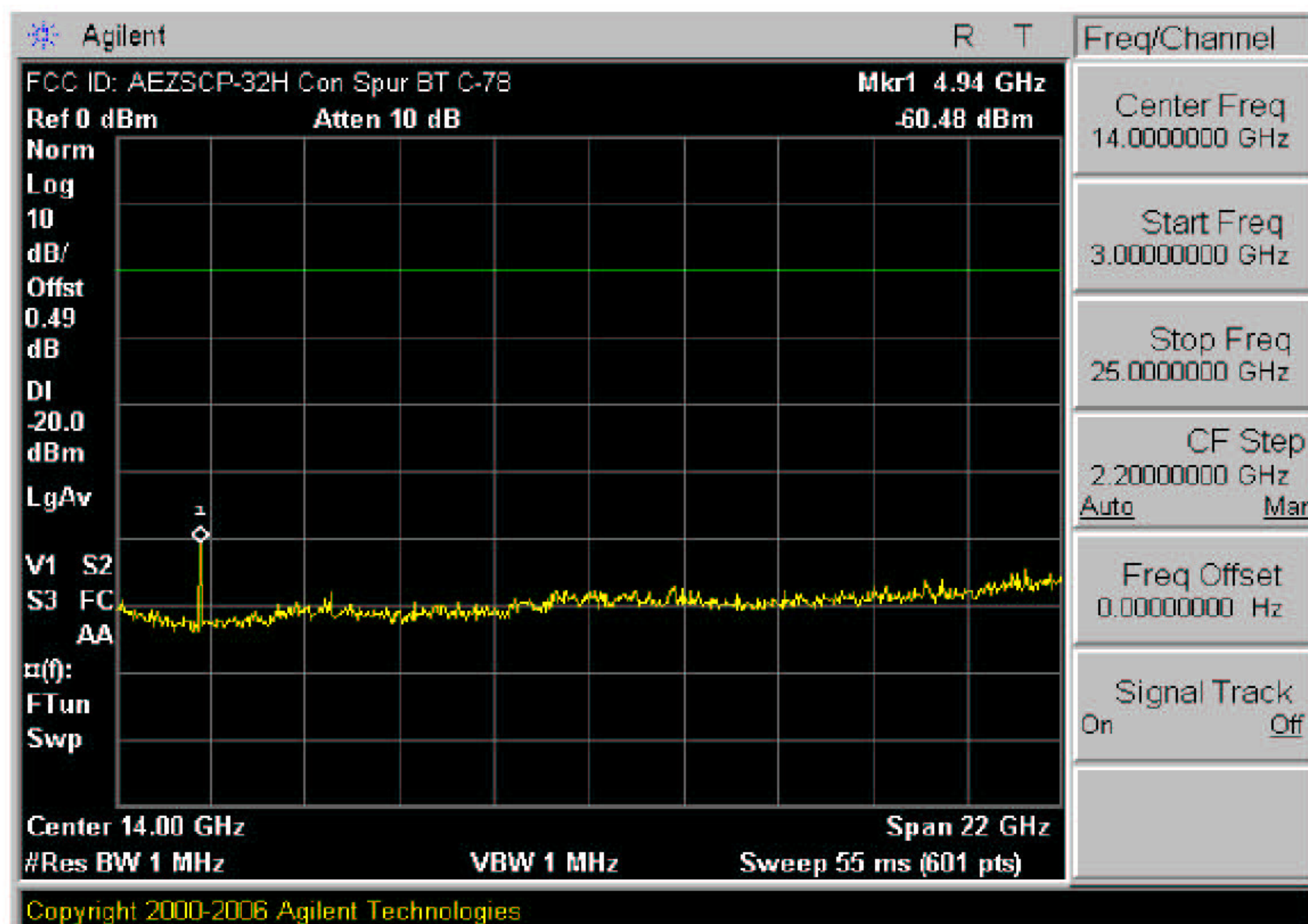
Plot 6-15. Conducted Spurious Plot (Bluetooth – Ch. 78)
