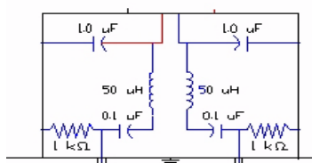
Figure 3.1-4. LISN Schematic Diagram
