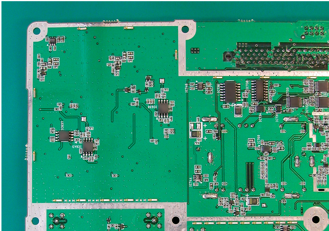
23-1 *RFMB board –back view (Part 1)
