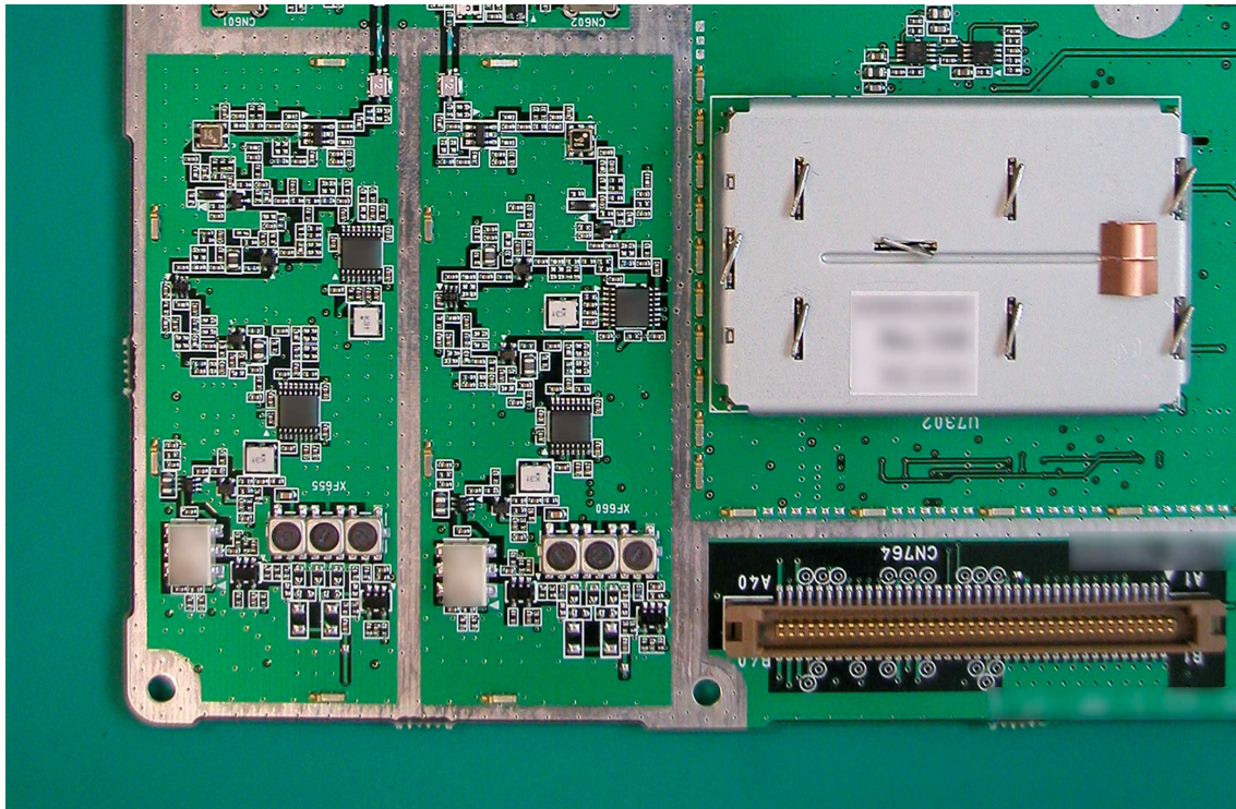
21-2 *RFMB board –front view (Part 2)
