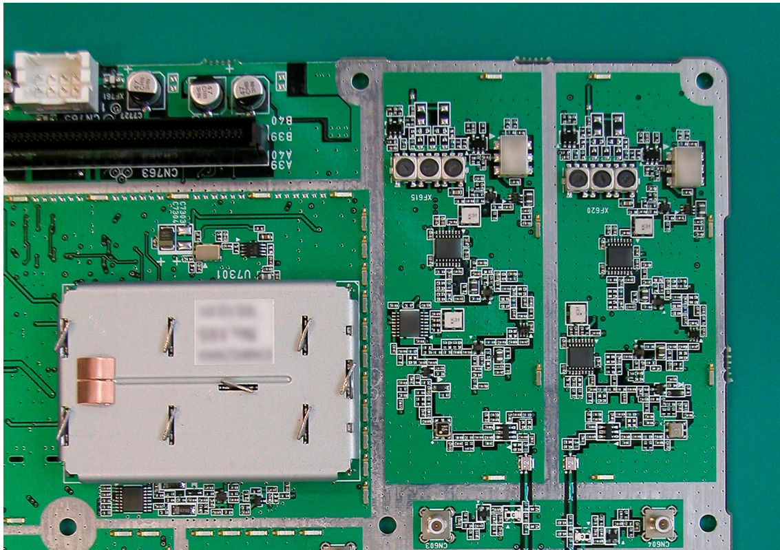
21-3 *RFMB board –front view (Part 3)
