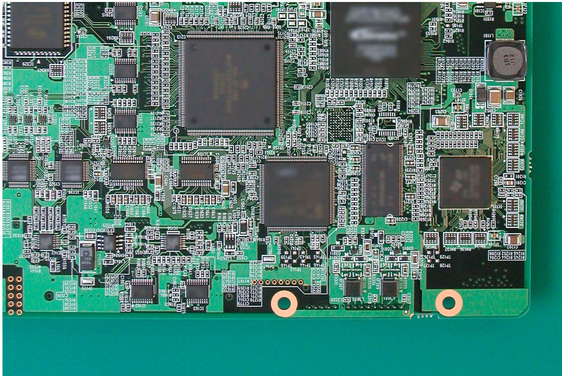
18-4 *Control board –back view (Part 4)
