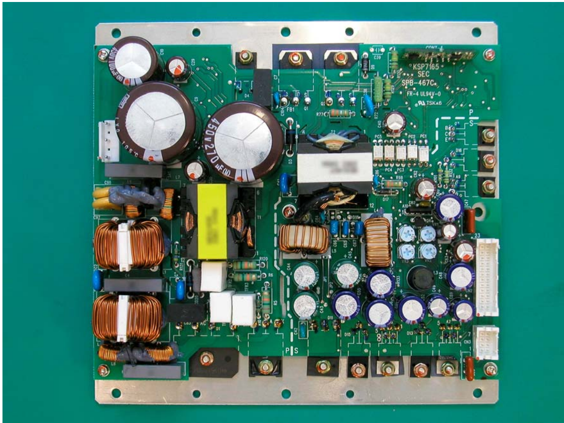
12 Power module (SENDAN, without cover)
