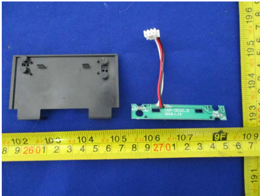
EUT – Charger Base Uncover 3 View
