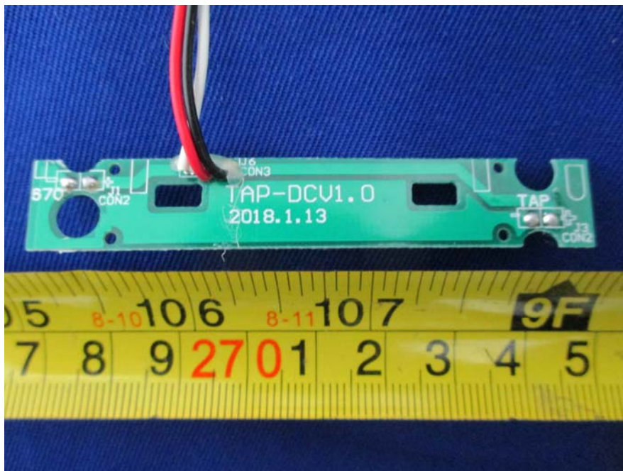
EUT – Charger Base PCB-3 Top View
