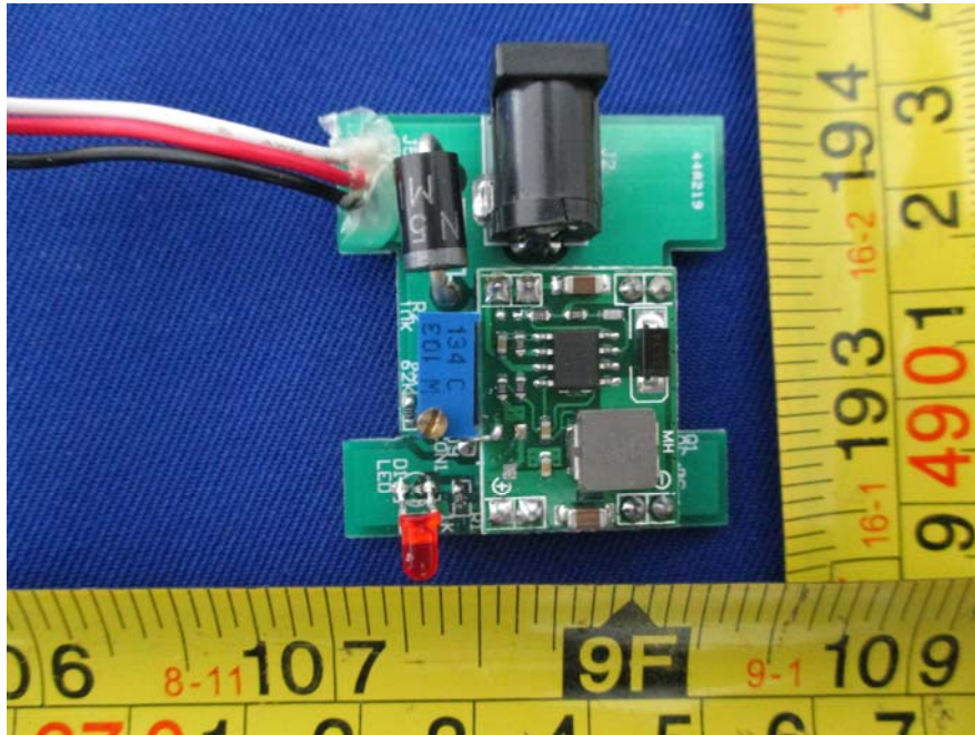
EUT – Charger Base PCB-2 Top View
