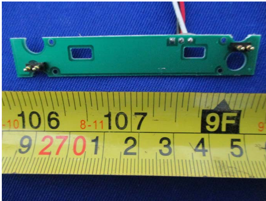
EUT – Charger Base PCB-3 Bottom View
