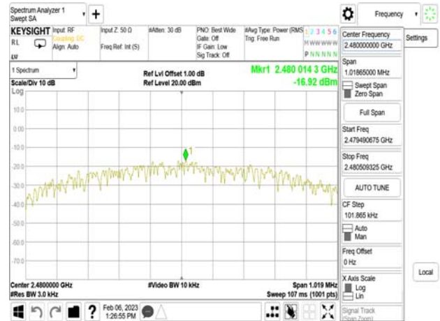
PSD_BLE 1M_HighCH39-2480MHz
