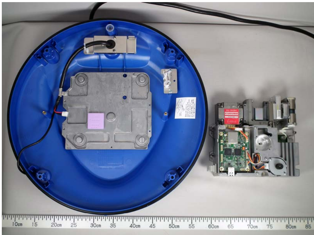
1.5 Top View (with Transceiver module removed)
