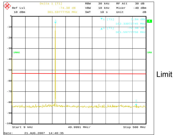
Graph 3.3b – Spurious Emissions at Antenna terminal on Channel 1088 with 2 W TX mode
