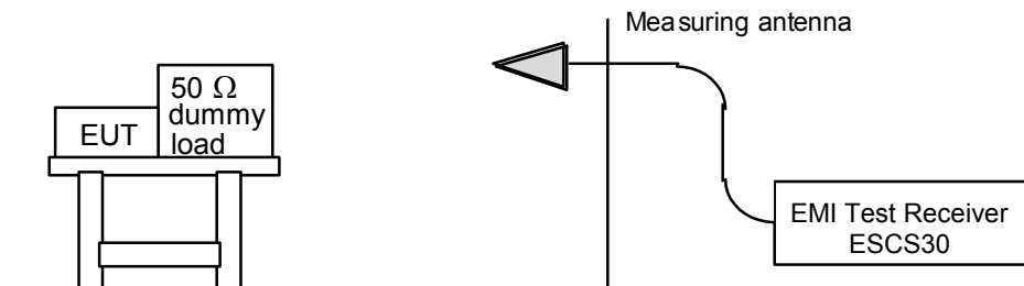
Fig 3.4A Setup for measurement of fundamental component
