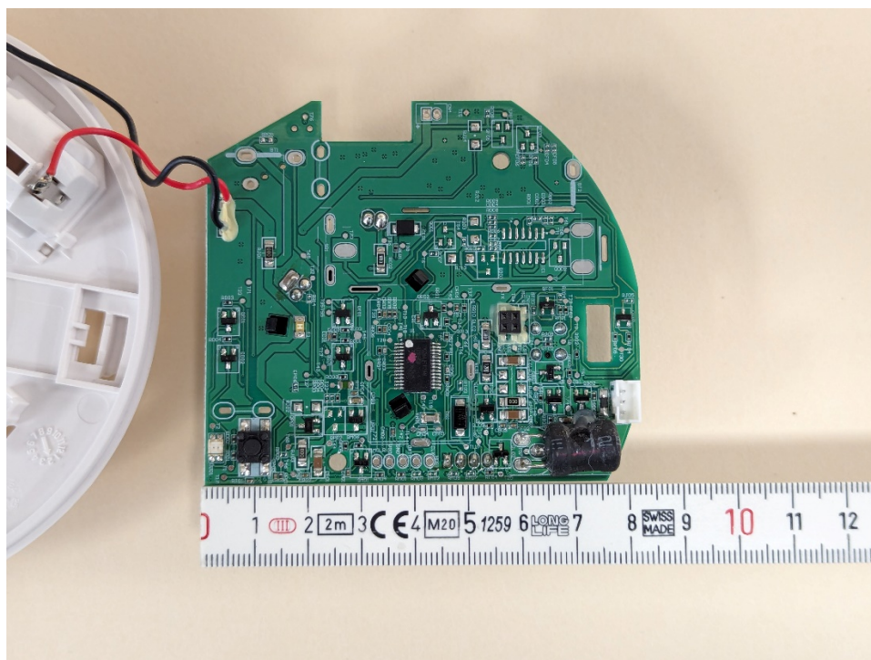
Bottom of Main PCB
