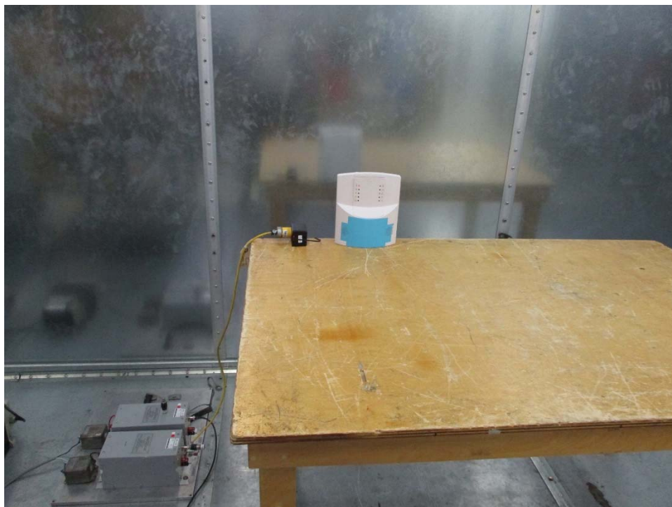
Conducted Emissions, Power Leads, Front Configuration
