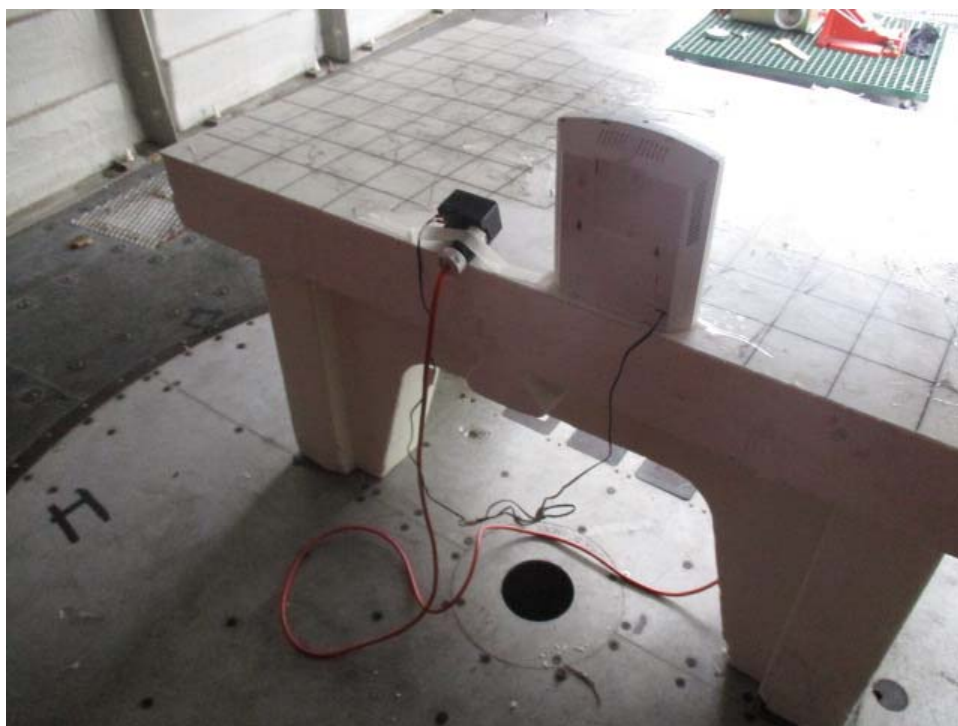
Spurious Radiated Emissions, EUT Configuration, Rear View
