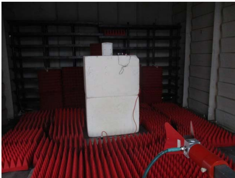
Spurious Radiated Emissions, Horizontal Polarization, 1 GHz to 10 GHz
