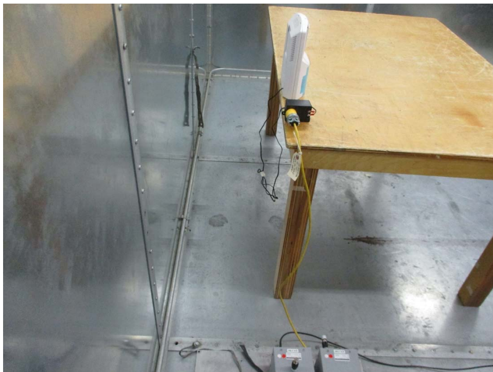
Conducted Emissions, Power Leads, Rear Configuration
