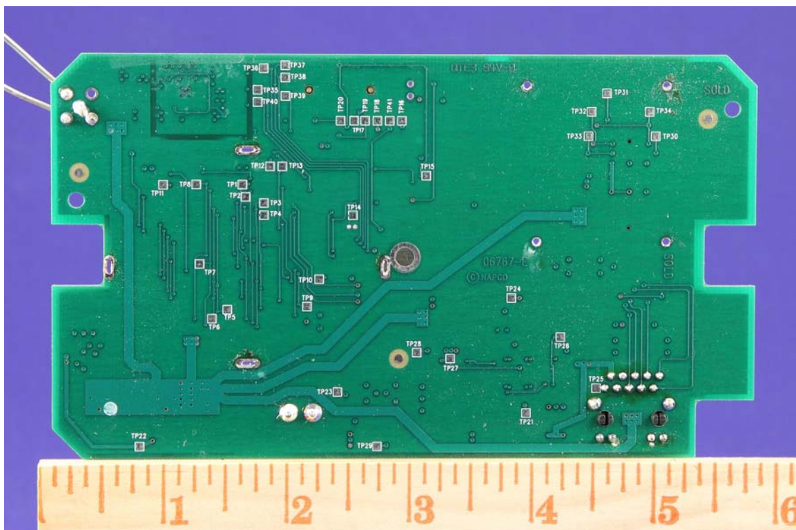
Solder Side:
