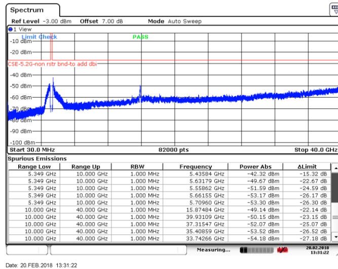
Figure 8.4-14: Spurious emissions outside restricted bands, Tx on ch 58, 802.11ac VHT80
