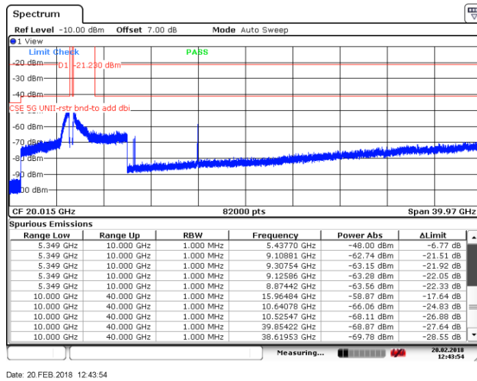
Figure 8.4-29: Spurious emissions within restricted bands, Tx on ch 64, 802.11a
