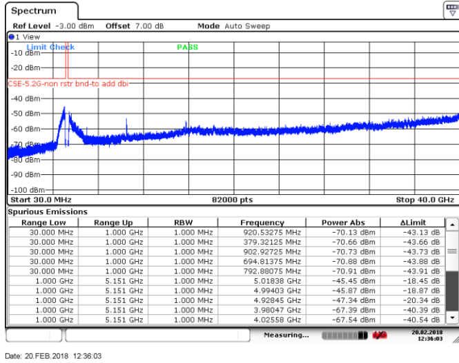
Figure 8.4-1: Spurious emissions outside restricted bands, Tx on ch 52, 802.11a
