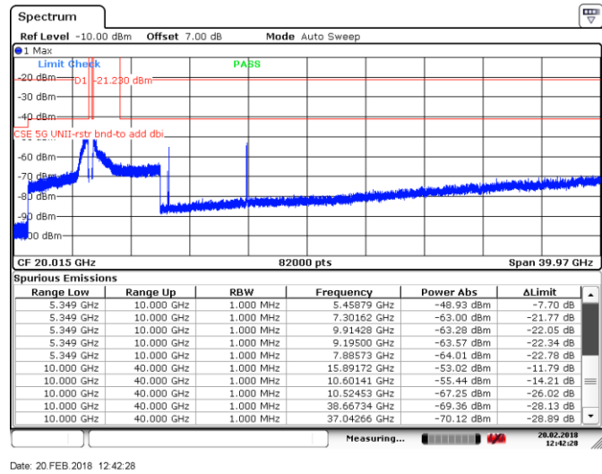
Figure 8.4-28: Spurious emissions within restricted bands, Tx on ch 60, 802.11a
