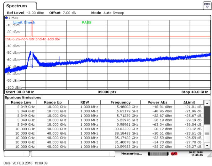
Figure 8.4-10: Spurious emissions outside restricted bands, Tx on ch 60, 802.11ac VHT20
