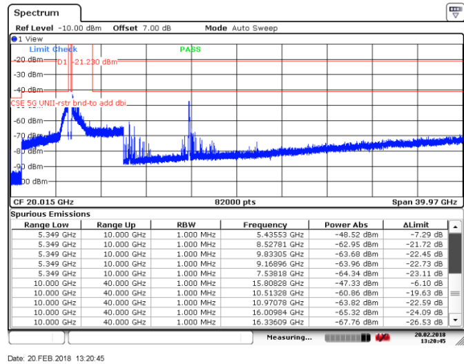
Figure 8.4-34: Peak Spurious emissions within restricted bands, Tx on ch 62, 802.11n HT40, Peak detector
