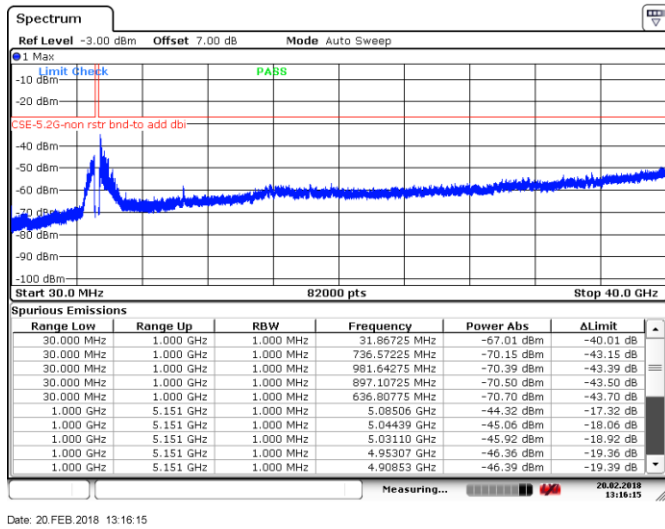
Figure 8.4-12: Spurious emissions outside restricted bands, Tx on ch 54, 802.11ac VHT40
