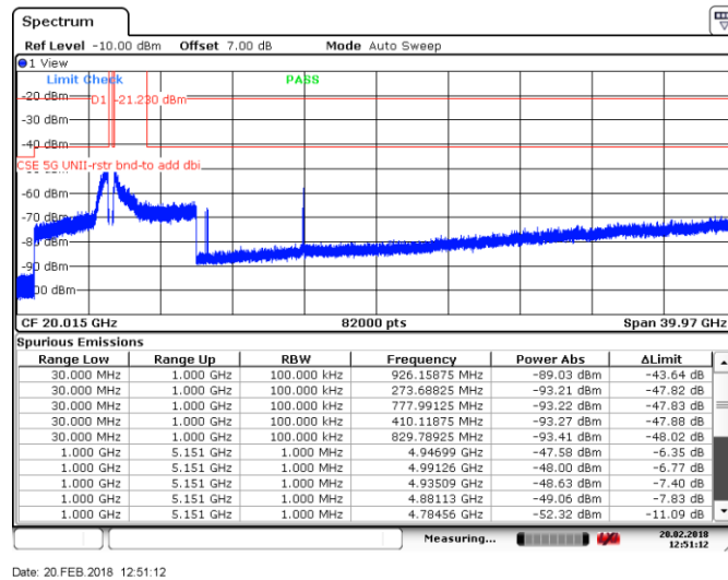
Figure 8.4-32: Spurious emissions within restricted bands, Tx on ch 64, 802.11n HT20
