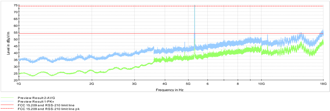
Figure 8.4-44: Cabinet Radiated spurious emission 1 to 18 GHz sample plot
