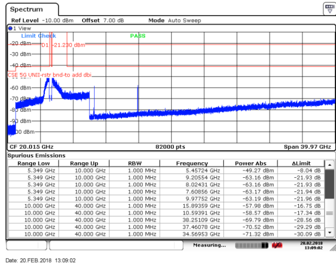
Figure 8.4-37: Spurious emissions within restricted bands, Tx on ch 60, 802.11ac VHT20
