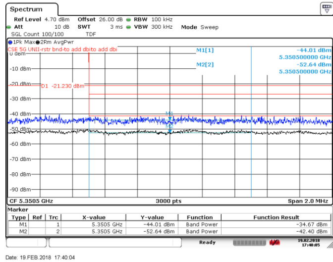
Figure 8.4-20: Upper band edge, Tx on ch 62, 802.11n HT40
