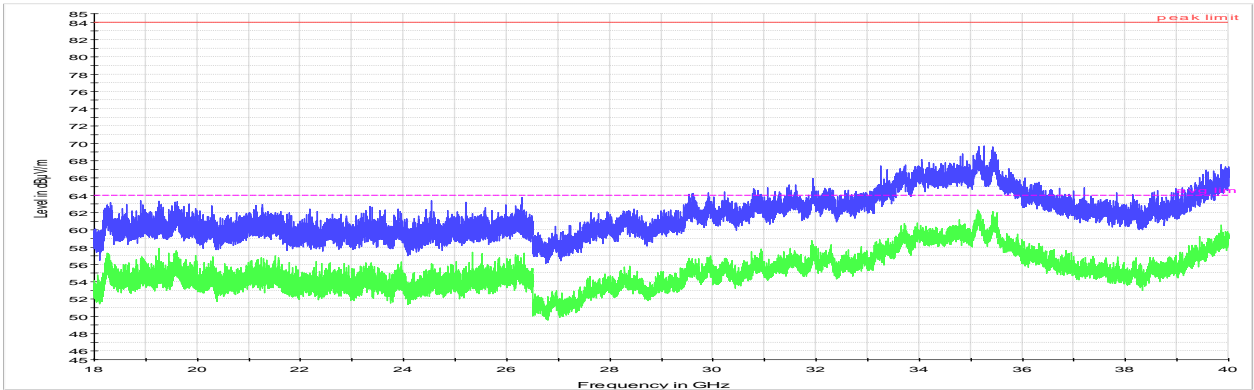
Figure 8.4-45: Cabinet Radiated spurious emission 18 to 40 GHz sample plot
