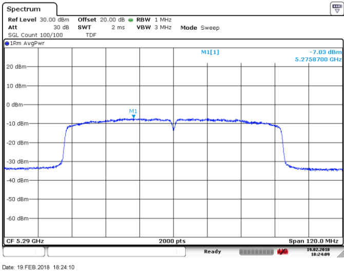
Figure 8.3-3: PSD on 802.11ac HT80, Sample plot
