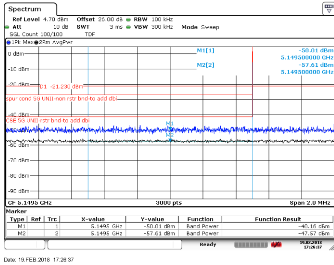
Figure 8.4-23: Lower band edge, Tx on ch 54, 802.11ac VHT40
