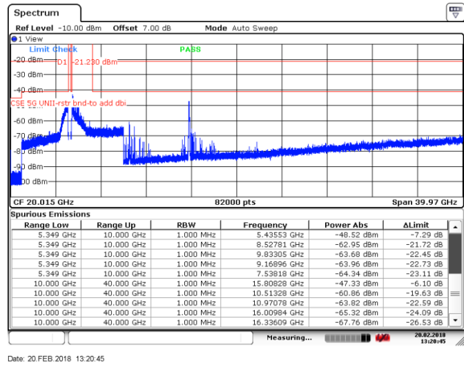
Figure 8.4-40: Spurious emissions within restricted bands, Tx on ch 62, 802.11ac VHT40
