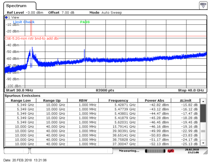
Figure 8.4-13: Spurious emissions outside restricted bands, Tx on ch 62, 802.11ac VHT40
