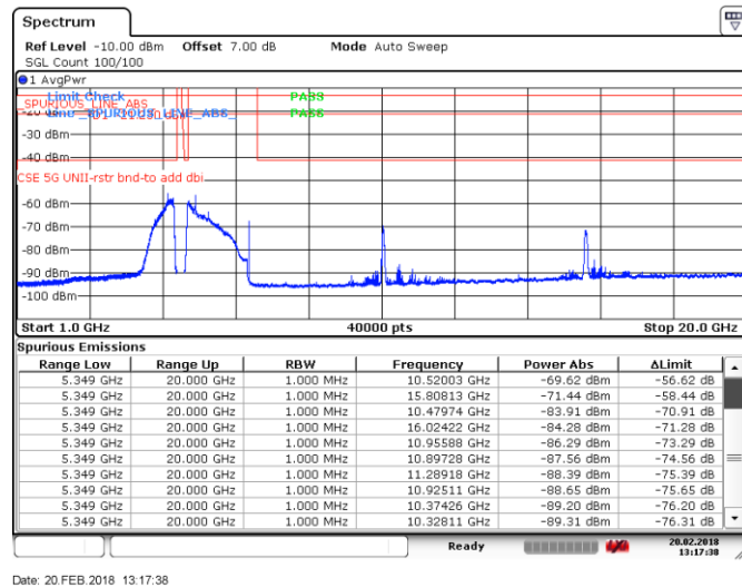
Figure 8.4-41: Spurious emissions within restricted bands, Tx on ch 54, 802.11ac VHT40, RMS detector
