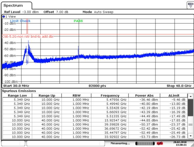
Figure 8.4-8: Spurious emissions outside restricted bands, Tx on ch 62, 802.11n HT40
