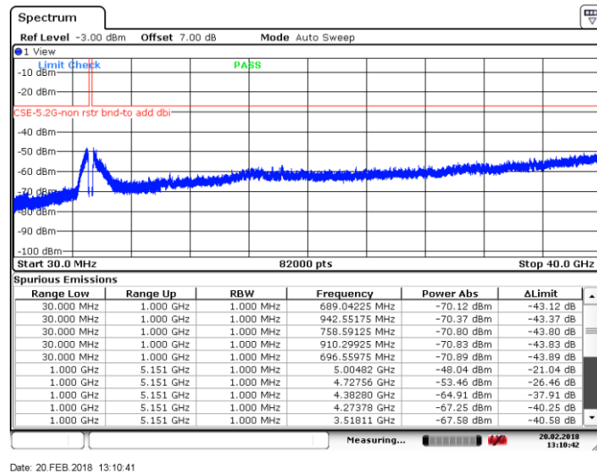
Figure 8.4-11: Spurious emissions outside restricted bands, Tx on ch 64, 802.11ac VHT20
