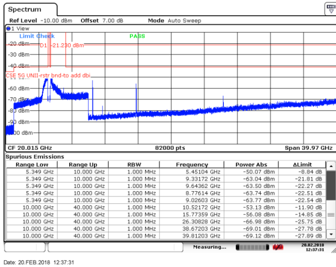
Figure 8.4-27: Spurious emissions within restricted bands, Tx on ch 52, 802.11a
