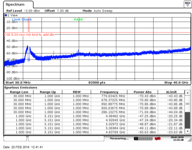
Figure 8.4-2: Spurious emissions outside restricted bands, Tx on ch 60, 802.11a
