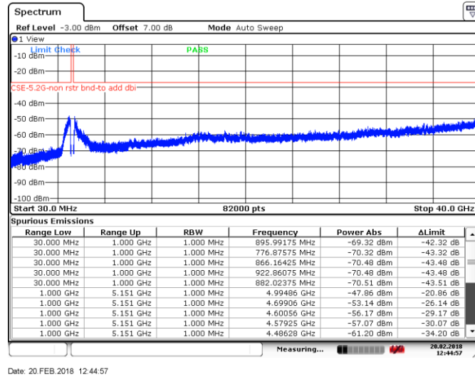
Figure 8.4-3: Spurious emissions outside restricted bands, Tx on ch 64, 802.11a
