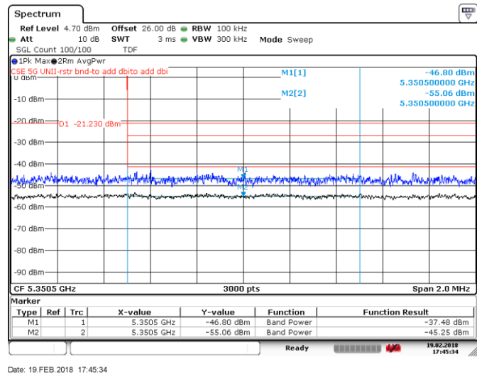
Figure 8.4-26: Upper band edge, Tx on ch 58, 802.11c VHT80
