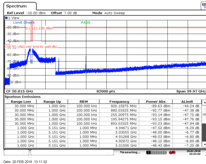
Figure 8.4-38: Spurious emissions within restricted bands, Tx on ch 64, 802.11ac VHT20
