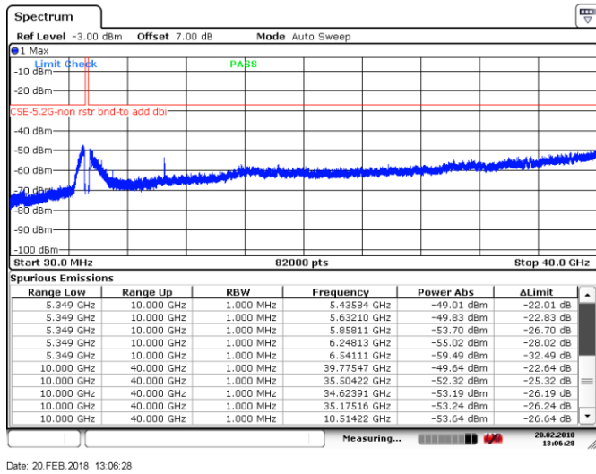
Figure 8.4-9: Spurious emissions outside restricted bands, Tx on ch 52, 802.11ac VHT20
