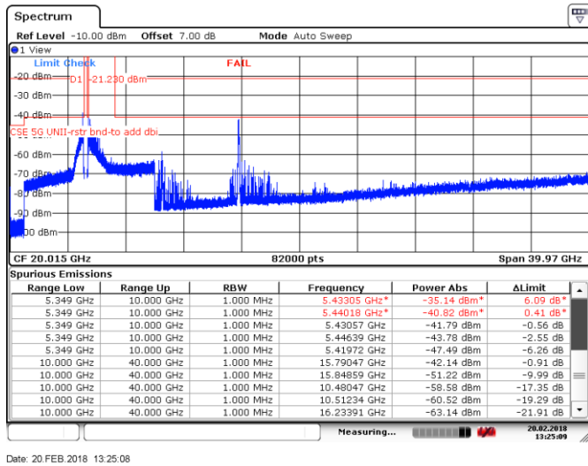
Figure 8.4-33: Spurious emissions within restricted bands, Tx on ch 54, 802.11n HT40, Peak detector
