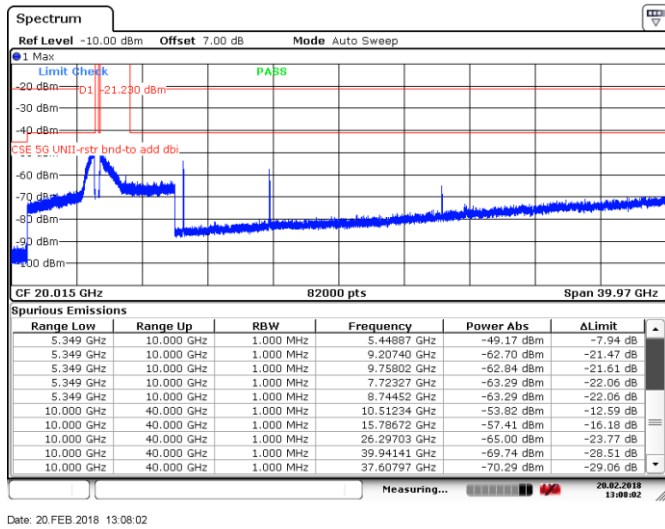
Figure 8.4-36: Spurious emissions within restricted bands, Tx on ch 52, 802.11ac VHT20
