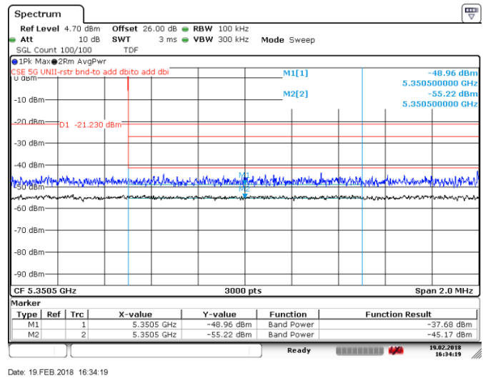
Figure 8.4-18: Upper band edge, Tx on ch 64, 802.11n HT20
