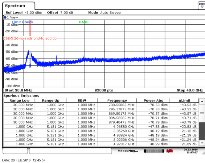
Figure 8.4-4: Spurious emissions outside restricted bands, Tx on ch 52, 802.11n HT20
