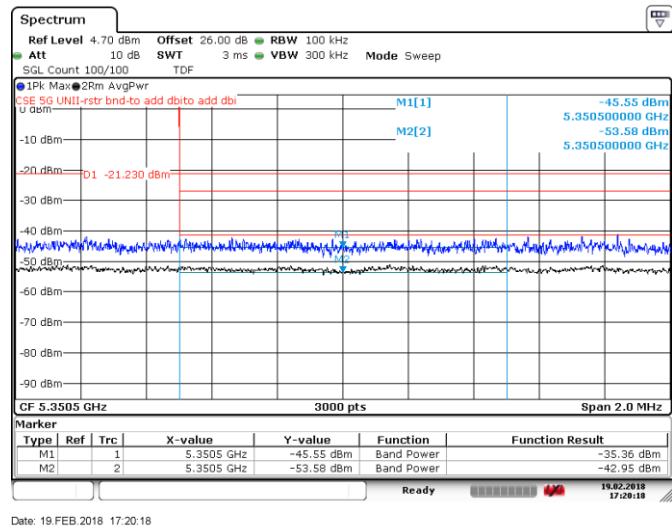
Figure 8.4-22: Upper band edge, Tx on ch 64, 802.11ac VHT20
