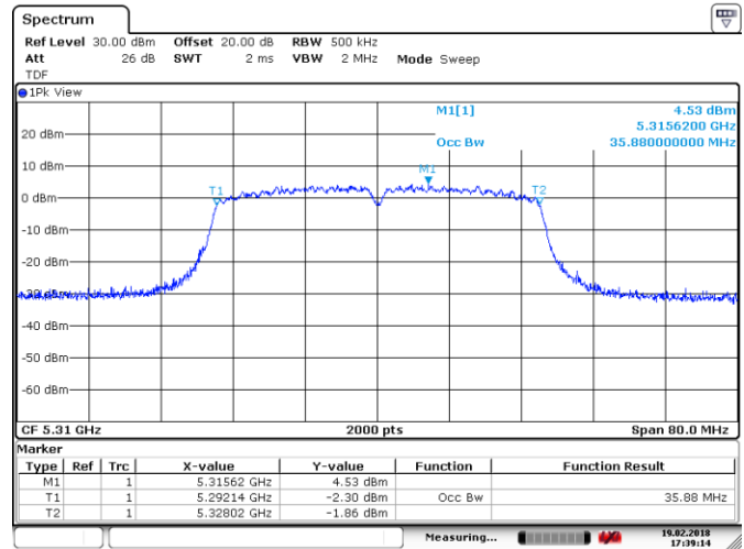
Figure 8.2-2: 99 % bandwidth on 802.11n HT40, sample plot
