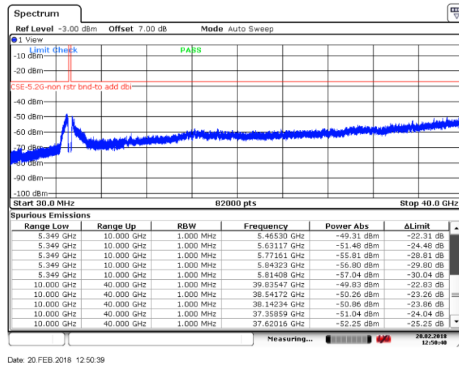
Figure 8.4-6: Spurious emissions outside restricted bands, Tx on ch 64, 802.11n HT20
