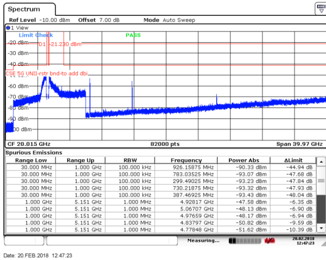
Figure 8.4-30: Spurious emissions within restricted bands, Tx on ch 52, 802.11n HT20
