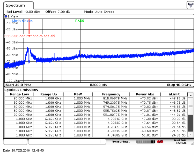
Figure 8.4-5: Spurious emissions outside restricted bands, Tx on ch 60, 802.11n HT20
