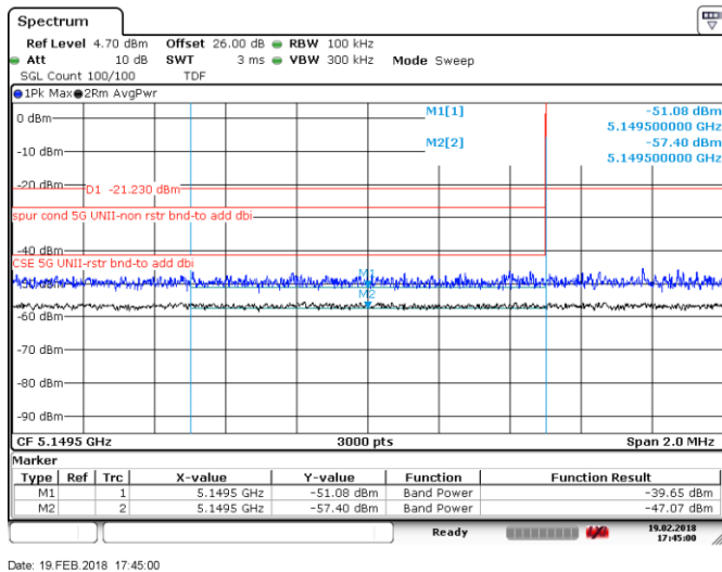
Figure 8.4-25: Lower band edge, Tx on ch 58, 802.11c VHT80
