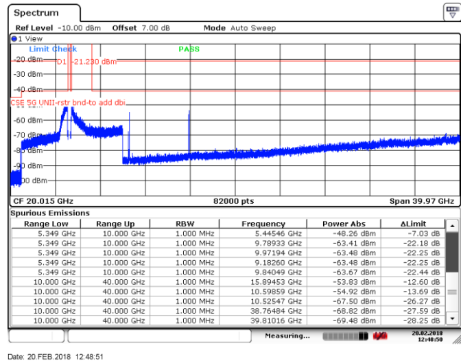
Figure 8.4-31: Spurious emissions within restricted bands, Tx on ch 60, 802.11n HT20
