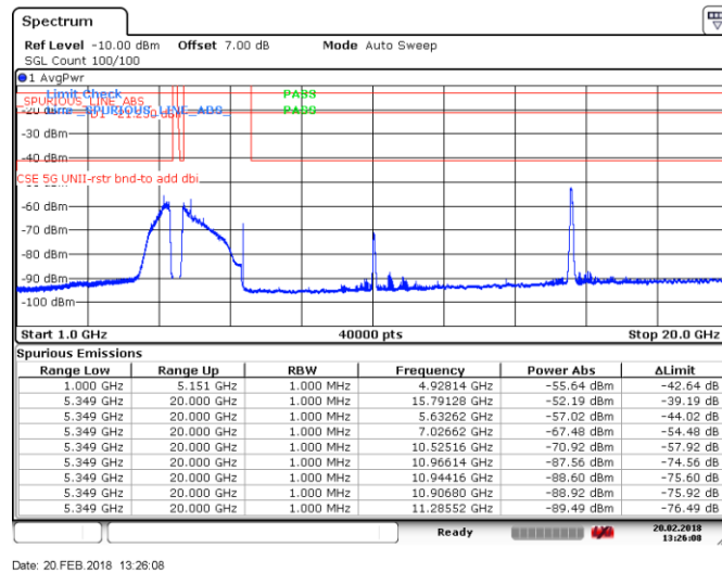
Figure 8.4-35: Spurious emissions within restricted bands, Tx on ch 54, 802.11n HT40, RMS detector
