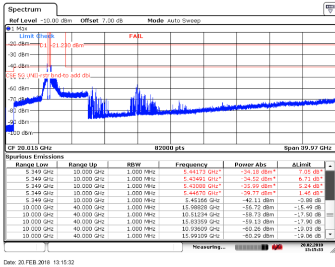
Figure 8.4-39: Spurious emissions within restricted bands, Tx on ch 54, 802.11ac VHT40, Peak detector
