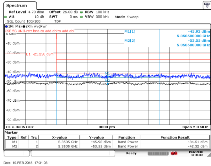
Figure 8.4-24: Upper band edge, Tx on ch 62, 802.11ac VHT40
