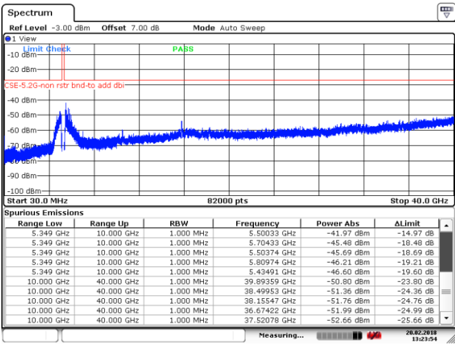
Figure 8.4-7: Spurious emissions outside restricted bands, Tx on ch 54, 802.11n HT40
