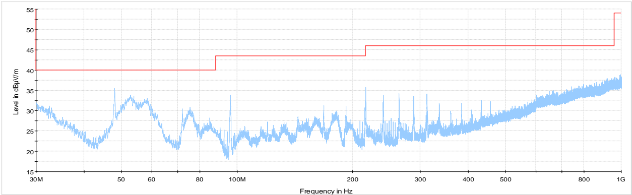
Figure 8.4-43: Cabinet Radiated spurious emission 30 MHz to 1 GHz sample plot
