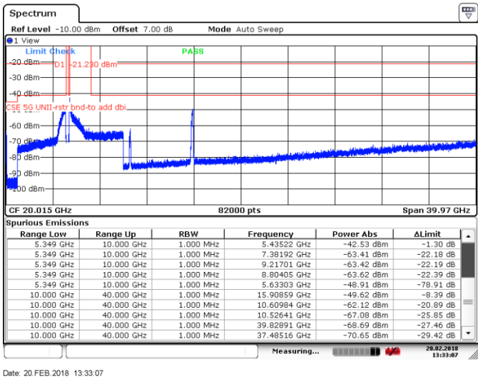
Figure 8.4-42: Spurious emissions within restricted bands, Tx on ch 58, 802.11ac VHT80
