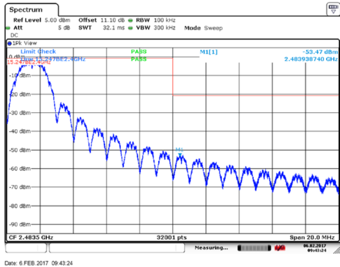
Figure 8.3.2: Bandedge Measurement, high channel, ant 0
