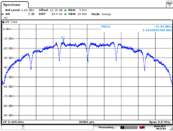
Figure 8.4-1: PSD, Low CH, ant o
