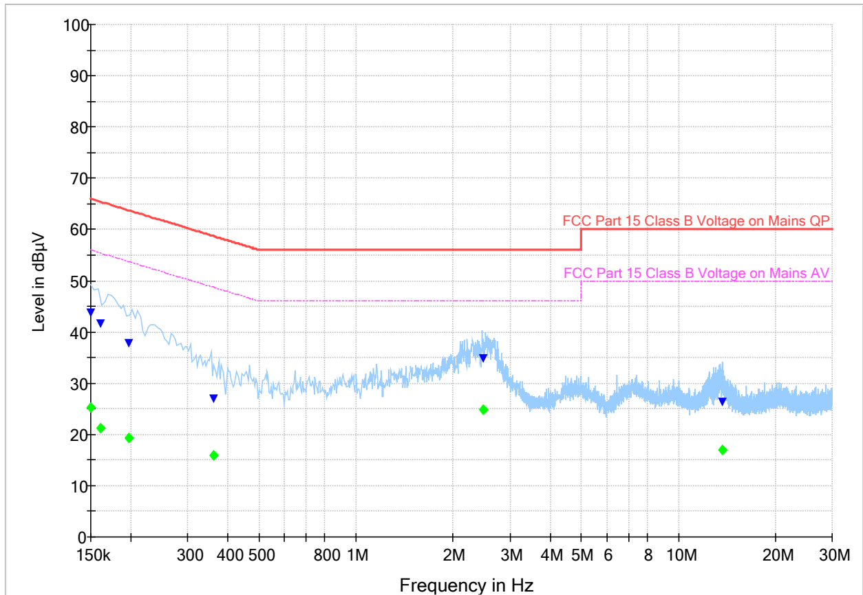
Plot 8.5-2: Conducted emissions, RF4CE CH25, ant o with RX Diversity ON, Delta Supply
