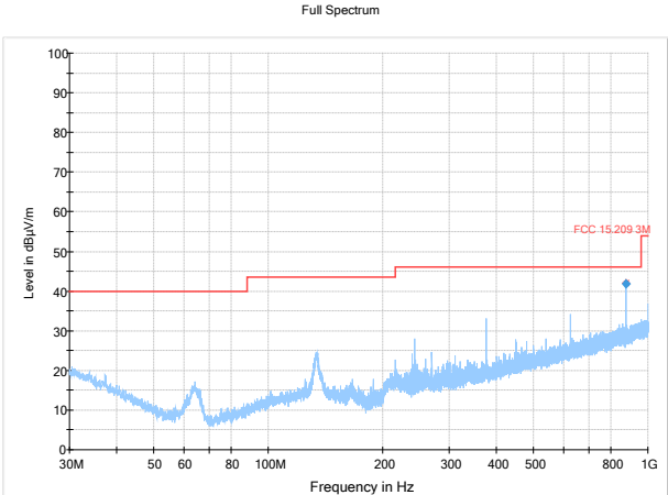
Figure 8.3.16: Radiated spurious emissions, high channel, 30-1000MHz, ant 0
