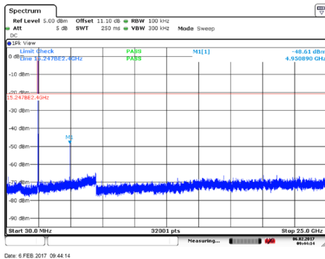
Figure 8.3.5: Conducted spurious emissions, high channel, ant 0
