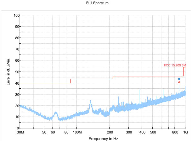
Figure 8.3.14: Radiated spurious emissions, mid channel, 30-1000MHz, ant 0
