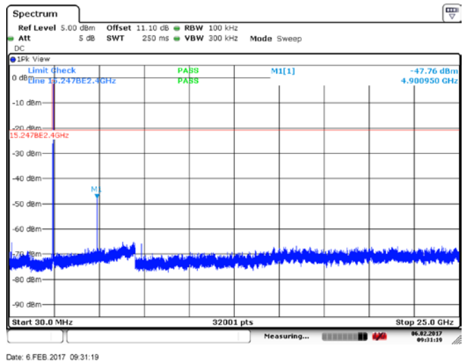
Figure 8.3.4: Conducted spurious emissions, mid channel, ant 0
