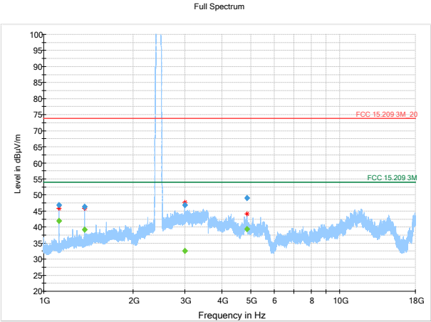
Figure 8.3.12: Radiated spurious emissions, low channel, 1-18GHz, ant 0
