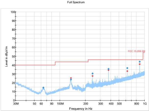
Figure 8.3.11: Radiated spurious emissions, low channel, 30-1000MHz, ant 0
