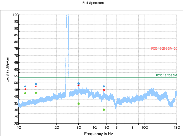
Figure 8.3.17: Radiated spurious emissions, high channel, 1-18GHz, ant 0
