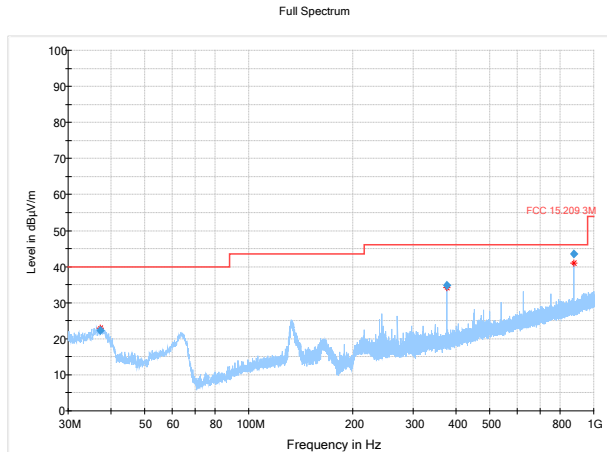
Figure 8.3.21: Radiated spurious emissions, RF4CE CH15 (2425MHz) ant 0, and BT GFSK 2480MHz, 30-1000MHz
