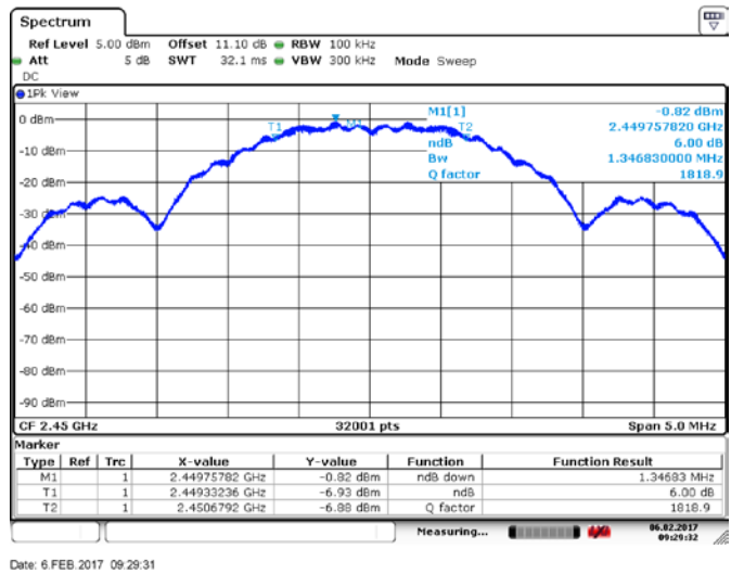
Figure 8.1-2: 6 dB bandwidth, Mid CH, Ant o
