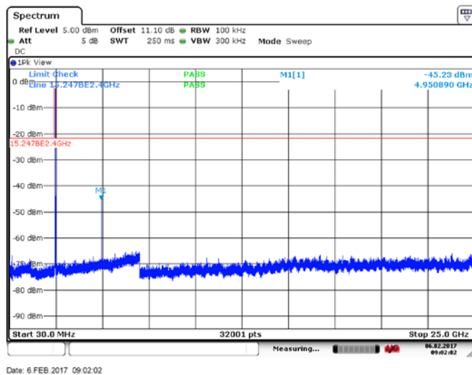
Figure 8.3.10: Conducted spurious emissions, high channel, ant 1
