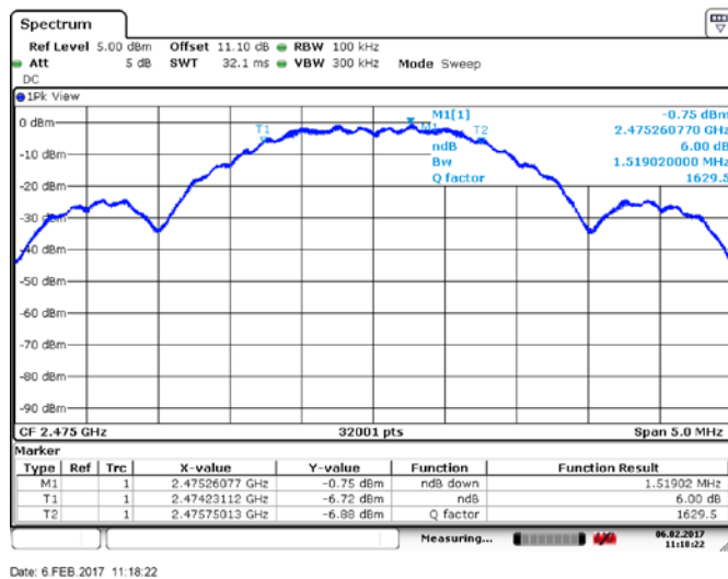
Figure 8.1-3: 6 dB bandwidth, High CH, Ant o
