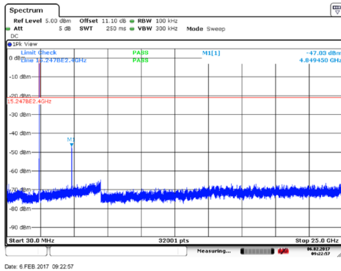
Figure 8.3.3: Conducted spurious emissions, low channel, ant 0
