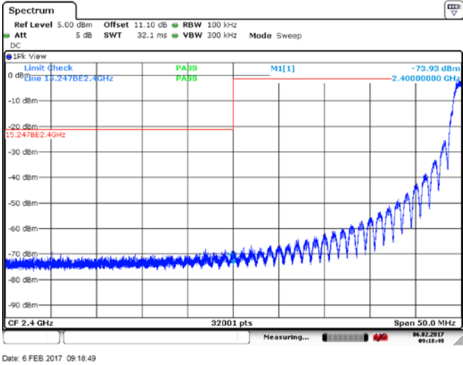
Figure 8.3.6: Bandedge Measurement, low channel, ant 1
