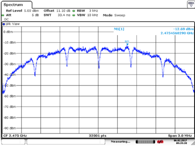
Figure 8.4-3: PSD, High CH, ant o
