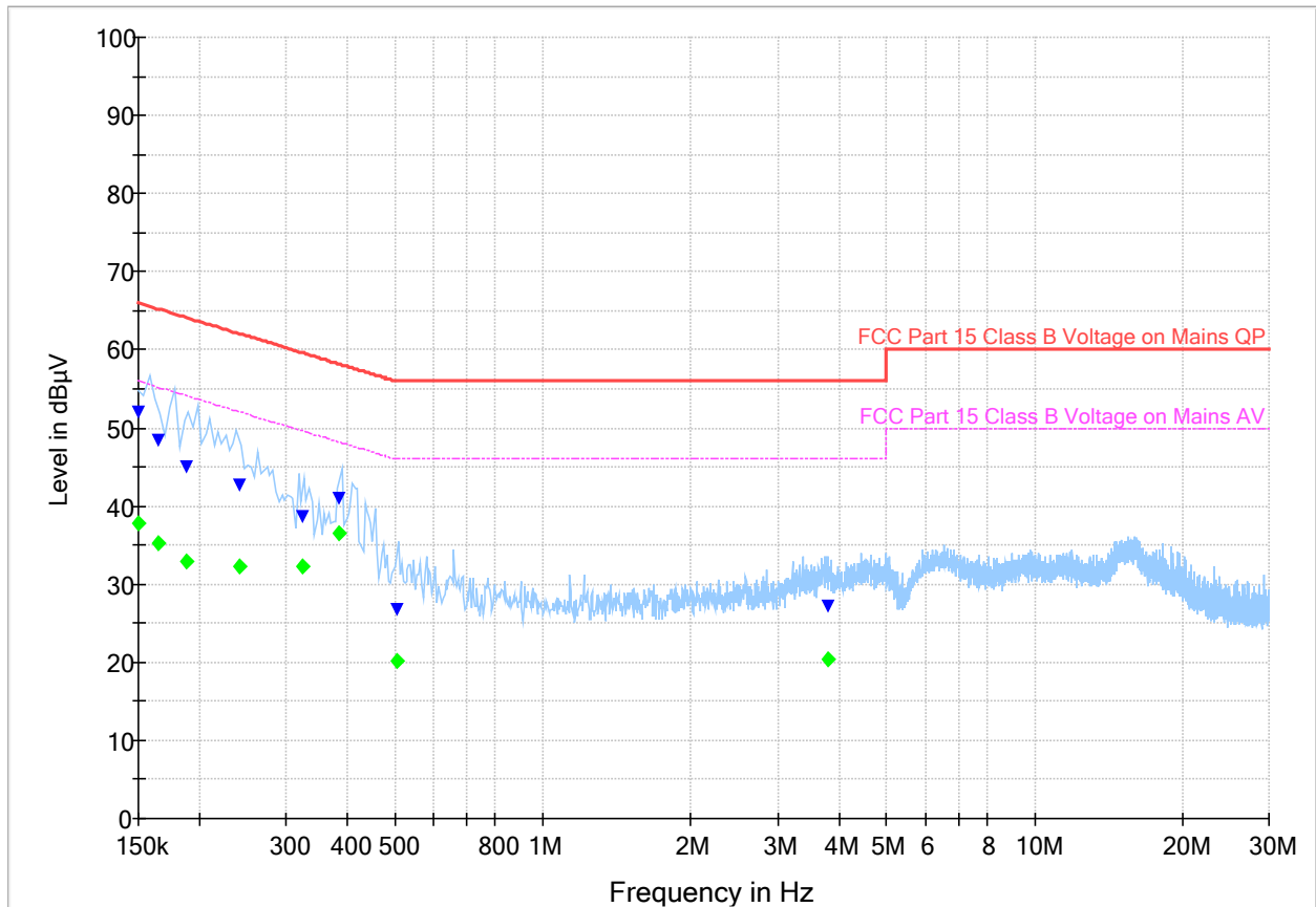
Plot 8.5-3: Conducted emissions, RF4CE CH15 ant o with RX Diversity ON, BT GFSK 2480MHz, ACBEL Supply
