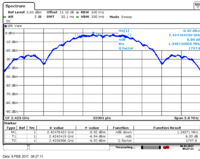
Figure 8.1-1: 6 dB bandwidth, Low CH, Ant o
