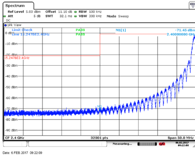
Figure 8.3.1: Bandedge Measurement, low channel, ant 0
