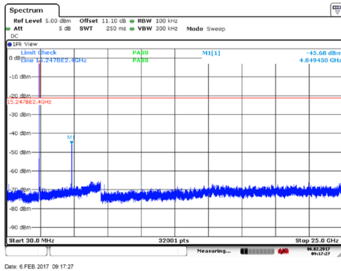
Figure 8.3.8: Conducted spurious emissions, low channel, ant 1
