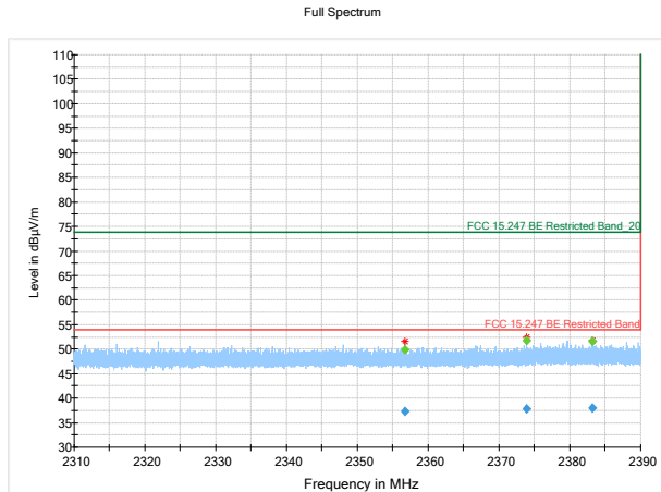
Figure 8.3.19: Radiated Bandedge in Restricted Band, low channel, ant 1
