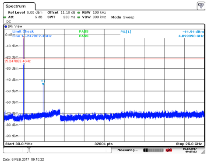
Figure 8.3.9: Conducted spurious emissions, mid channel, ant 1
