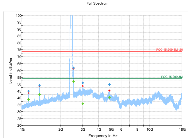
Figure 8.3.22: Radiated spurious emissions, RF4CE CH15 (2425MHz) ant 0, and BT GFSK 2480MHz, 1-18GHz
