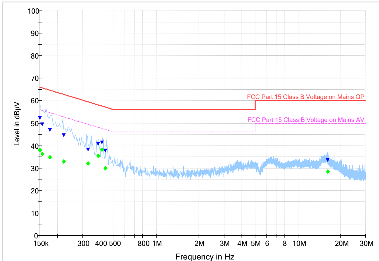
Plot 8.5-4: Conducted emissions, RF4CE CH15 ant o with RX Diversity ON, BTLE 2480MHz, ACBEL Supply
