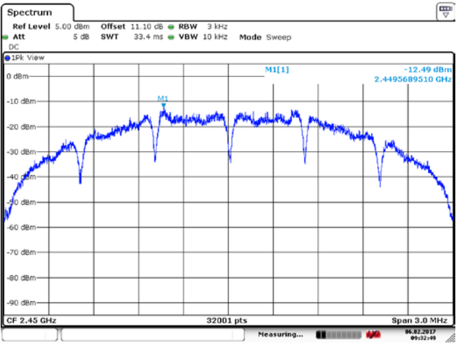
Figure 8.4-2: PSD, Mid CH, ant o
