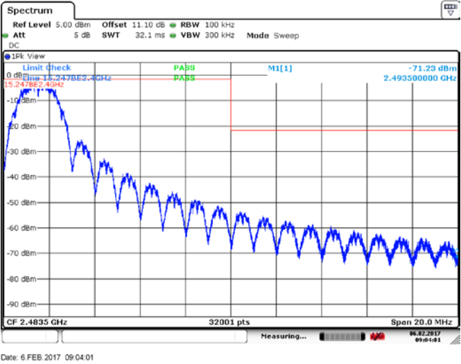
Figure 8.3.7: Bandedge Measurement, high channel, ant 1
