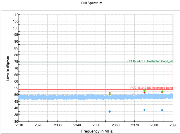
Figure 8.3.13: Radiated Bandedge in Restricted Band, low channel, ant 0
