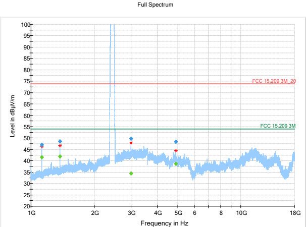
Figure 8.3.15: Radiated spurious emissions, mid channel, 1-18GHz, ant 0
