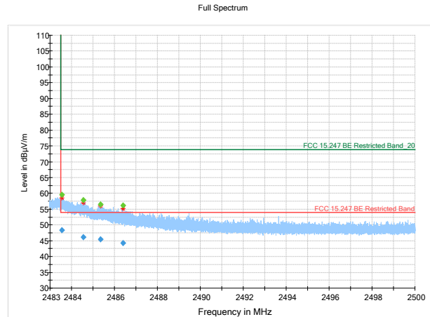
Figure 8.3.20: Radiated Bandedge in Restricted Band, high channel, ant 1
