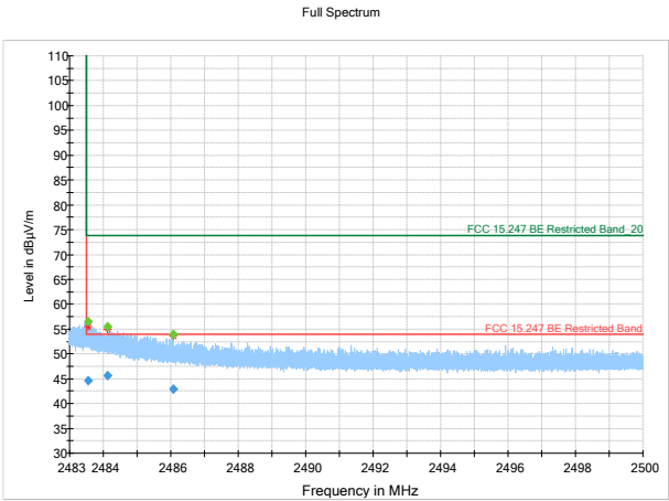
Figure 8.3.18: Radiated Bandedge in Restricted Band, high channel, ant 0
