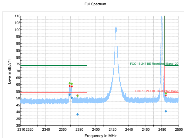
Figure 8.3.23: Radiated Bandedge in Restricted Band, RF4CE CH15 (2425MHz) ant 0, and BT GFSK 2480MHz,
