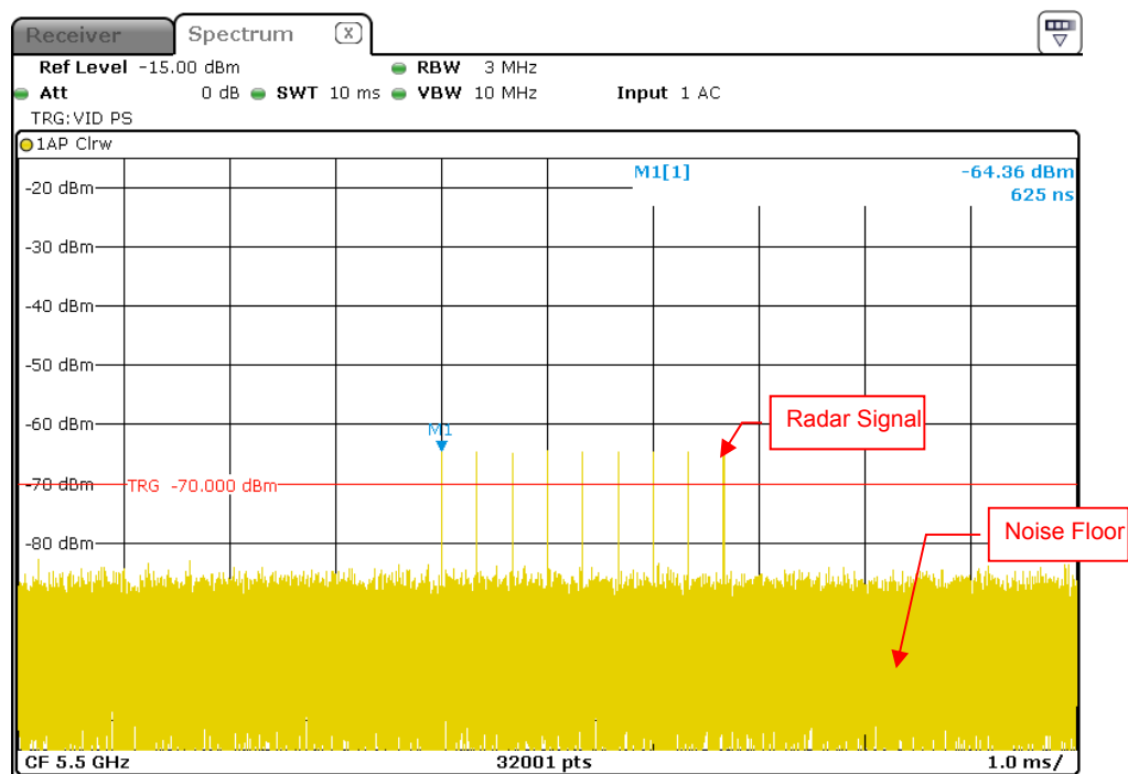
Radar Signal 6
