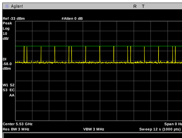
Plot 20. DFS Calibration, Radar Type 5, 5530 MHz
