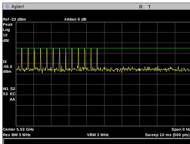
Plot 19. DFS Calibration, Radar Type 4, 5530 MHz
