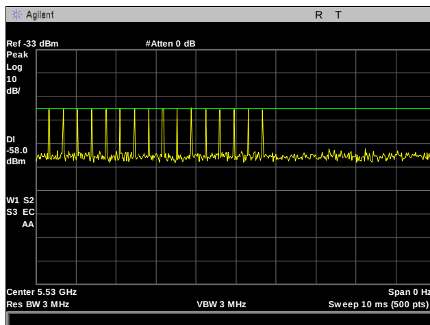
Plot 18. DFS Calibration, Radar Type 3, 5530 MHz
