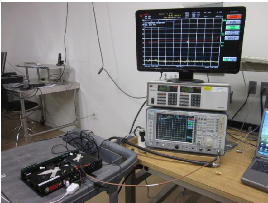
Conducted Emissions Antenna Test Setup Picture
