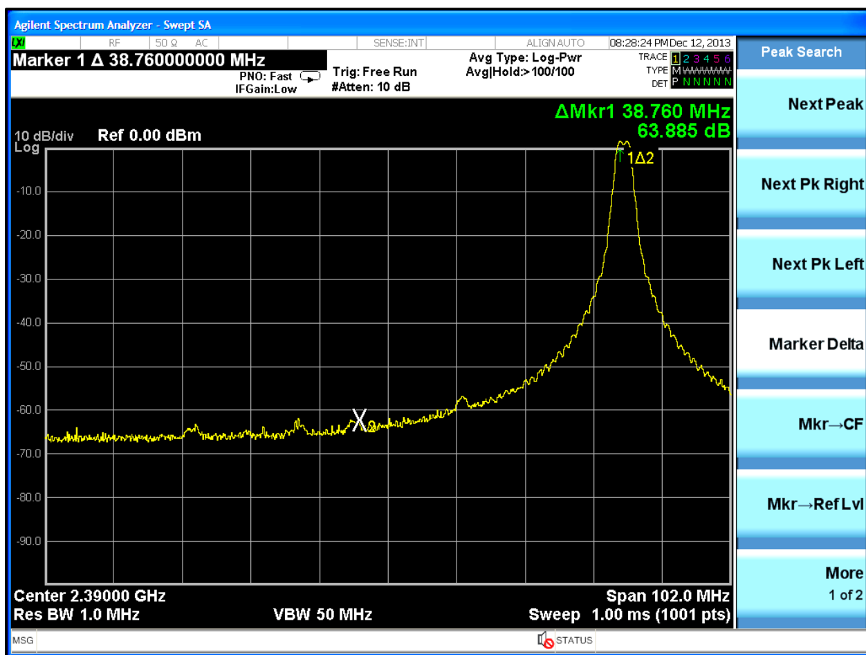
Plot 4-1: Lower Band Edge (2425 MHz)
