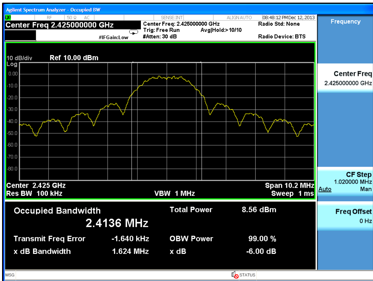
Plot 6-1: 6 dB Bandwidth (2425 MHz)
