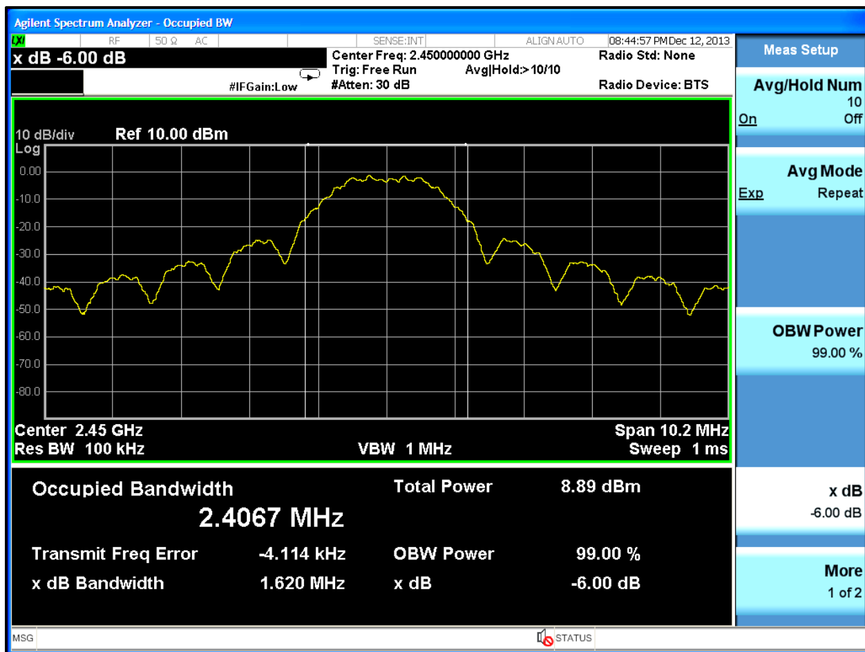
Plot 6-2: 6 dB Bandwidth (2450 MHz)
