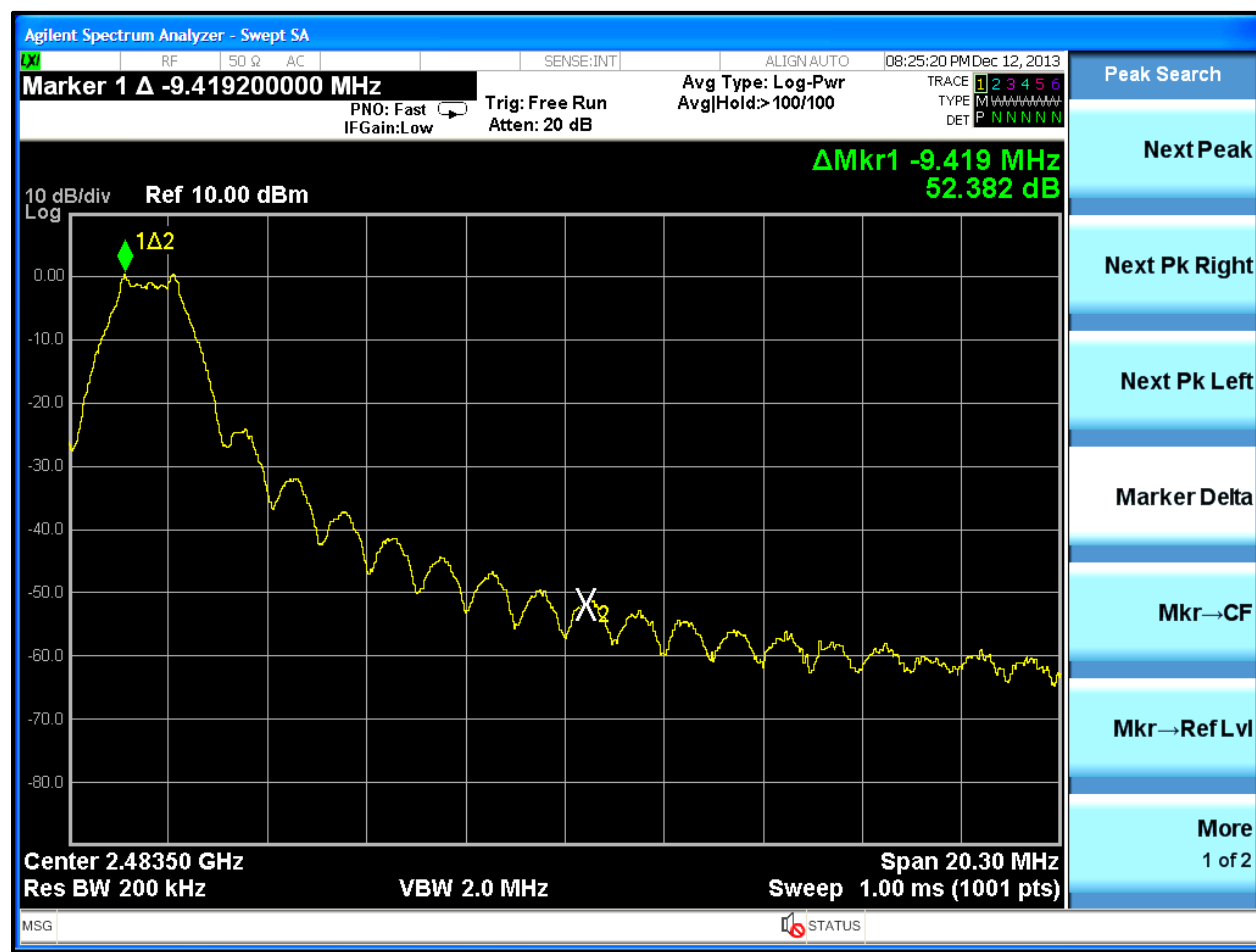
Plot 4-2: Upper Band Edge (2475 MHz)
