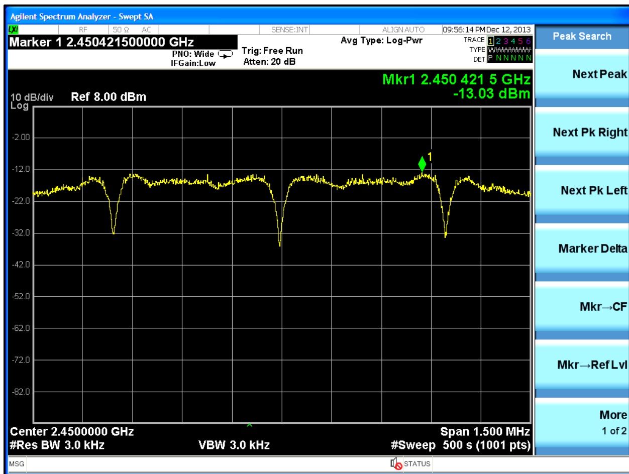
Plot 7-2: Power Spectral Density (2450 MHz)
