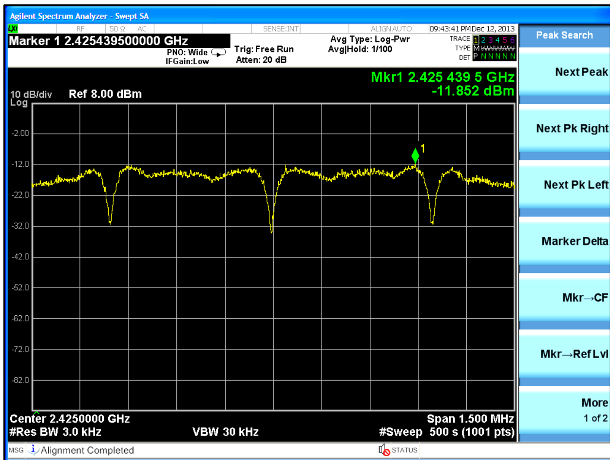
Plot 7-1: Power Spectral Density (2425 MHz)
