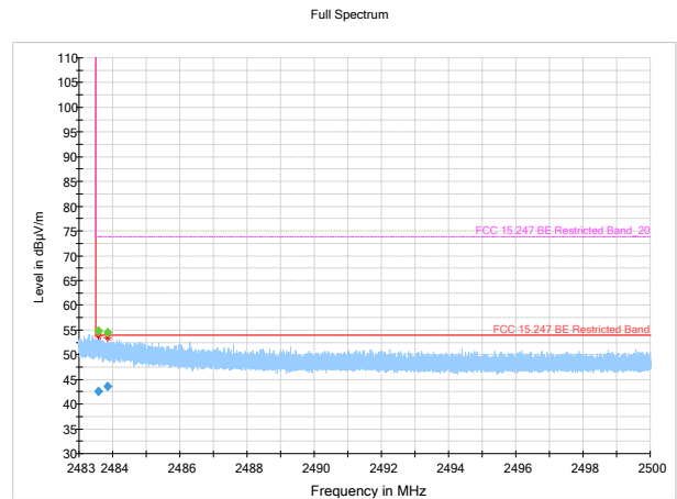
Figure 8.3.21: Radiated Bandedge in Restricted Band, high channel, ant 0
