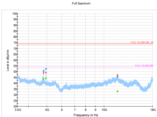
Figure 8.3.20: Radiated spurious emissions, high channel, 3.5-18GHz, ant 0
