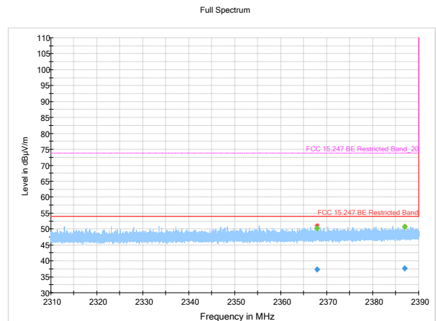
Figure 8.3.14: Radiated Bandedge in Restricted Band, low channel, ant 0
