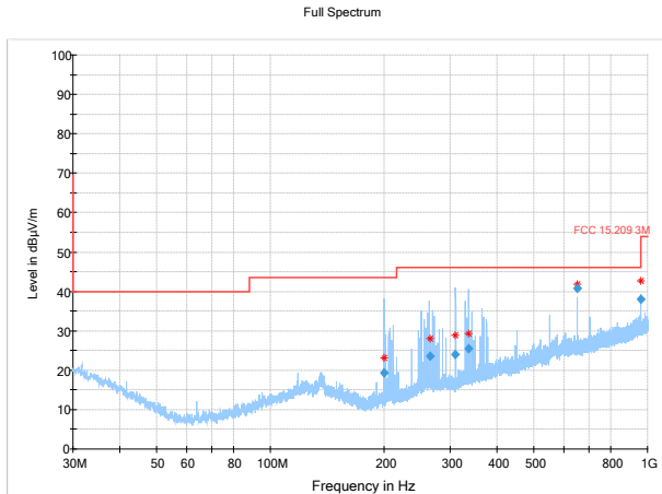
Figure 8.3.18: Radiated spurious emissions, high channel, 30-1000MHz, ant 0
