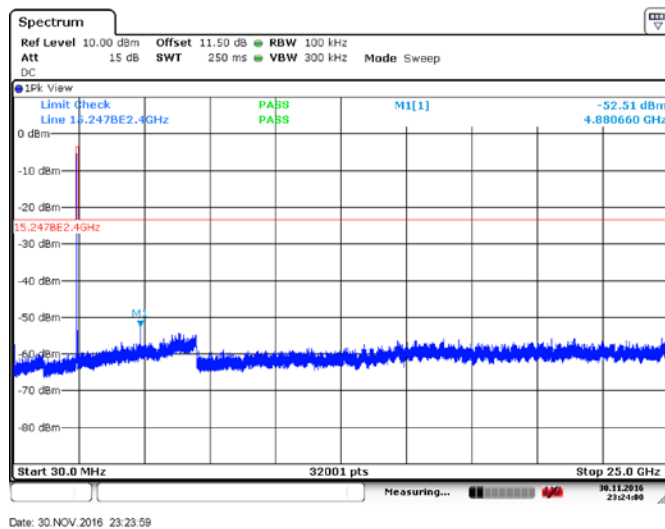
Figure 8.3.10: Conducted spurious emissions, mid channel, ant 1
