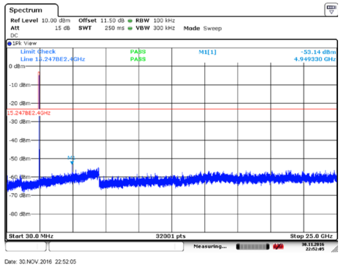
Figure 8.3.4: Conducted spurious emissions, high channel, ant 0
