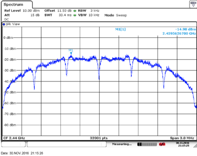
Figure 8.4-5: PSD, Mid CH, ant 1
