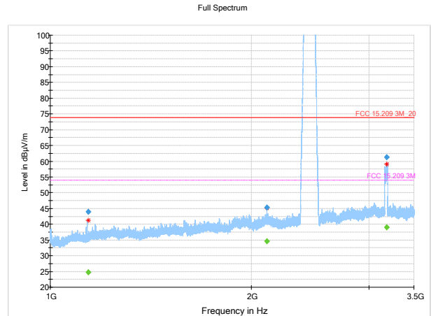
Figure 8.3.12: Radiated spurious emissions, low channel, 1-3.5GHz, ant 0
