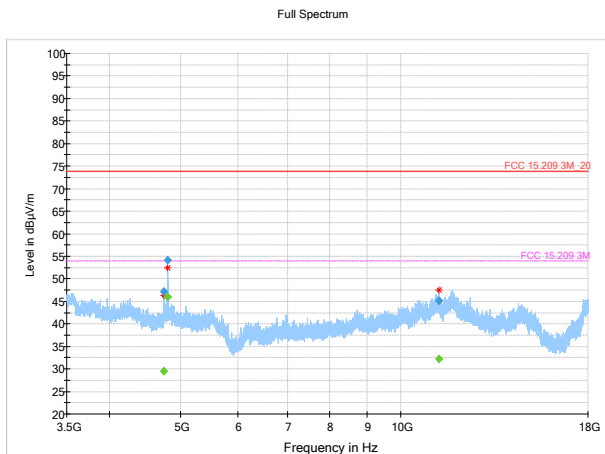
Figure 8.3.13: Radiated spurious emissions, low channel, 3.5-18GHz, ant 0
