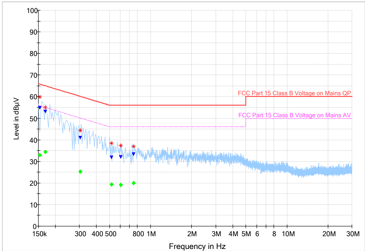
Plot 8.5-3: Conducted emissions, ant o, NetBit Supply
