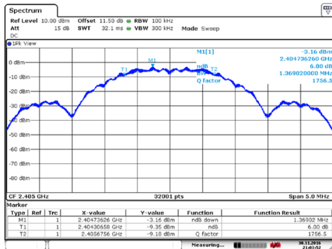
Figure 8.1-4: 6 dB bandwidth, Low CH, Ant 1
