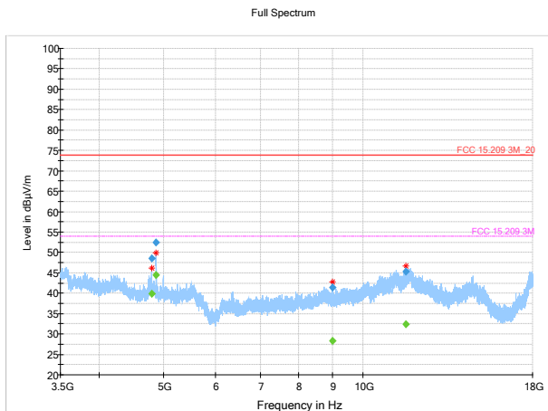
Figure 8.3.17: Radiated spurious emissions, mid channel, 3.5-18GHz, ant 0
