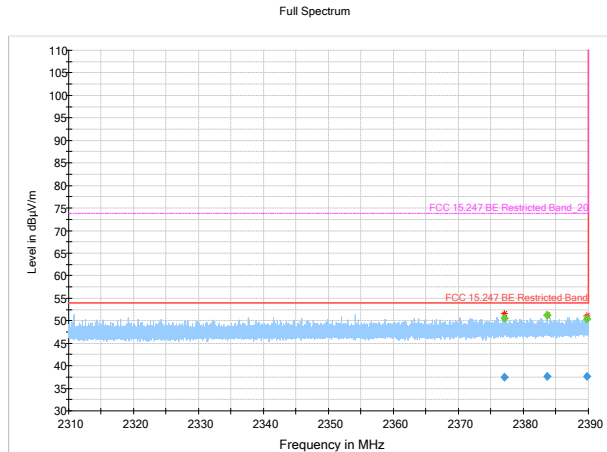
Figure 8.3.22: Radiated Bandedge in Restricted Band, low channel, ant 1
