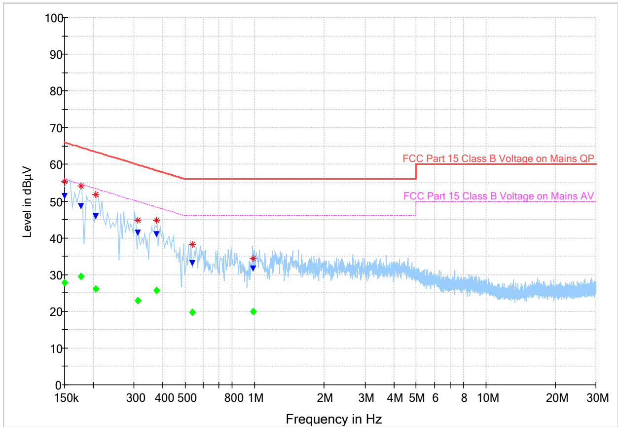
Plot 8.5-4: Conducted emissions, ant 1, NetBit Supply
