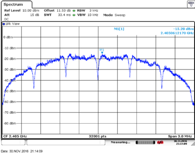
Figure 8.4-4: PSD, Low CH, ant 1
