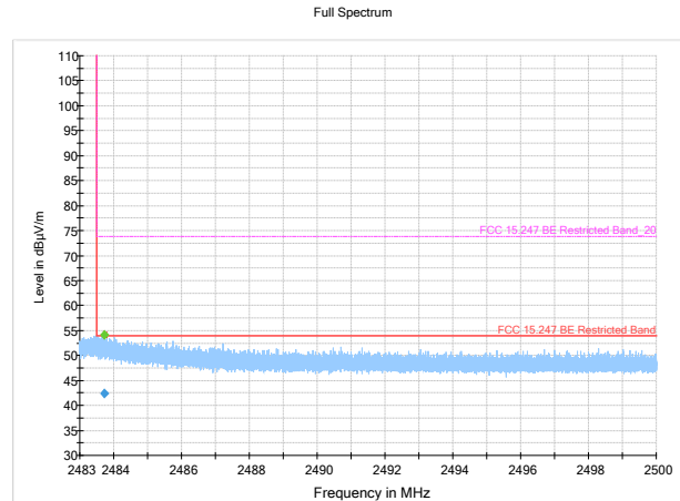
Figure 8.3.23: Radiated Bandedge in Restricted Band, high channel, ant 1
