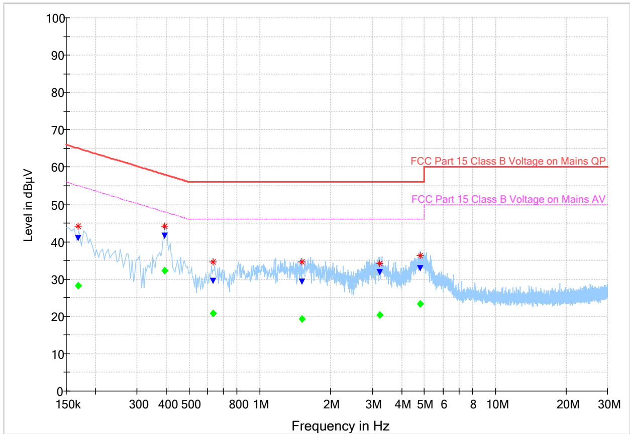
Plot 8.5-2: Conducted emissions, ant 1, ADP Supply
