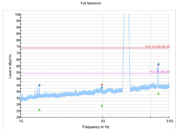
Figure 8.3.16: Radiated spurious emissions, mid channel, 1-3.5GHz, ant 0
