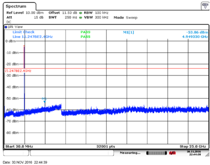
Figure 8.3.9: Conducted spurious emissions, high channel, ant 1
