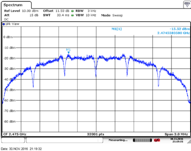
Figure 8.4-6: PSD, High CH, ant 1
