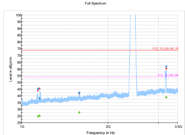
Figure 8.3.19: Radiated spurious emissions, high channel, 1-3.5GHz, ant 0
