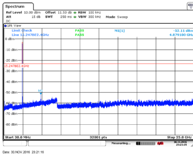
Figure 8.3.5: Conducted spurious emissions, mid channel, ant 0
