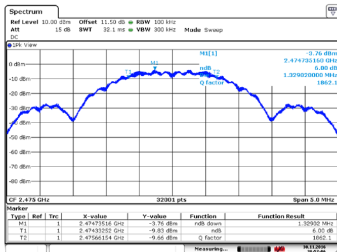
Figure 8.1-6: 6 dB bandwidth, High CH, Ant 1
