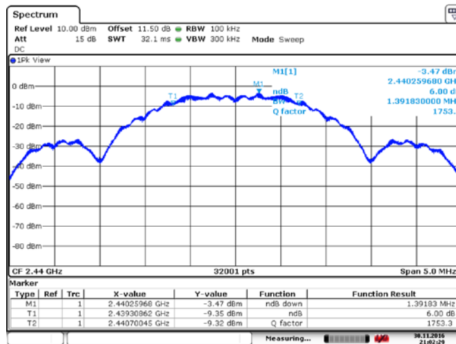
Figure 8.1-5: 6 dB bandwidth, Mid CH, Ant 1
