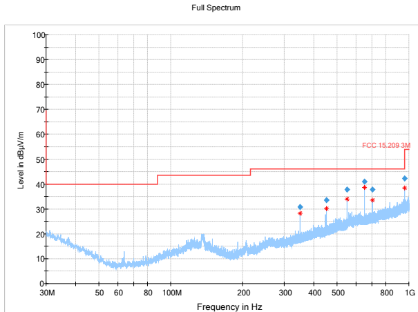
Figure 8.3.15: Radiated spurious emissions, mid channel, 30-1000MHz, ant 0
