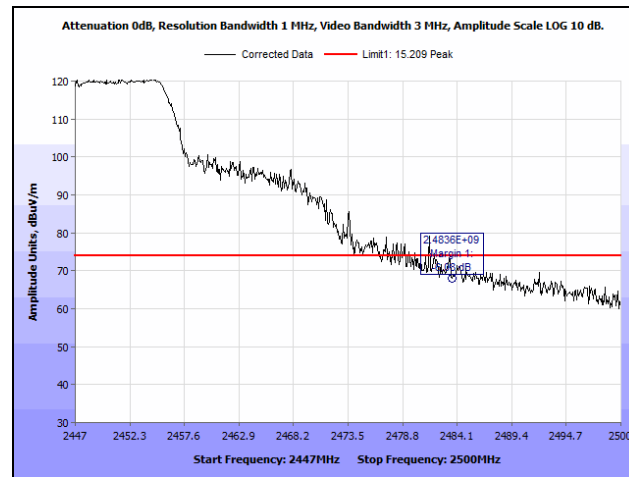
Plot 231. Radiated Restricted Band Edge, 2447 MHz, 802.11n 20 MHz, SISO, Peak
