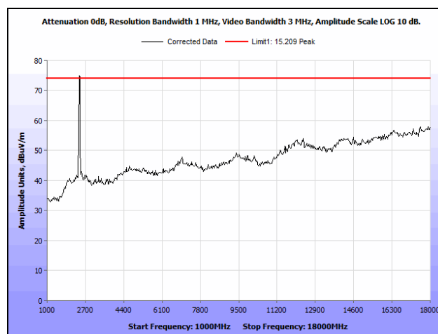
Plot 159. Radiated Spurious Emissions, Low Channel, 802.11n 40 MHz, 1 GHz – 18 GHz, Peak, SISO
