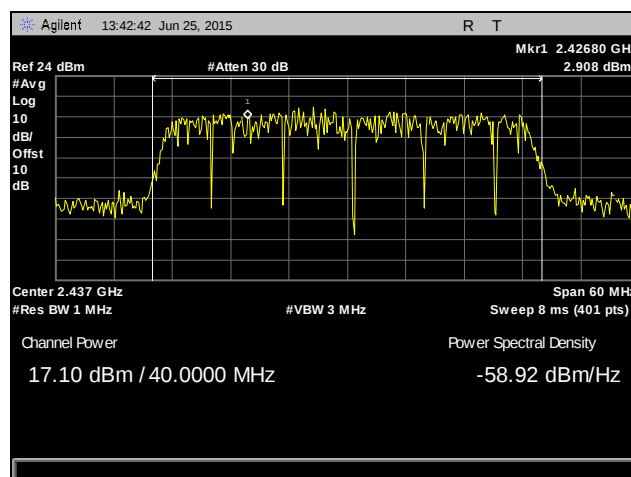
Plot 86. Peak Power Output, 2437 MHz, 802.11n 40 MHz, MIMO
