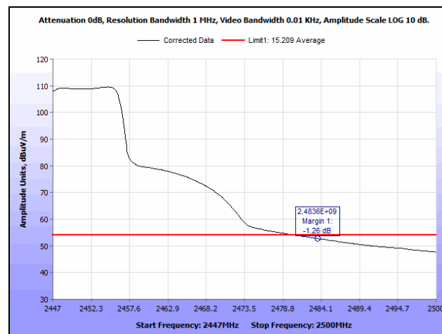
Plot 230. Radiated Restricted Band Edge, 2447 MHz, 802.11n 20 MHz, SISO, Average
