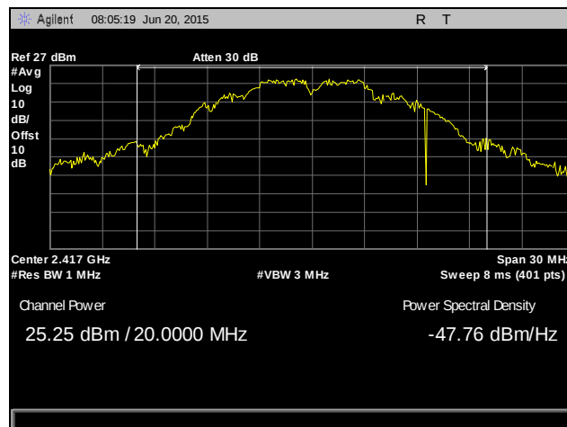
Plot 47. Peak Power Output, 2417 MHz, 802.11b, SISO
