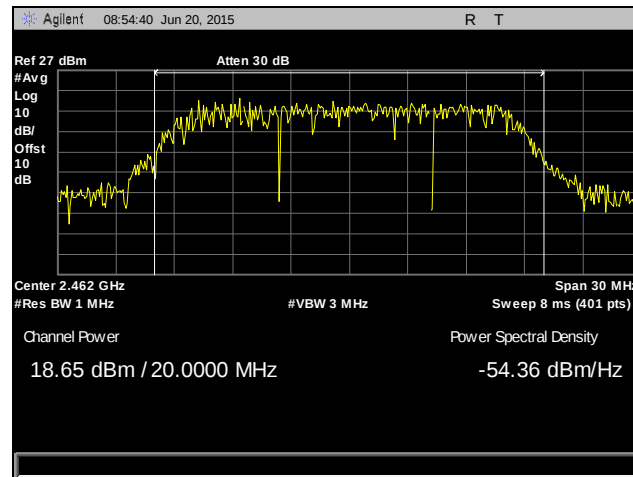
Plot 72. Peak Power Output, 2462 MHz, 802.11n 20 MHz, MIMO
