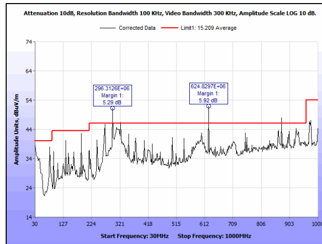
Plot 145. Radiated Spurious Emissions, High Channel, 802.11n 20 MHz, 30 MHz – 1 GHz, SISO
