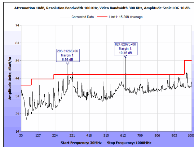
Plot 121. Radiated Spurious Emissions, Low Channel, 802.11g, 30 MHz – 1 GHz, SISO
