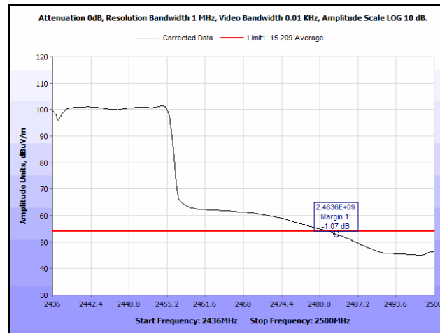
Plot 258. Radiated Restricted Band Edge, 2437 MHz, 802.11n 40 MHz, SISO, Average
