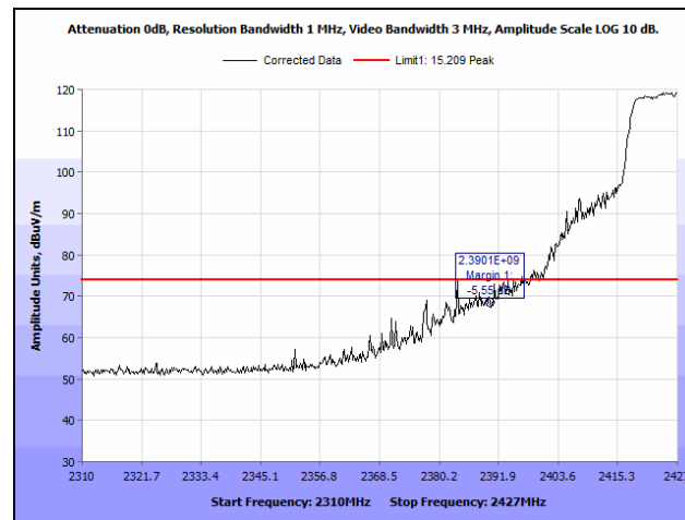
Plot 223. Radiated Restricted Band Edge, 2427 MHz, 802.11n 20 MHz, SISO, Peak
