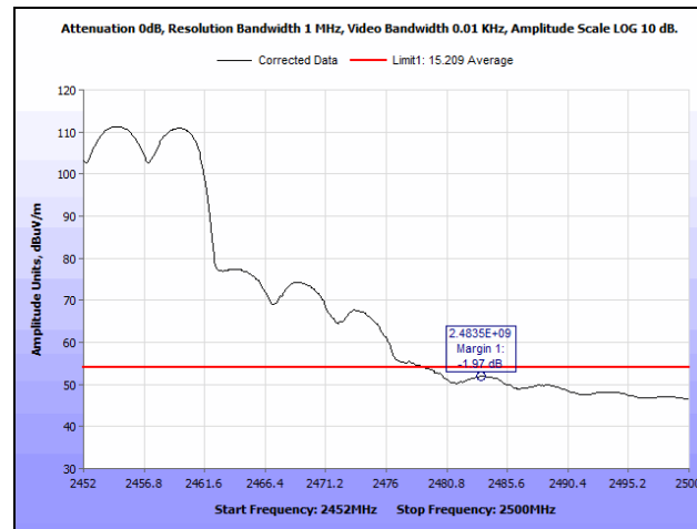
Plot 210. Radiated Restricted Band Edge, 2452 MHz, 802.11n 20 MHz, MIMO, Average
