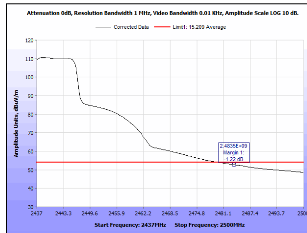
Plot 226. Radiated Restricted Band Edge, 2437 MHz, 802.11n 20 MHz, SISO, Average
