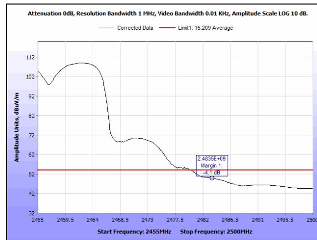
Plot 182. Radiated Restricted Band Edge, 2457 MHz, 802.11g, MIMO, Average
