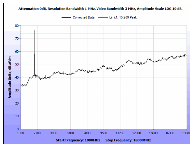
Plot 135. Radiated Spurious Emissions, Mid Channel, 802.11n 20 MHz, 1 GHz – 18 GHz, Peak, MIMO
