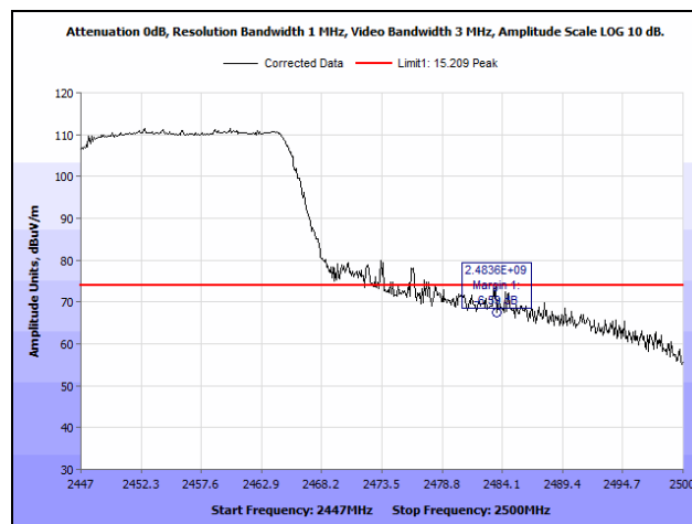
Plot 263. Radiated Restricted Band Edge, 2447 MHz, 802.11n 40 MHz, SISO, Peak
