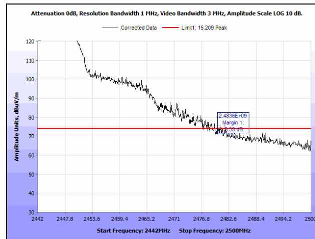
Plot 229. Radiated Restricted Band Edge, 2442 MHz, 802.11n 20 MHz, SISO, Peak
