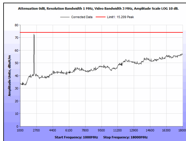
Plot 153. Radiated Spurious Emissions, Mid Channel, 802.11n 40 MHz, 1 GHz – 18 GHz, Peak, MIMO
