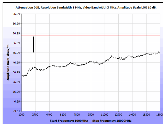
Plot 111. Radiated Spurious Emissions, High Channel, 802.11b, 1 GHz – 18 GHz, Peak, SISO
