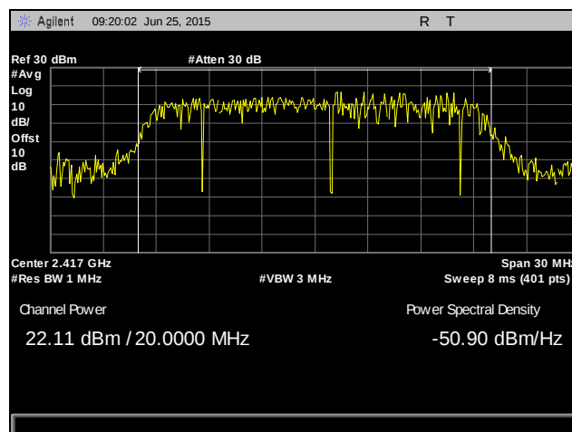
Plot 74. Peak Power Output, 2417 MHz, 802.11n 20 MHz, SISO
