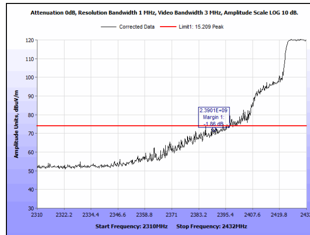
Plot 225. Radiated Restricted Band Edge, 2432 MHz, 802.11n 20 MHz, SISO, Peak
