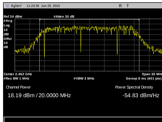
Plot 83. Peak Power Output, 2462 MHz, 802.11n 20 MHz, SISO
