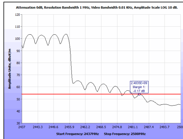
Plot 244. Radiated Restricted Band Edge, 2437 MHz, 802.11n 40 MHz, MIMO, Average
