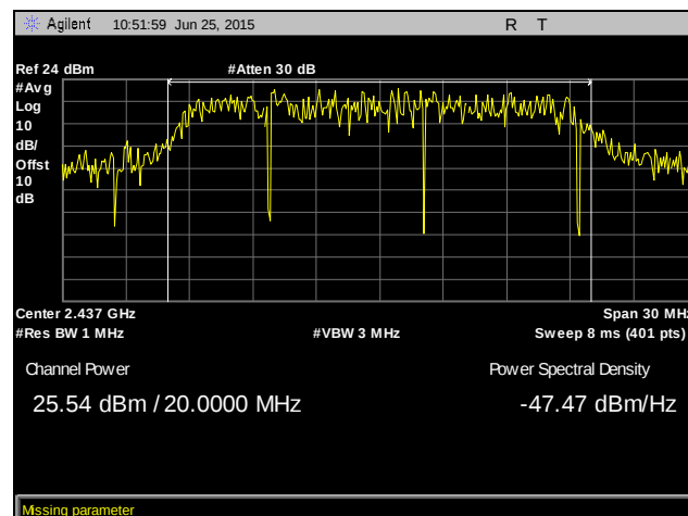
Plot 78. Peak Power Output, 2437 MHz, 802.11n 20 MHz, SISO
