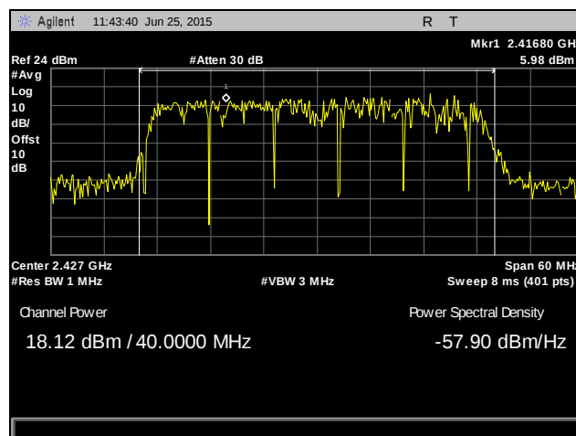
Plot 91. Peak Power Output, 2427 MHz, 802.11n 40 MHz, SISO
