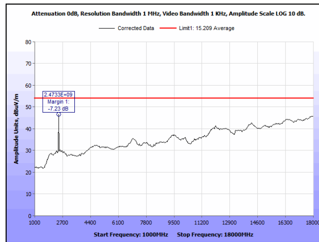
Plot 146. Radiated Spurious Emissions, High Channel, 802.11n 20 MHz, 1 GHz – 18 GHz, Average, SISO
