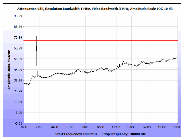
Plot 114. Radiated Spurious Emissions, Low Channel, 802.11g, 1 GHz – 18 GHz, Peak, MIMO
