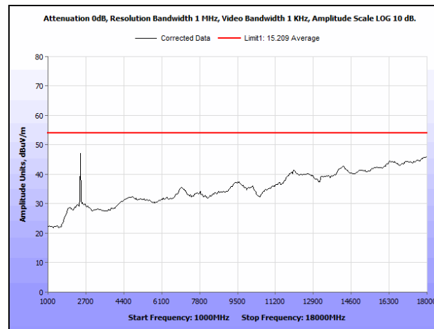
Plot 164. Radiated Spurious Emissions, High Channel, 802.11n 40 MHz, 1 GHz – 18 GHz, Average, SISO
