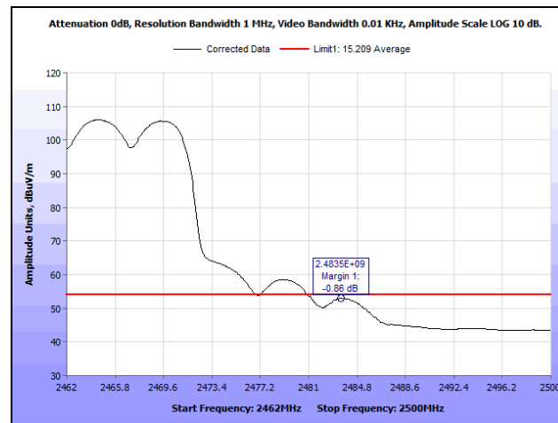
Plot 214. Radiated Restricted Band Edge, 2462 MHz, 802.11n 20 MHz, MIMO, Average
