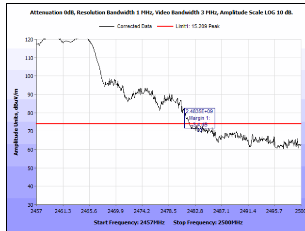
Plot 213. Radiated Restricted Band Edge, 2457 MHz, 802.11n 20 MHz, MIMO, Peak
