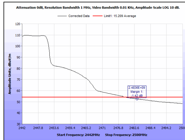
Plot 228. Radiated Restricted Band Edge, 2442 MHz, 802.11n 20 MHz, SISO, Average
