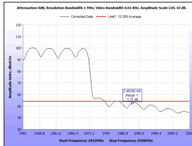
Plot 250. Radiated Restricted Band Edge, 2452 MHz, 802.11n 40 MHz, MIMO, Average
