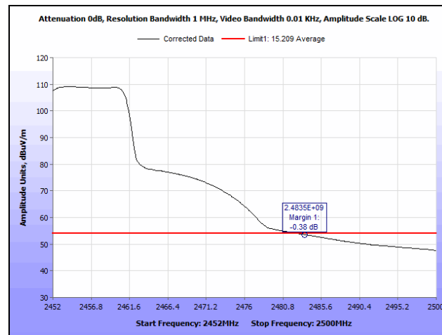
Plot 232. Radiated Restricted Band Edge, 2452 MHz, 802.11n 20 MHz, SISO, Average
