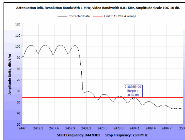
Plot 248. Radiated Restricted Band Edge, 2447 MHz, 802.11n 40 MHz, MIMO, Average
