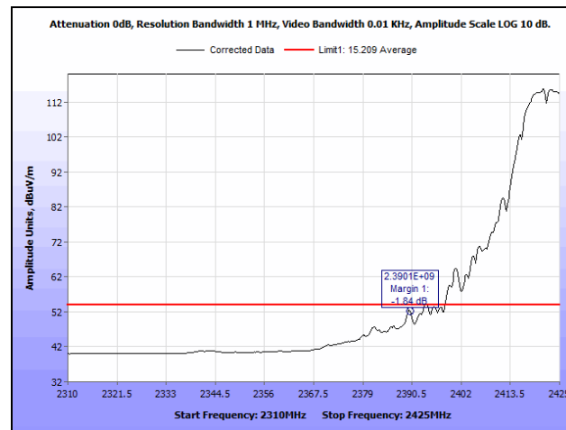
Plot 174. Radiated Restricted Band Edge, 2422 MHz, 802.11b, SISO, Average
