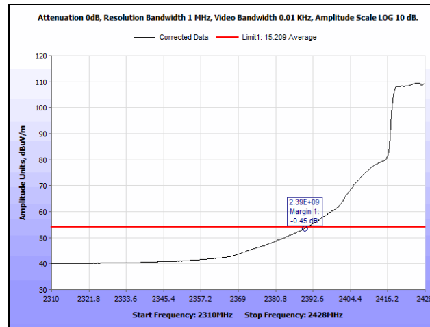
Plot 222. Radiated Restricted Band Edge, 2427 MHz, 802.11n 20 MHz, SISO, Average
