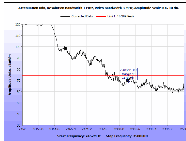
Plot 211. Radiated Restricted Band Edge, 2452 MHz, 802.11n 20 MHz, MIMO, Peak
