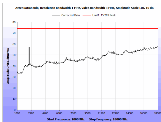
Plot 105. Radiated Spurious Emissions, Low Channel, 802.11b, 1 GHz – 18 GHz, Peak, SISO
