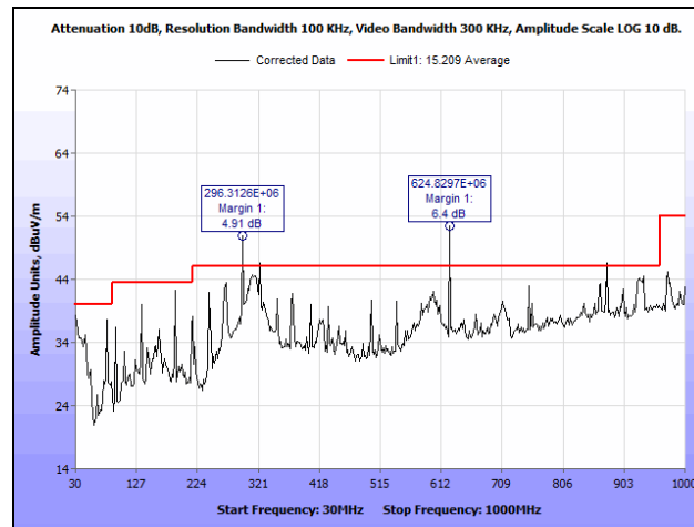
Plot 133. Radiated Spurious Emissions, Mid Channel, 802.11n 20 MHz, 30 MHz – 1GHz, MIMO
