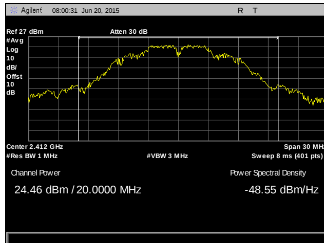
Plot 46. Peak Power Output, 2412 MHz, 802.11b, SISO
