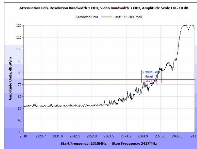
Plot 207. Radiated Restricted Band Edge, 2417 MHz, 802.11n 20 MHz, MIMO, Peak
