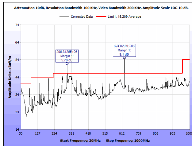
Plot 100. Radiated Spurious Emissions, High Channel, 802.11b, 30 MHz – 1 GHz, MIMO
