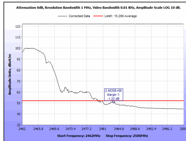
Plot 168. Radiated Restricted Band Edge, 2462 MHz, 802.11b, MIMO, Average
