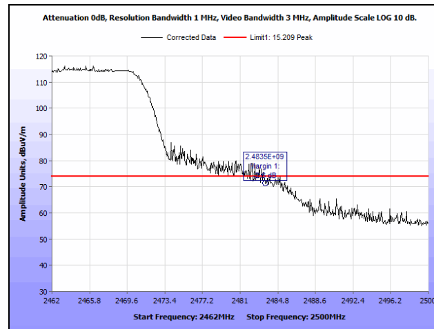
Plot 237. Radiated Restricted Band Edge, 2462 MHz, 802.11n 20 MHz, SISO, Peak
