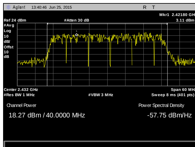
Plot 85. Peak Power Output, 2432 MHz, 802.11n 40 MHz, MIMO
