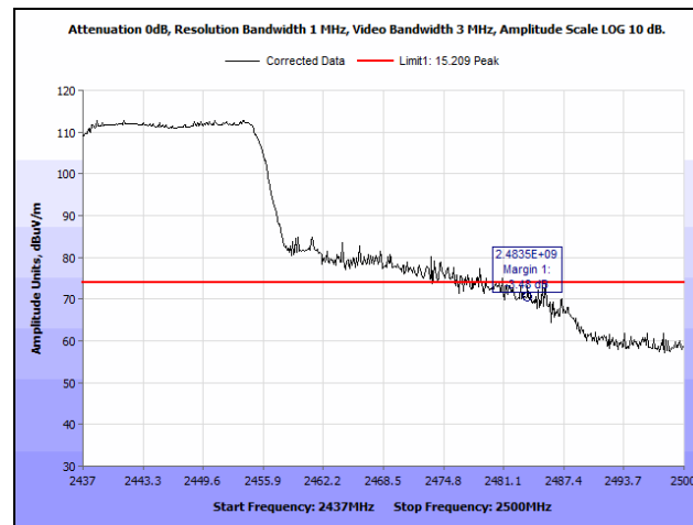
Plot 259. Radiated Restricted Band Edge, 2437 MHz, 802.11n 40 MHz, SISO, Peak
