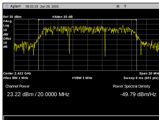
Plot 75. Peak Power Output, 2422 MHz, 802.11n 20 MHz, SISO
