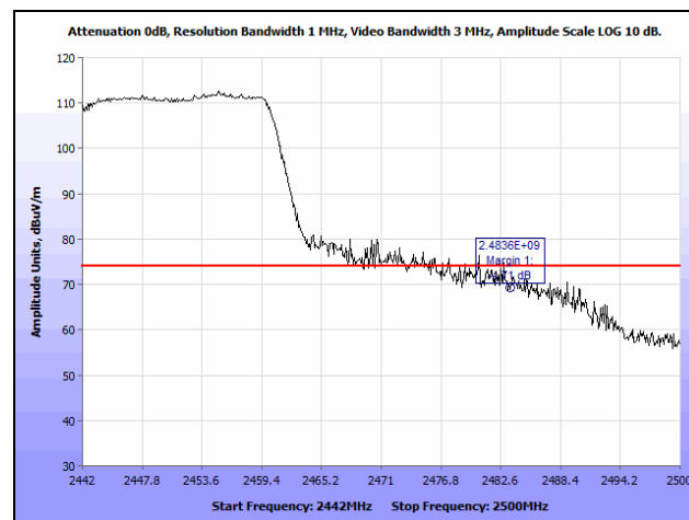
Plot 260. Radiated Restricted Band Edge, 2442 MHz, 802.11n 40 MHz, SISO, Peak
