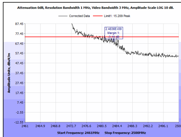
Plot 203. Radiated Restricted Band Edge, 2462 MHz, 802.11g, SISO, Peak
