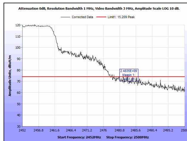
Plot 233. Radiated Restricted Band Edge, 2452 MHz, 802.11n 20 MHz, SISO, Peak
