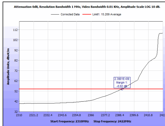
Plot 192. Radiated Restricted Band Edge, 2427 MHz, 802.11g, SISO, Average
