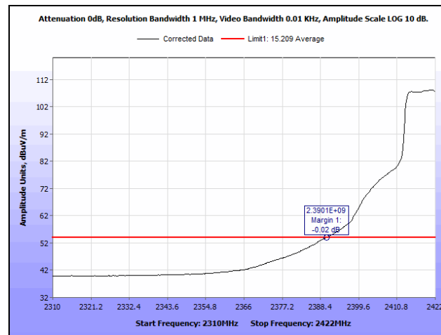
Plot 190. Radiated Restricted Band Edge, 2422 MHz, 802.11g, SISO, Average
