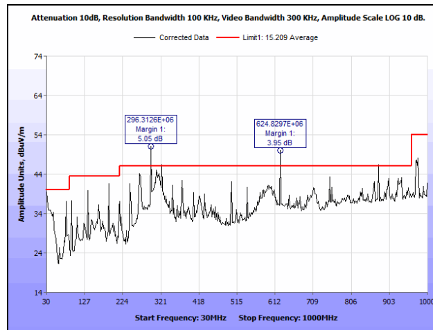
Plot 142. Radiated Spurious Emissions, Mid Channel, 802.11n 20 MHz, 30 MHz – 1 GHz, SISO
