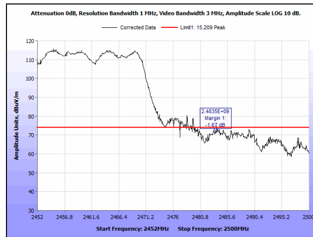
Plot 251. Radiated Restricted Band Edge, 2452 MHz, 802.11n 40 MHz, MIMO, Peak
