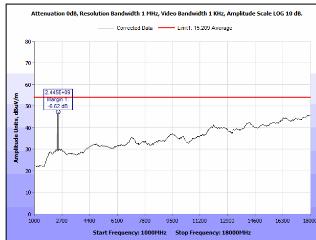
Plot 134. Radiated Spurious Emissions, Mid Channel, 802.11n 20 MHz, 1 GHz – 18 GHz, Average, MIMO
