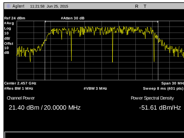
Plot 82. Peak Power Output, 2457 MHz, 802.11n 20 MHz, SISO
