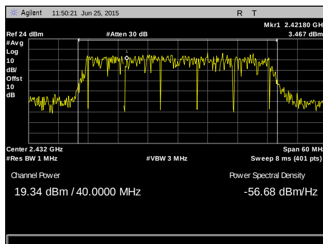
Plot 92. Peak Power Output, 2432 MHz, 802.11n 40 MHz, SISO
