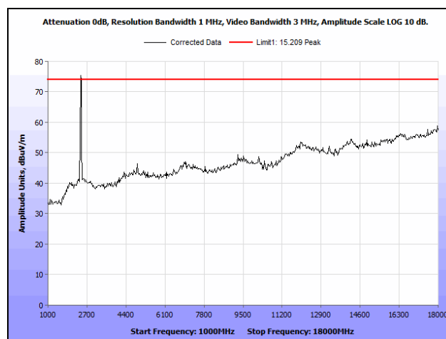
Plot 150. Radiated Spurious Emissions, Low Channel, 802.11n 40 MHz, 1 GHz – 18 GHz, Peak, MIMO
