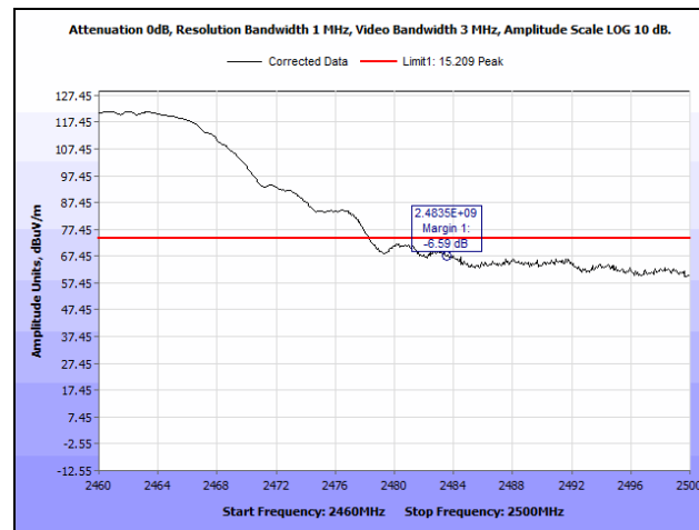
Plot 169. Radiated Restricted Band Edge, 2462 MHz, 802.11b, MIMO, Peak
