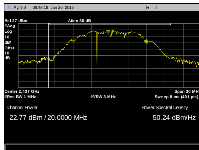
Plot 44. Peak Power Output, Mid Channel, 802.11b, MIMO, Antenna 1
