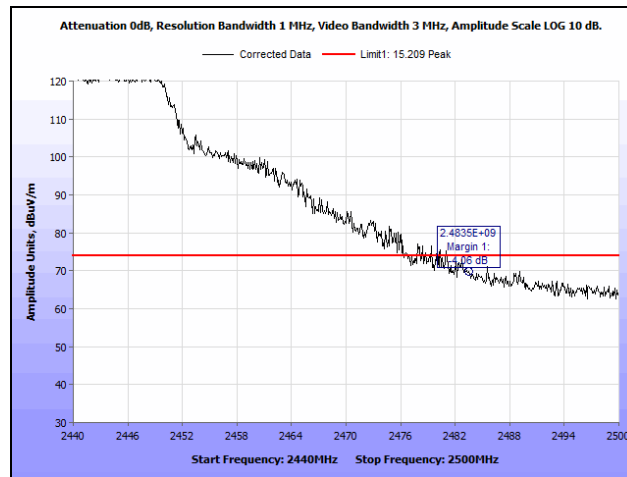
Plot 195. Radiated Restricted Band Edge, 2442 MHz, 802.11g, SISO, Peak
