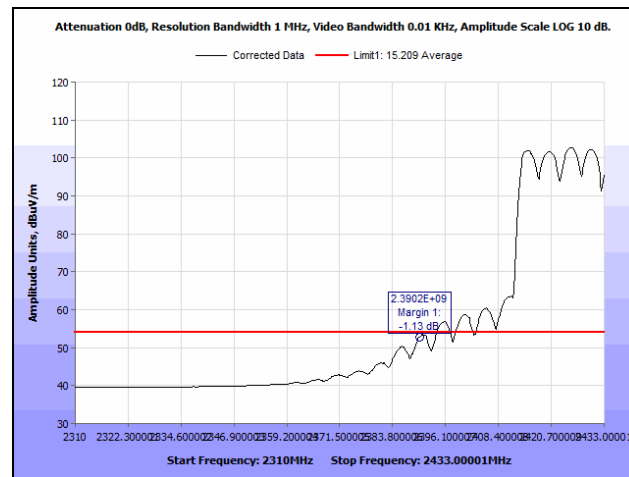
Plot 242. Radiated Restricted Band Edge, 2432 MHz, 802.11n 40 MHz, MIMO, Average
