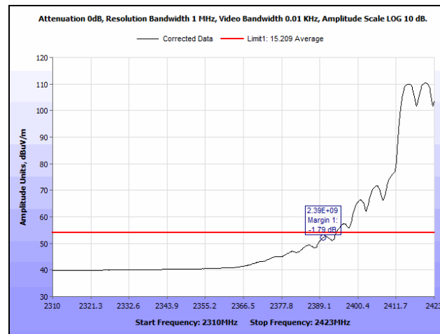
Plot 208. Radiated Restricted Band Edge, 2422 MHz, 802.11n 20 MHz, MIMO, Average
