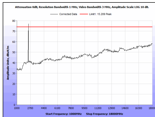
Plot 99. Radiated Spurious Emissions, Mid Channel, 802.11b, 1 GHz – 18 GHz, Peak, MIMO
