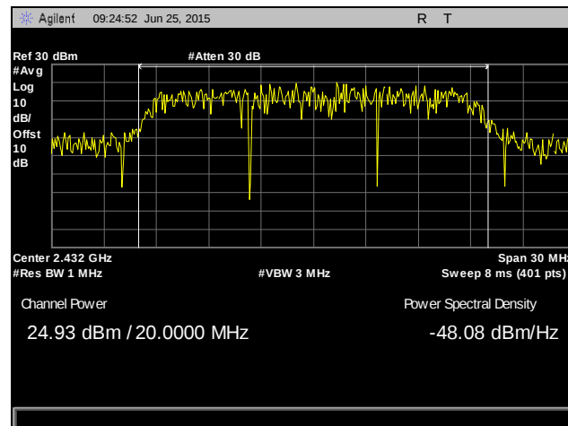
Plot 77. Peak Power Output, 2432 MHz, 802.11n 20 MHz, SISO
