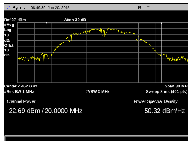
Plot 45. Peak Power Output, High Channel, 802.11b, MIMO, Antenna 1
