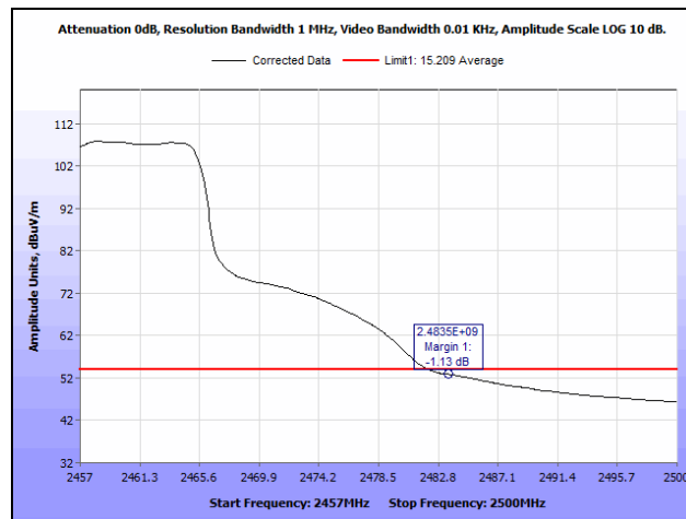
Plot 200. Radiated Restricted Band Edge, 2457 MHz, 802.11g, SISO, Average
