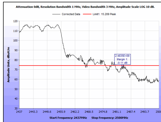
Plot 245. Radiated Restricted Band Edge, 2437 MHz, 802.11n 40 MHz, MIMO, Peak
