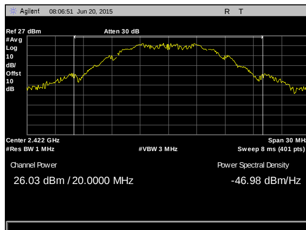
Plot 48. Peak Power Output, 2422 MHz, 802.11b, SISO
