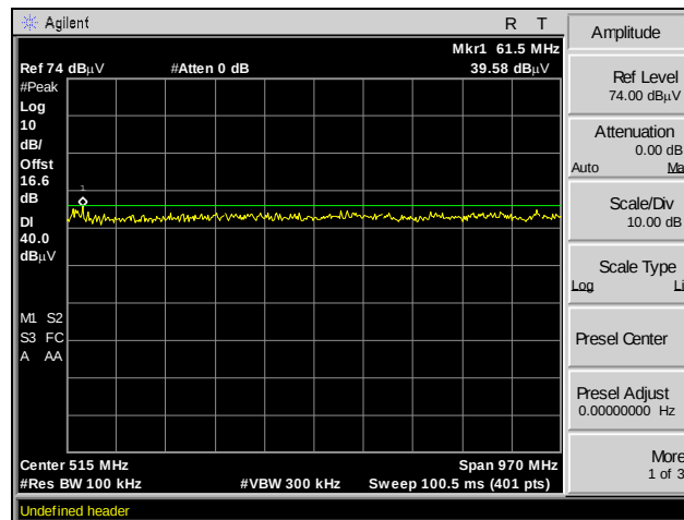
Plot 117. Spurious Emissions, Channel 149, 802.11n 20 MHz, SISO, 30 MHz – 1 GHz
