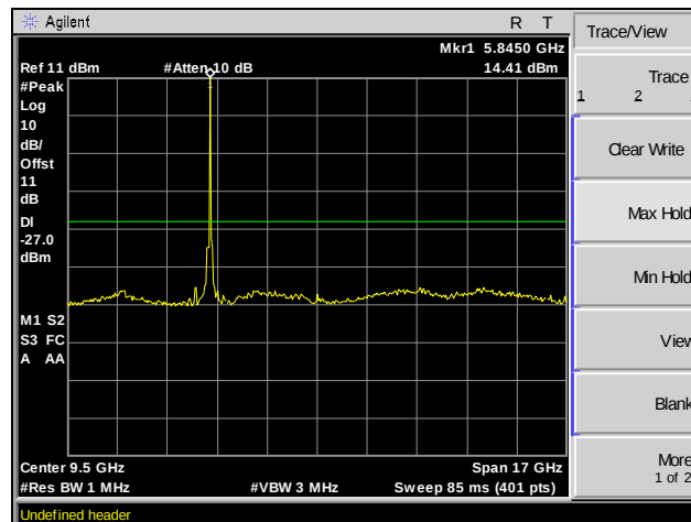
Plot 122. Spurious Emissions, Channel 165, 802.11n 20 MHz, SISO, 1 GHz – 18 GHz
