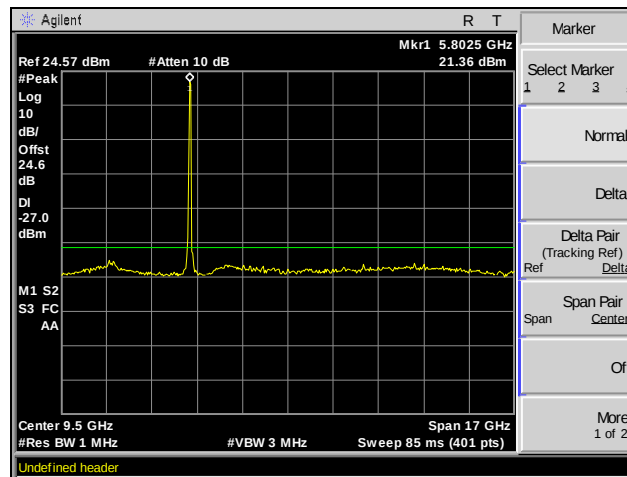
Plot 100. Spurious Emissions, Channel 157, 802.11ac 40 MHz, MIMO, 1 GHz – 18 GHz
