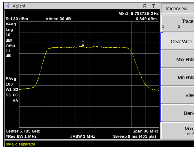
Plot 67. Peak Power Spectral Density, Channel 157, 802.11n 20 MHz, SISO
