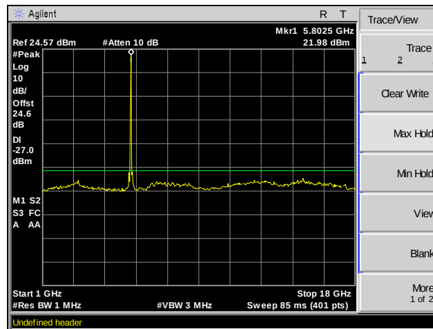
Plot 76. Spurious Emissions, Channel 157, 802.11a 20 MHz, MIMO, 1 GHz – 18 GHz
