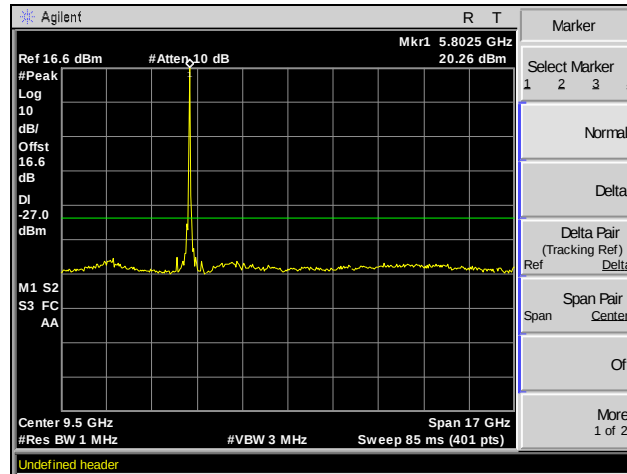
Plot 82. Spurious Emissions, Channel 157, 802.11a 20 MHz, SISO, 1 GHz – 18 GHz
