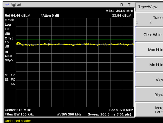
Plot 123. Spurious Emissions, Channel 149, 802.11n 40 MHz, MIMO, 30 MHz – 1 GHz
