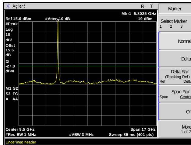
Plot 130. Spurious Emissions, Channel 157, 802.11n 40 MHz, SISO, 1 GHz – 18 GHz
