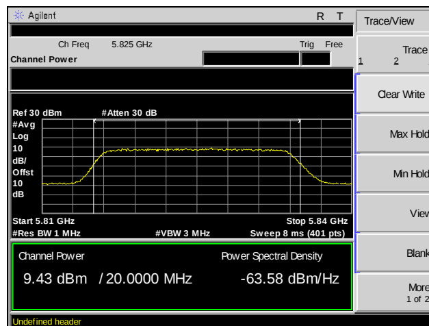
Plot 25. RF Power Output, Channel 165, 802.11ac 20 MHz, MIMO
