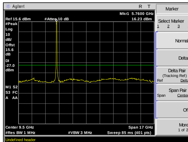
Plot 102. Spurious Emissions, Channel 149, 802.11ac 40 MHz, SISO, 1 GHz – 18 GHz
