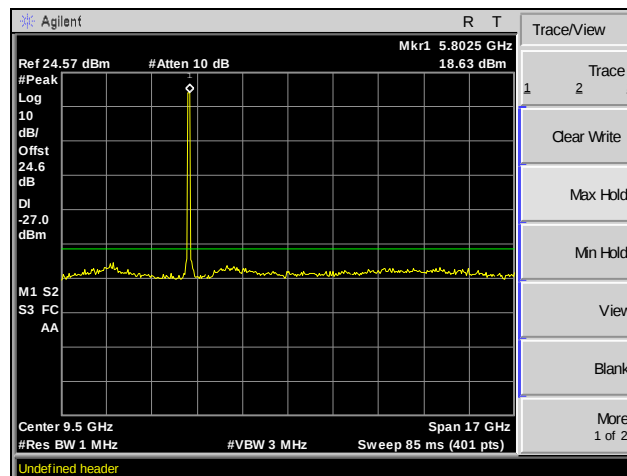
Plot 124. Spurious Emissions, Channel 149, 802.11n 40 MHz, MIMO, 1 GHz – 18 GHz
