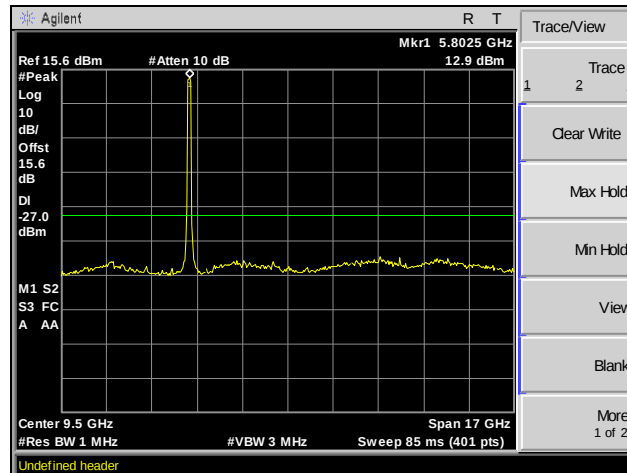
Plot 108. Spurious Emissions, Channel 149, 802.11ac 80 MHz, SISO, 1 GHz – 18 GHz
