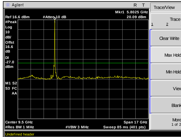
Plot 120. Spurious Emissions, Channel 157, 802.11n 20 MHz, SISO, 1 GHz – 18 GHz
