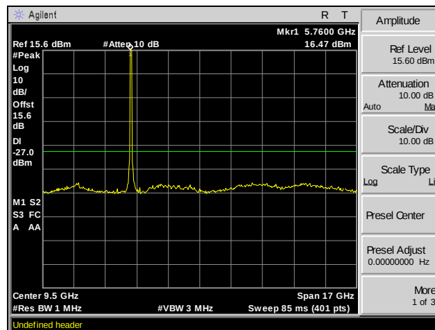
Plot 128. Spurious Emissions, Channel 149, 802.11n 40 MHz, SISO, 1 GHz – 18 GHz
