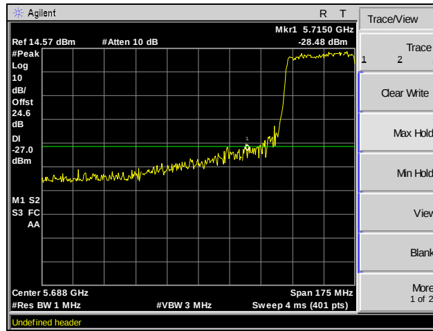
Plot 147. Band Edge, Channel 157, 802.11ac 80 MHz, MIMO
