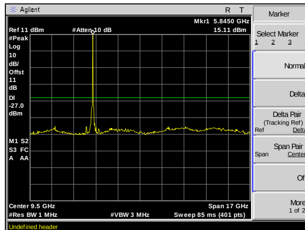
Plot 84. Spurious Emissions, Channel 165, 802.11a 20 MHz, SISO, 1 GHz – 18 GHz
