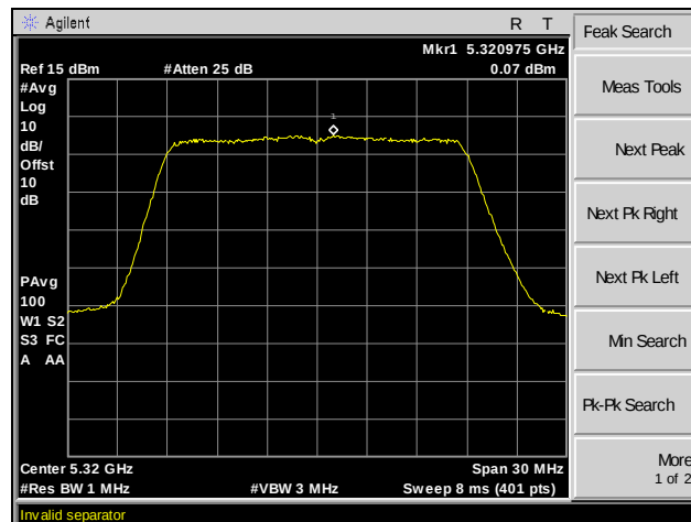
Plot 138. Peak Power Spectral Density, 802.11n 20 MHz, Channel 64, MIMO
