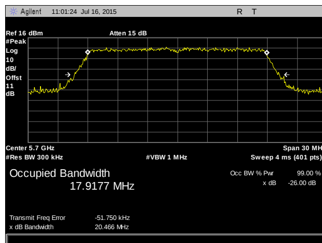
Plot 31. Occupied Bandwidth, 802.11n 20 MHz, 5700 MHz, Port 1
