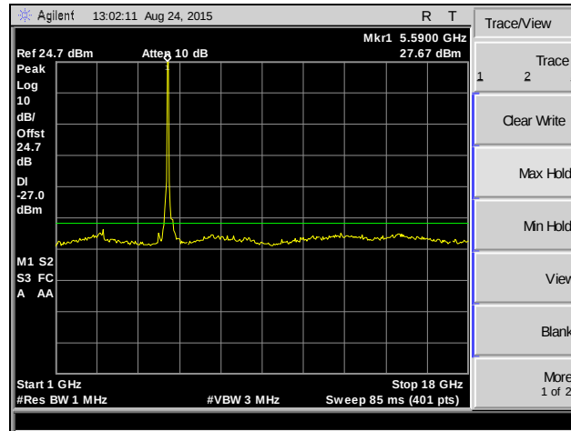
Plot 200. Spurious Emissions, 802.11ac 40 MHz, Channel 116, MIMO
