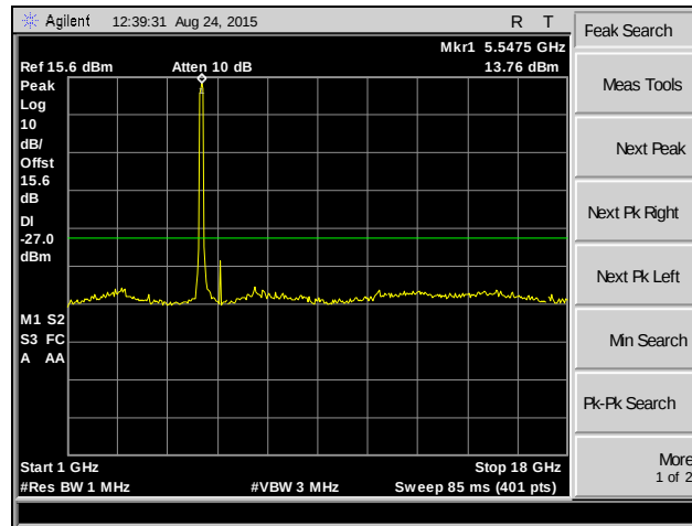
Plot 239. Spurious Emissions, 802.11ac 80 MHz, Channel 100, SISO
