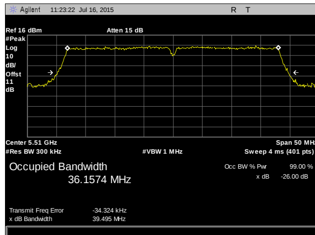
Plot 35. Occupied Bandwidth, 802.11n 40 MHz, 5510 MHz
