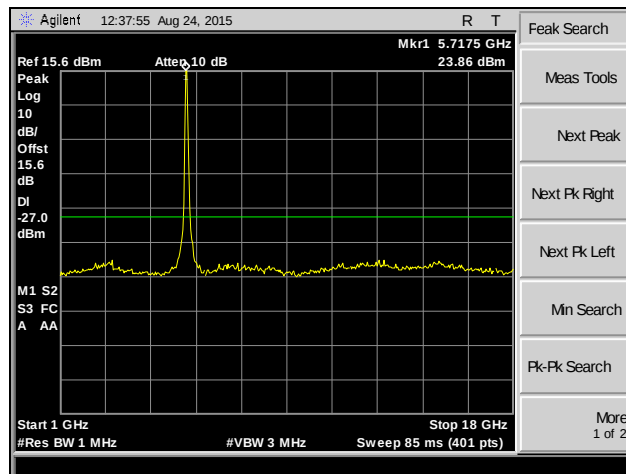
Plot 255. Spurious Emissions, 802.11n 40 MHz, Channel 140, SISO
