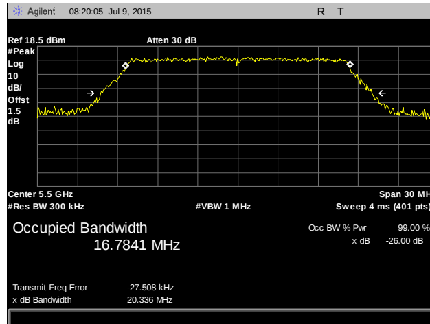
Plot 6. Occupied Bandwidth, 802.11a, 5500 MHz
