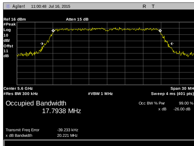
Plot 30. Occupied Bandwidth, 802.11n 20 MHz, 5600 MHz, Port 1
