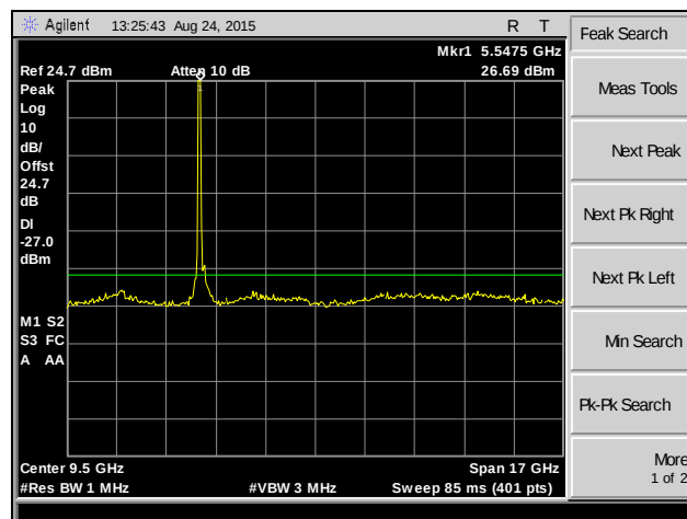
Plot 215. Spurious Emissions, 802.11n 40 MHz, Channel 100, MIMO
