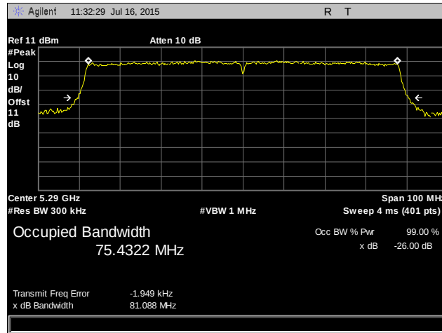
Plot 22. Occupied Bandwidth, 802.11ac 80 MHz, 5290 MHz
