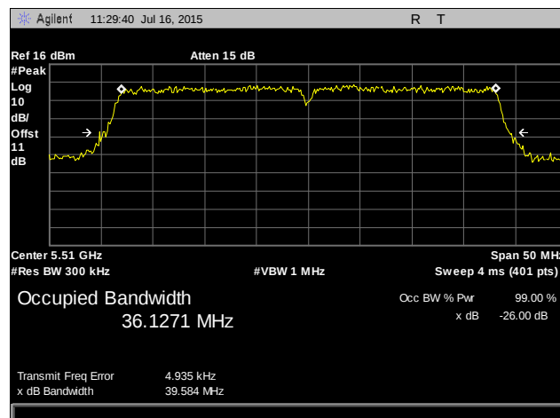
Plot 19. Occupied Bandwidth, 802.11n 40 MHz, 5510 MHz
