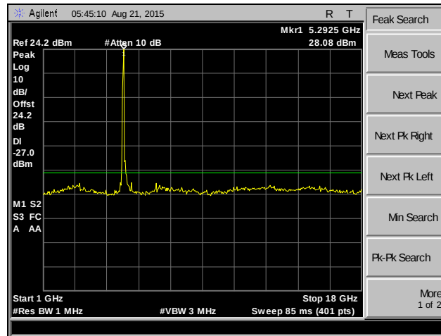
Plot 207. Spurious Emissions, 802.11n 20 MHz, Channel 52, MIMO
