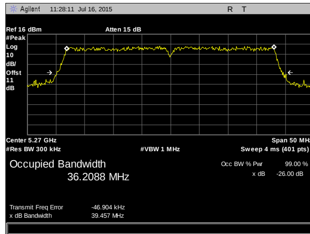
Plot 17. Occupied Bandwidth, 802.11n 40 MHz, 5270 MHz
