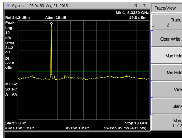
Plot 208. Spurious Emissions, 802.11n 20 MHz, Channel 60, MIMO
