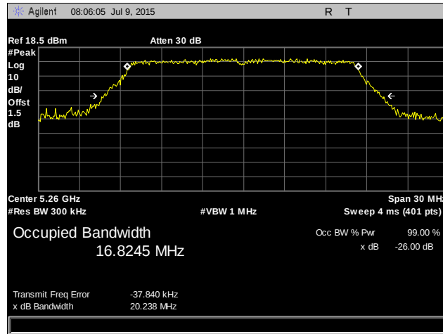
Plot 3. Occupied Bandwidth, 802.11a, 5260 MHz
