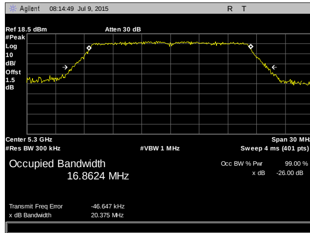
Plot 4. Occupied Bandwidth, 802.11a, 5300 MHz
