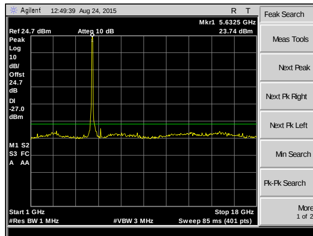
Plot 205. Spurious Emissions, 802.11ac 80 MHz, Channel 124, MIMO
