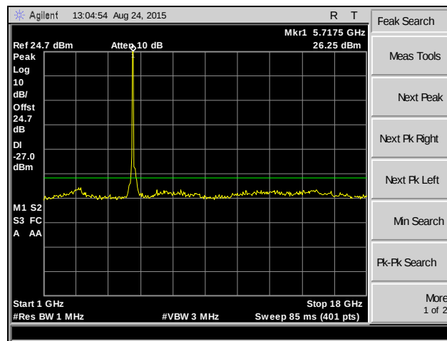
Plot 201. Spurious Emissions, 802.11ac 40 MHz, Channel 132, MIMO
