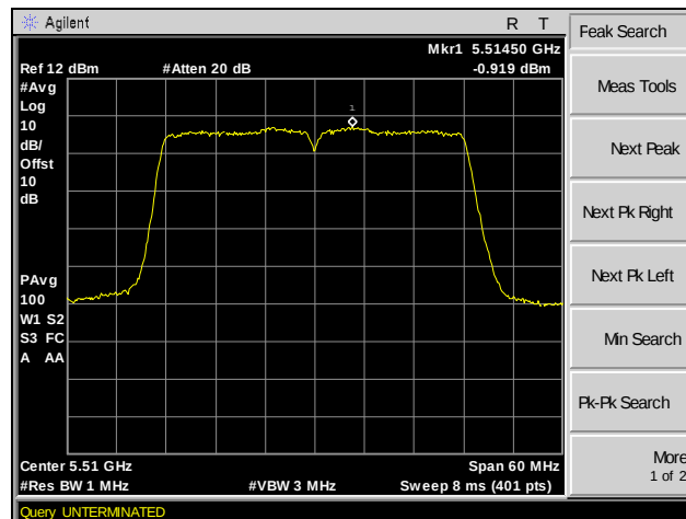
Plot 128. Peak Power Spectral Density, 802.11ac 40 MHz, Channel 100, MIMO
