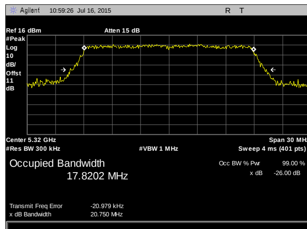
Plot 28. Occupied Bandwidth, 802.11n 20 MHz, 5320 MHz, Port 1
