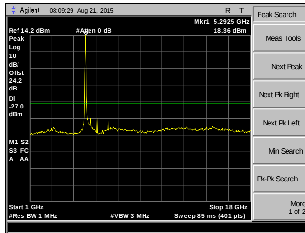
Plot 213. Spurious Emissions, 802.11n 40 MHz, Channel 52, MIMO
