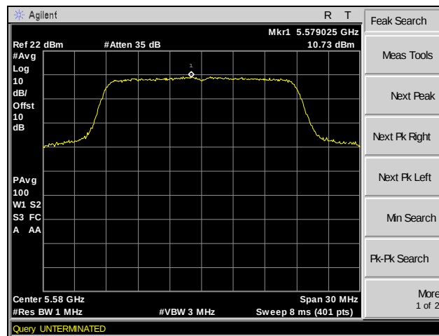
Plot 159. Peak Power Spectral Density, 802.11ac 20 MHz, Channel 116, SISO
