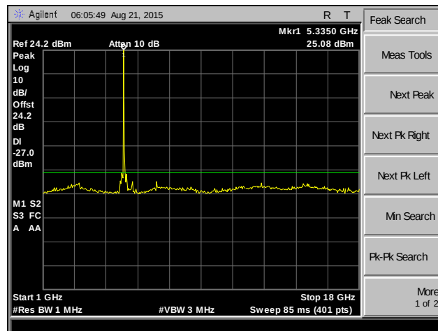
Plot 209. Spurious Emissions, 802.11n 20 MHz, Channel 64, MIMO
