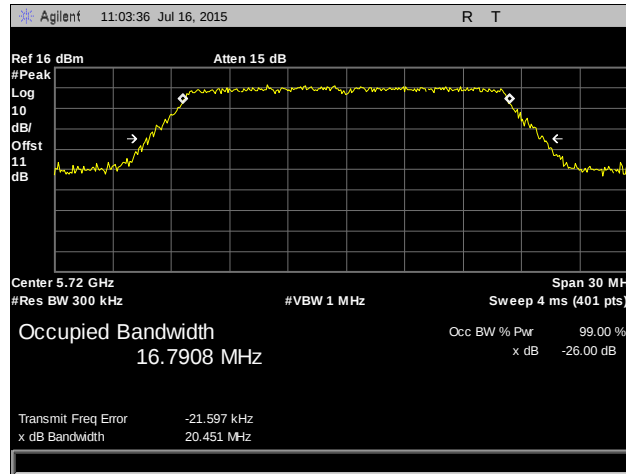
Plot 9. Occupied Bandwidth, 802.11a, 5720 MHz
