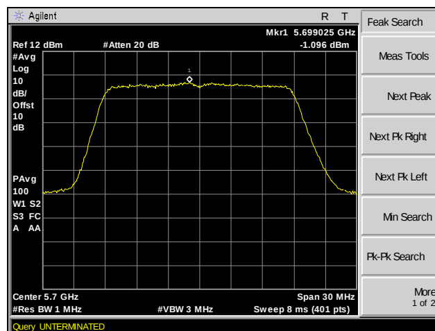
Plot 141. Peak Power Spectral Density, 802.11n 20 MHz, Channel 140, MIMO
