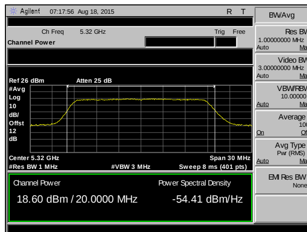
Plot 101. RF Output Power, 802.11n 20 MHz, Channel 64, SISO
