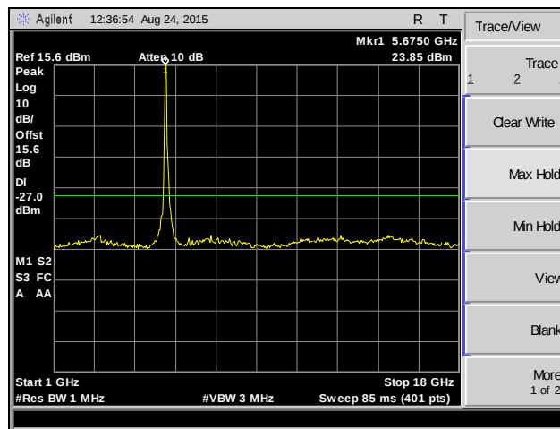
Plot 254. Spurious Emissions, 802.11n 40 MHz, Channel 132, SISO
