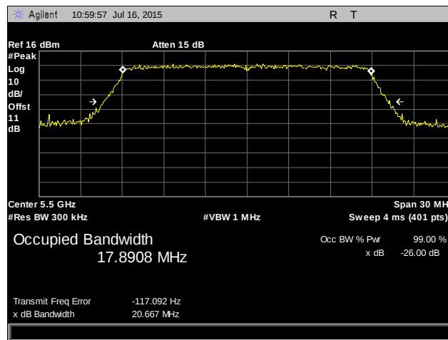
Plot 29. Occupied Bandwidth, 802.11n 20 MHz, 5500 MHz, Port 1
