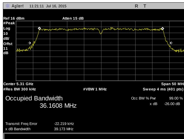
Plot 34. Occupied Bandwidth, 802.11n 40 MHz, 5310 MHz
