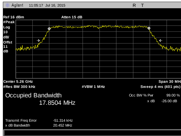
Plot 10. Occupied Bandwidth, 802.11ac 20 MHz, 5260 MHz, Port 1
