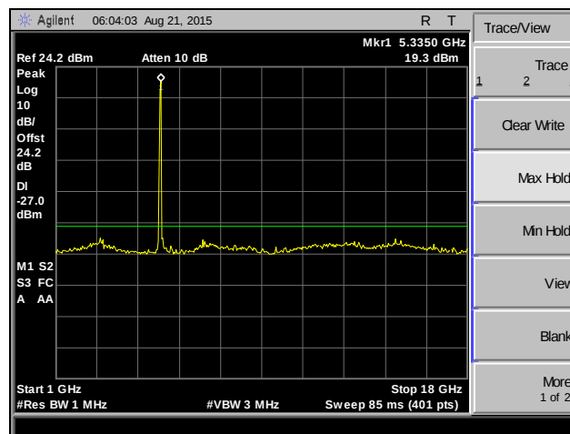
Plot 192. Spurious Emissions, 802.11ac 20 MHz, Channel 60, MIMO
