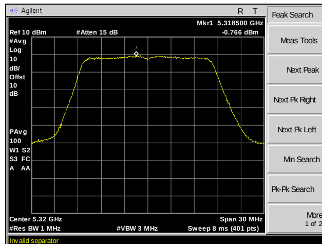
Plot 114. Peak Power Spectral Density, 802.11a, Channel 64, MIMO
