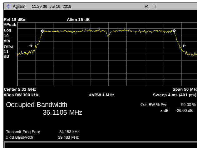
Plot 18. Occupied Bandwidth, 802.11n 40 MHz, 5310 MHz
