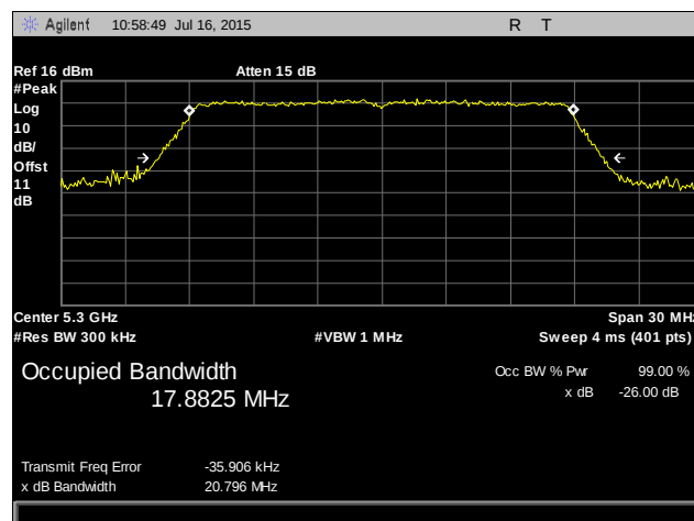
Plot 27. Occupied Bandwidth, 802.11n 20 MHz, 5300 MHz, Port 1
