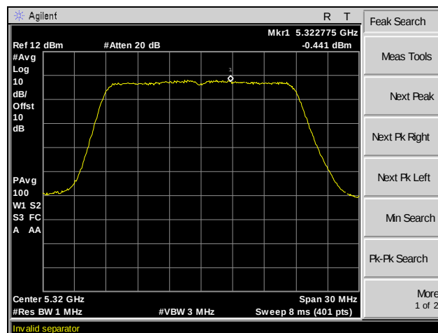
Plot 121. Peak Power Spectral Density, 802.11ac 20 MHz, Channel 64, MIMO
