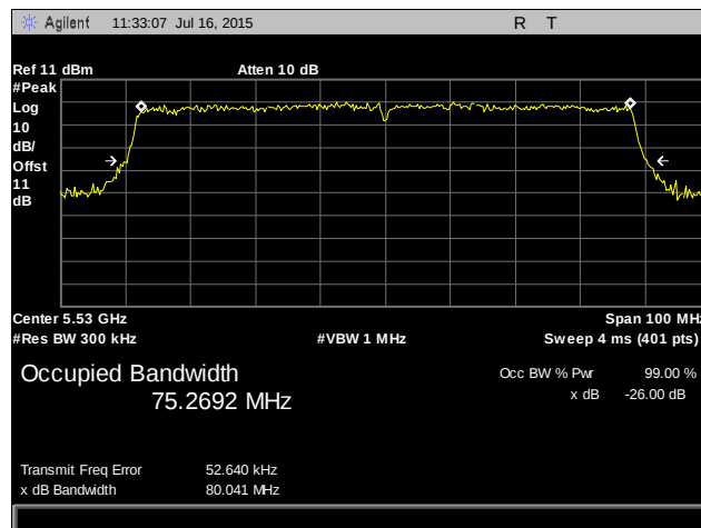
Plot 23. Occupied Bandwidth, 802.11ac 80 MHz, 5530 MHz
