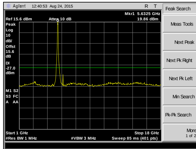
Plot 240. Spurious Emissions, 802.11ac 80 MHz, Channel 116, SISO
