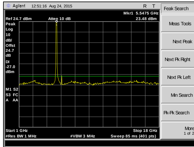
Plot 203. Spurious Emissions, 802.11ac 80 MHz, Channel 100, MIMO
