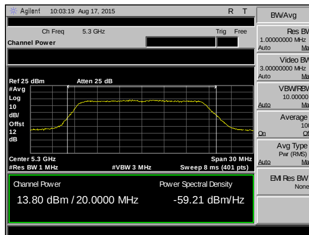
Plot 76. RF Output Power, 802.11a, Channel 60, SISO
