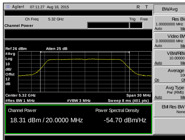
Plot 77. RF Output Power, 802.11a, Channel 64, SISO
