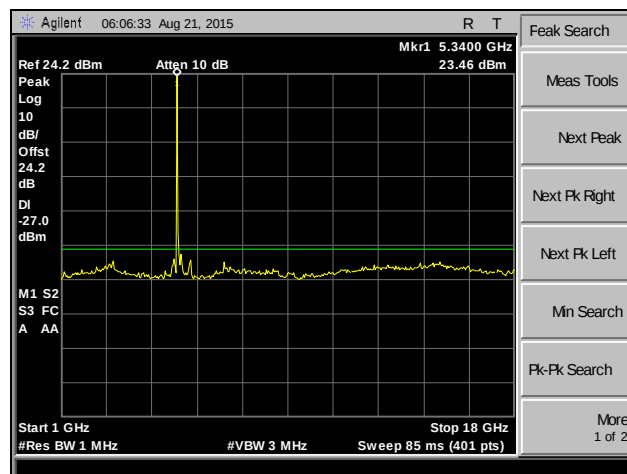
Plot 193. Spurious Emissions, 802.11ac 20 MHz, Channel 64, MIMO
