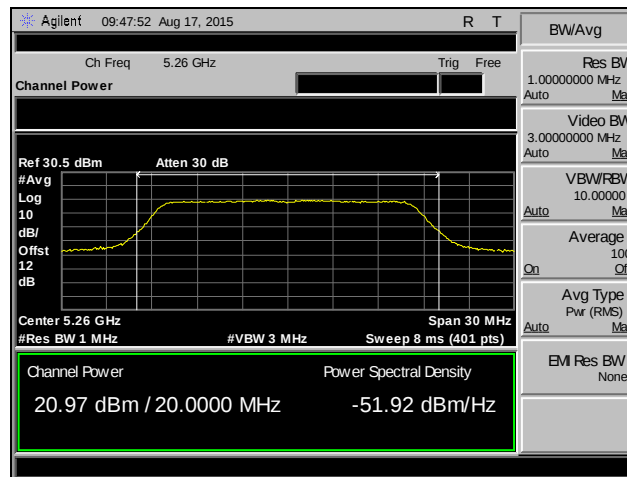
Plot 75. RF Output Power, 802.11a, Channel 52, SISO
