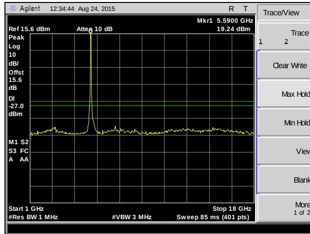
Plot 236. Spurious Emissions, 802.11ac 40 MHz, Channel 116, SISO
