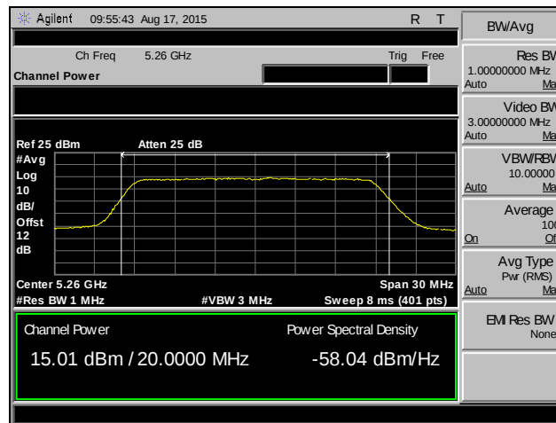
Plot 38. RF Output Power, 802.11a, Channel 52, MIMO
