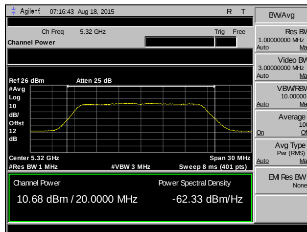
Plot 40. RF Output Power, 802.11a, Channel 64, MIMO
