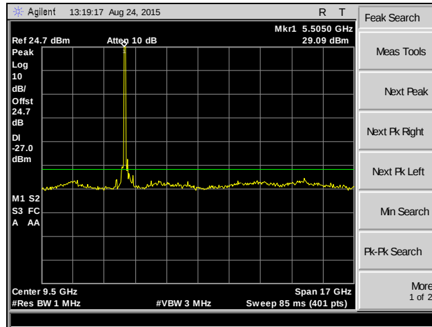
Plot 210. Spurious Emissions, 802.11n 20 MHz, Channel 100, MIMO
