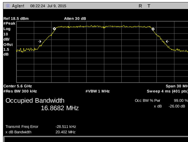
Plot 7. Occupied Bandwidth, 802.11a, 5600 MHz
