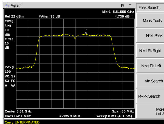
Plot 164. Peak Power Spectral Density, 802.11ac 40 MHz, Channel 100, SISO
