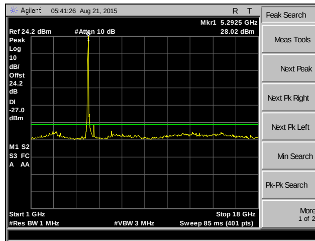
Plot 191. Spurious Emissions, 802.11ac 20 MHz, Channel 52, MIMO
