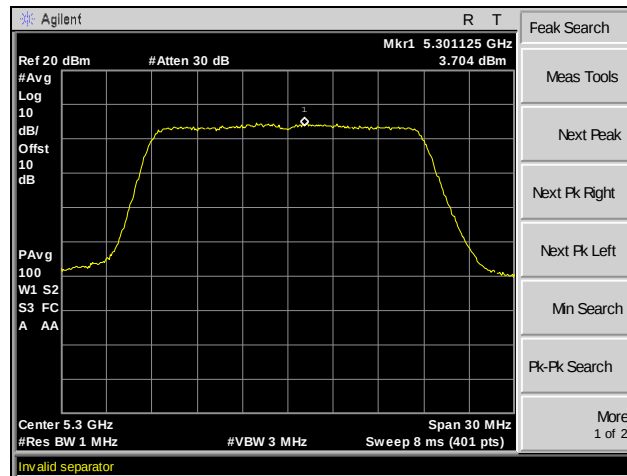
Plot 173. Peak Power Spectral Density, 802.11n 20 MHz, Channel 60, SISO
