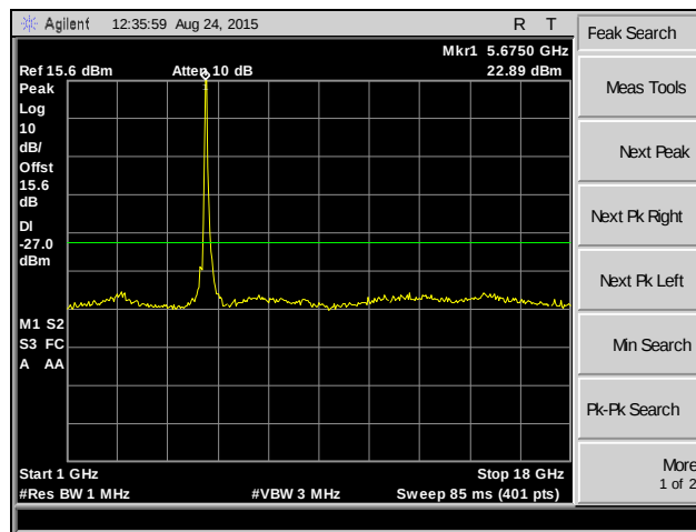
Plot 237. Spurious Emissions, 802.11ac 40 MHz, Channel 132, SISO
