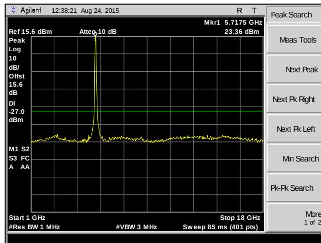
Plot 238. Spurious Emissions, 802.11ac 40 MHz, Channel 140, SISO
