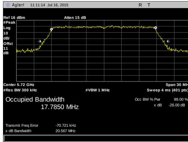
Plot 16. Occupied Bandwidth, 802.11ac 20 MHz, 5720 MHz, Port 1
