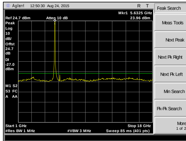
Plot 204. Spurious Emissions, 802.11ac 80 MHz, Channel 116, MIMO
