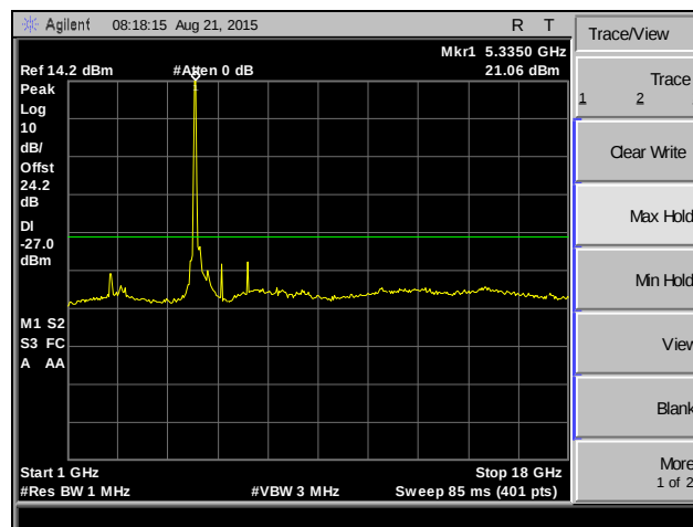
Plot 214. Spurious Emissions, 802.11n 40 MHz, Channel 60, MIMO
