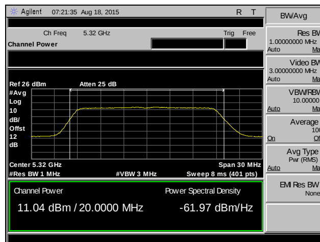
Plot 64. RF Output Power, 802.11n 20 MHz, Channel 64, MIMO
