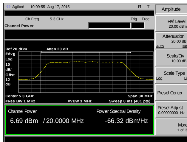
Plot 39. RF Output Power, 802.11a, Channel 60, MIMO
