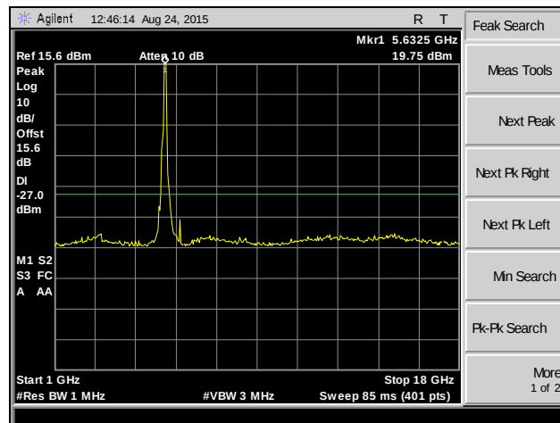
Plot 241. Spurious Emissions, 802.11ac 80 MHz, Channel 124, SISO
