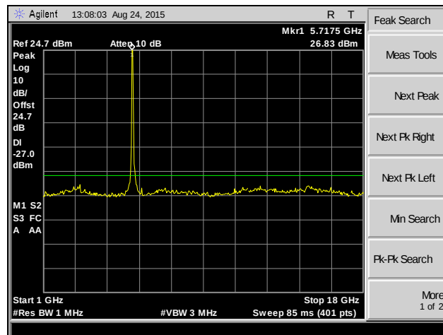
Plot 202. Spurious Emissions, 802.11ac 40 MHz, Channel 140, MIMO
