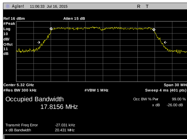
Plot 12. Occupied Bandwidth, 802.11ac 20 MHz, 5320 MHz, Port 1
