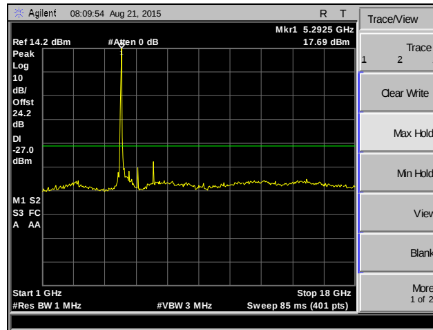
Plot 197. Spurious Emissions, 802.11ac 40 MHz, Channel 52, MIMO
