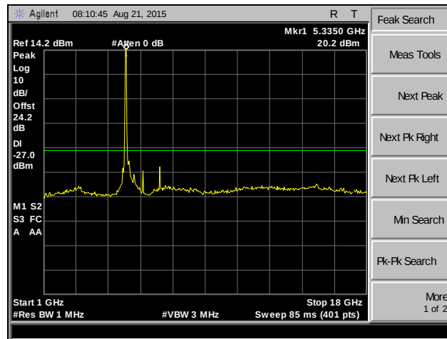
Plot 198. Spurious Emissions, 802.11ac 40 MHz, Channel 60, MIMO
