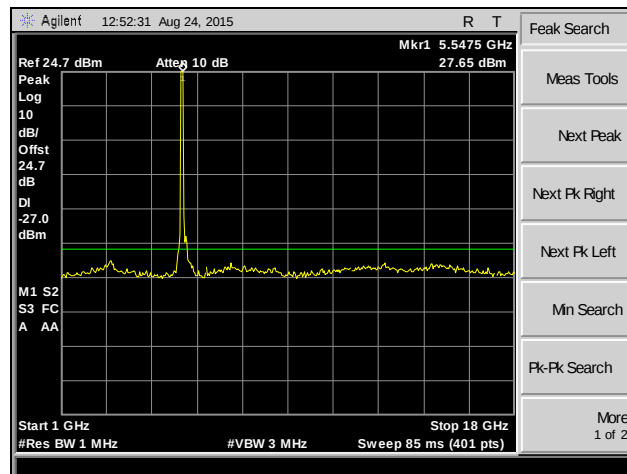
Plot 199. Spurious Emissions, 802.11ac 40 MHz, Channel 100, MIMO
