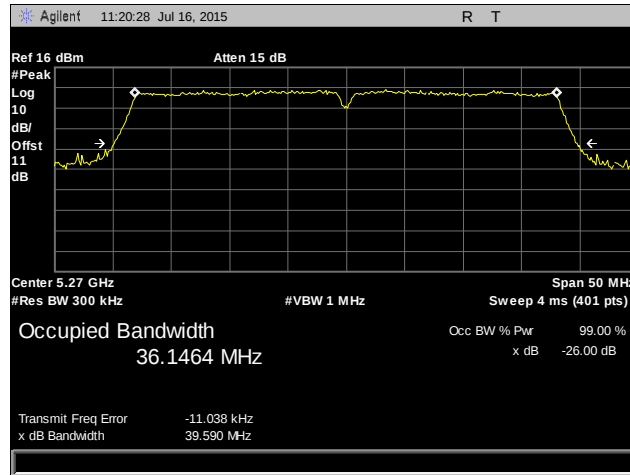
Plot 33. Occupied Bandwidth, 802.11n 40 MHz, 5270 MHz
