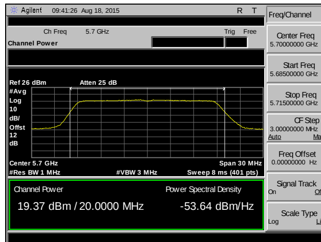
Plot 87. RF Output Power, 802.11ac 20 MHz, Channel 140, SISO
