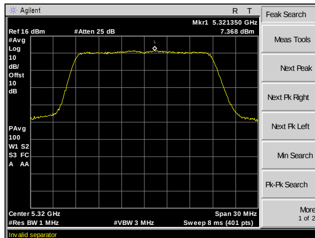
Plot 157. Peak Power Spectral Density, 802.11ac 20 MHz, Channel 64, SISO
