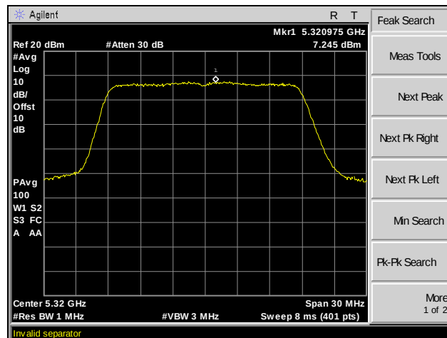
Plot 174. Peak Power Spectral Density, 802.11n 20 MHz, Channel 64, SISO
