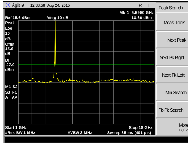
Plot 253. Spurious Emissions, 802.11n 40 MHz, Channel 116, SISO
