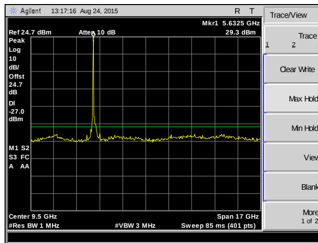
Plot 211. Spurious Emissions, 802.11n 20 MHz, Channel 120, MIMO
