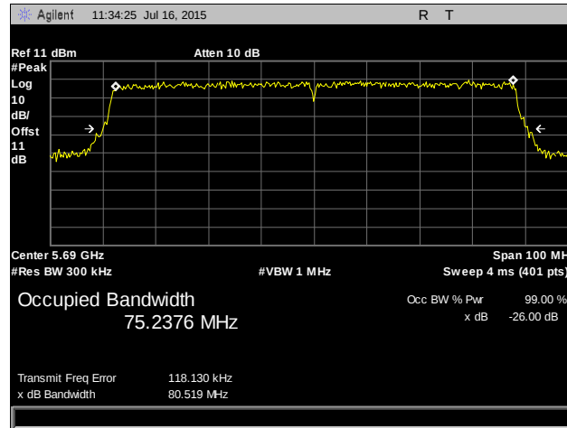
Plot 25. Occupied Bandwidth, 802.11ac 80 MHz, 5690 MHz
