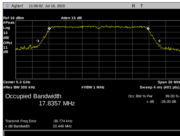
Plot 11. Occupied Bandwidth, 802.11ac 20 MHz, 5300 MHz, Port 1
