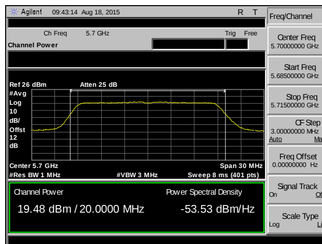
Plot 104. RF Output Power, 802.11n 20 MHz, Channel 140, SISO
