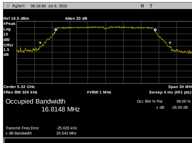
Plot 5. Occupied Bandwidth, 802.11a, 5320 MHz
