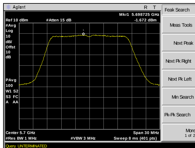
Plot 117. Peak Power Spectral Density, 802.11a, Channel 140, MIMO
