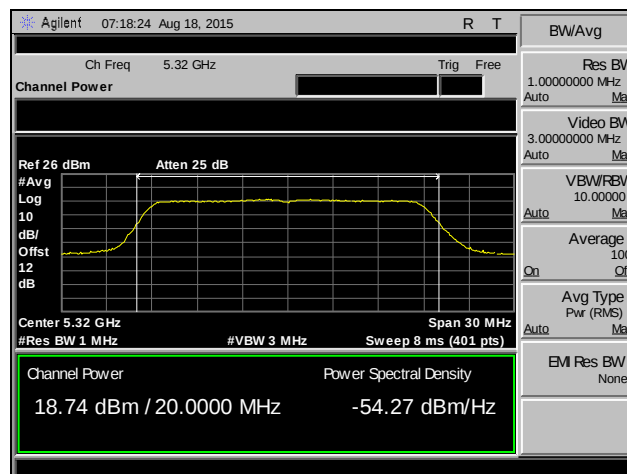
Plot 84. RF Output Power, 802.11ac 20 MHz, Channel 64, SISO
