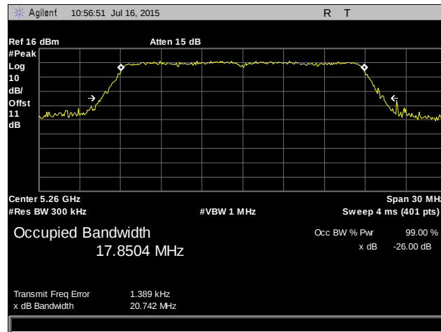
Plot 26. Occupied Bandwidth, 802.11n 20 MHz, 5260 MHz, Port 1
