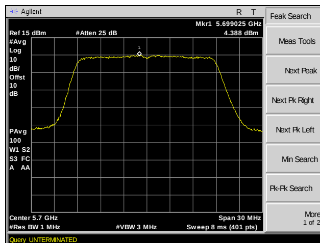
Plot 160. Peak Power Spectral Density, 802.11ac 20 MHz, Channel 140, SISO
