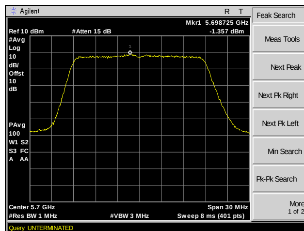
Plot 124. Peak Power Spectral Density, 802.11ac 20 MHz, Channel 140, MIMO
