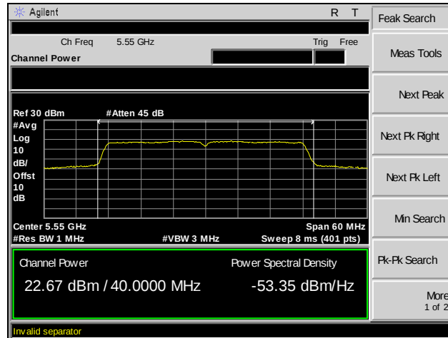
Plot 92. RF Output Power, 802.11ac 40 MHz, Channel 108, SISO
