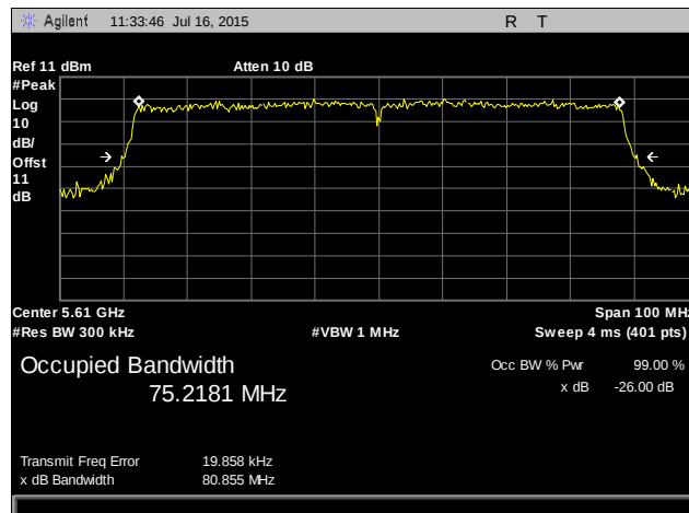
Plot 24. Occupied Bandwidth, 802.11ac 80 MHz, 5610 MHz
