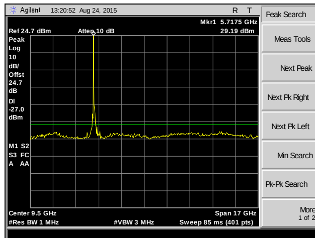
Plot 212. Spurious Emissions, 802.11n 20 MHz, Channel 140, MIMO
