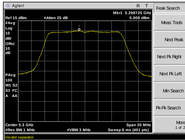
Plot 150. Peak Power Spectral Density, 802.11a, Channel 60, SISO
