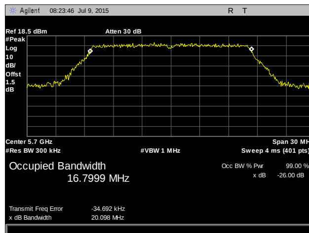
Plot 8. Occupied Bandwidth, 802.11a, 5700 MHz
