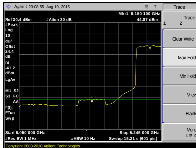
Plot 158. Band Edge, 802.11ac 40 MHz, MIMO, Channel 44, Average
