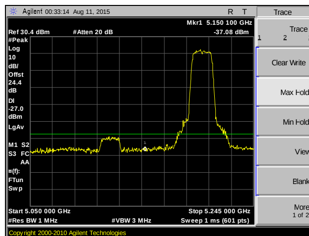
Plot 105. Band Edge, 802.11a 20 MHz, MIMO, Channel 40, Peak
