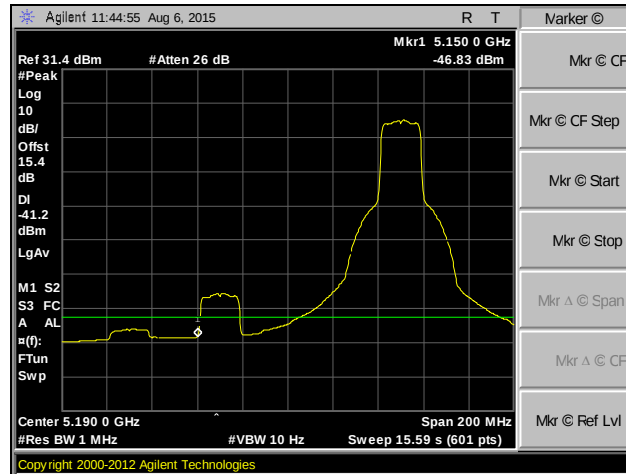
Plot 126. Band Edge, 802.11a 20 MHz, SISO, Channel 48, Average
