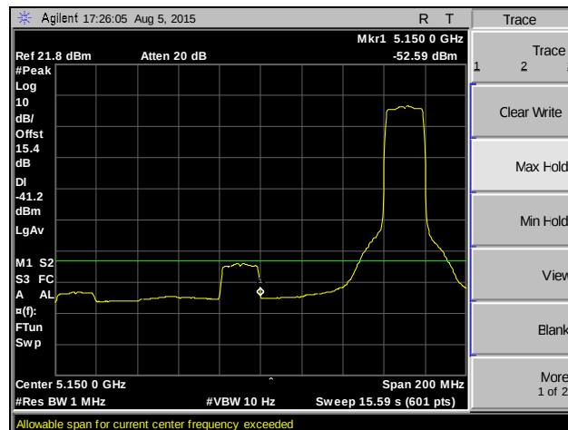
Plot 190. Band Edge, 802.11n 20 MHz, SISO, Channel 44, Average
