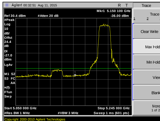
Plot 133. Band Edge, 802.11ac 20 MHz, MIMO, Channel 40, Peak
