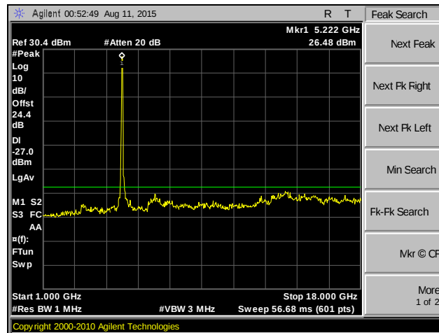
Plot 99. Spurious Emissions, 802.11n 40 MHz, SISO, High Channel
