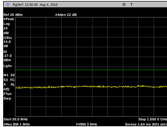
Plot 71. Spurious Emissions, Worst Case Emission Plot, 30 MHz – 1 GHz
