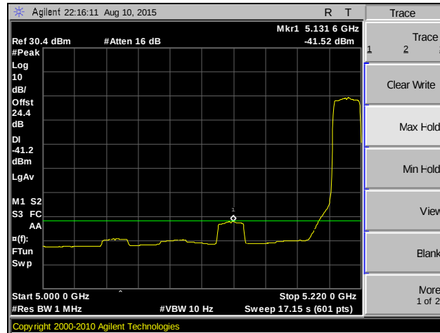
Plot 174. Band Edge, 802.11n 20 MHz, MIMO, Channel 42, Average
