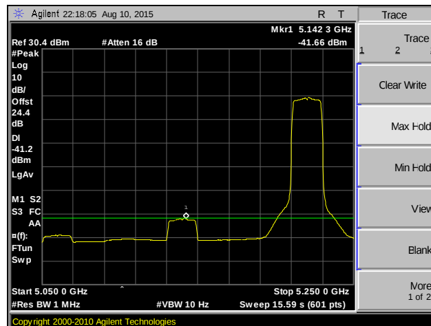
Plot 176. Band Edge, 802.11n 20 MHz, MIMO, Channel 44, Average
