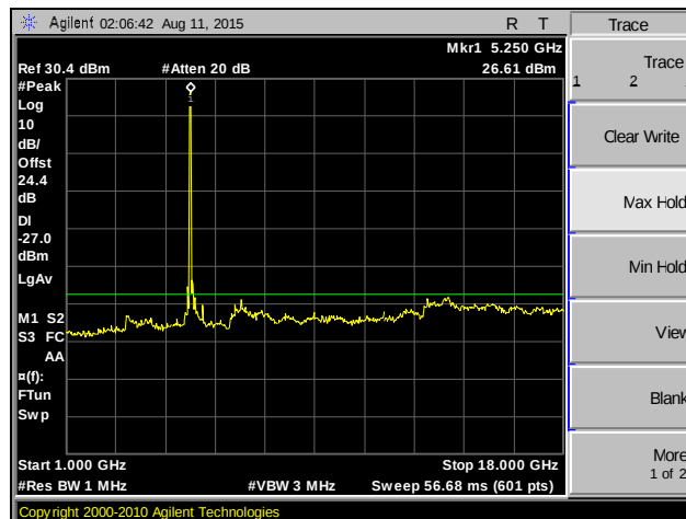
Plot 92. Spurious Emissions, 802.11n 20 MHz, MIMO, High Channel
