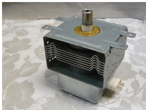
Magnetron View
