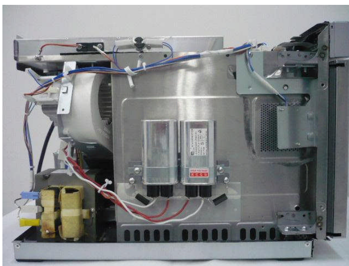
Left Side View without Enclosure
