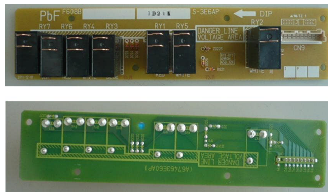
Top and Bottom View of Power Relay Board
