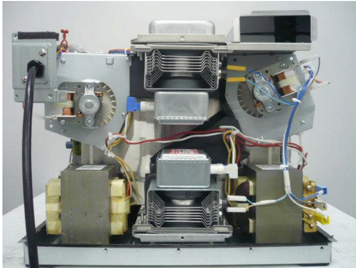
Rear View without Enclosure
