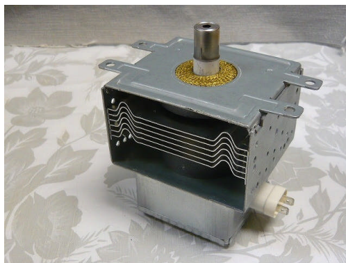
Magnetron View
