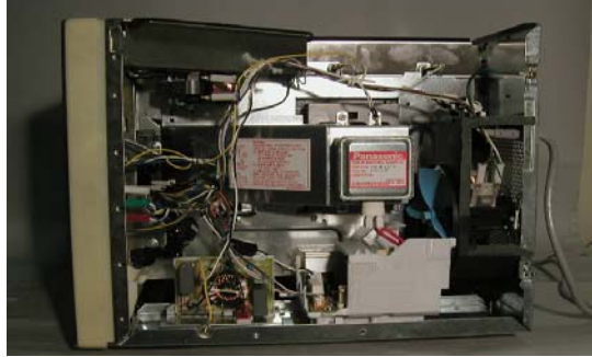
Exhibit 2-D2: Right Side View of Model MCEW With Enclosure Removed
