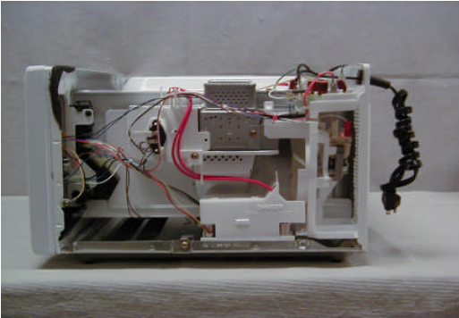
Exhibit: B3 NN-H765 Right side view, No enclosure
