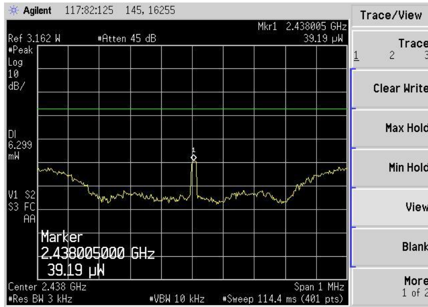
Plot 19 – Channel 1
