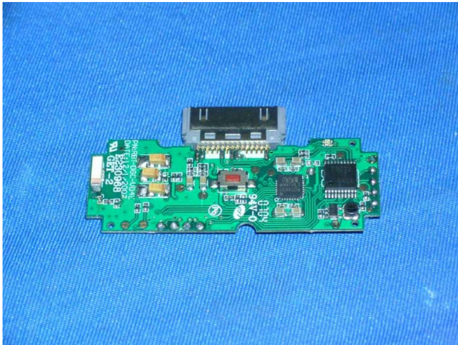
Bluetooth Dongle Main PCB comp side
