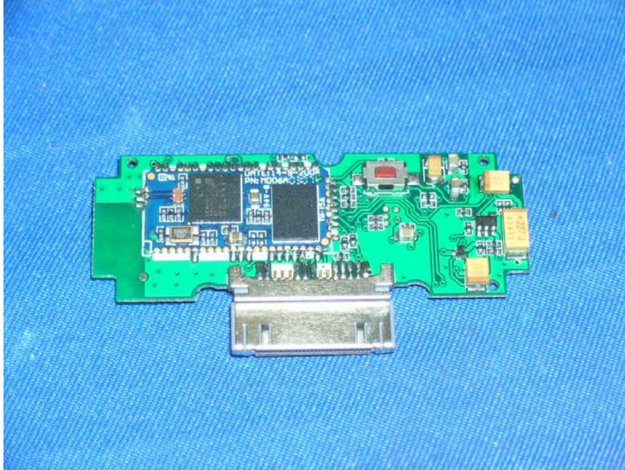
Bluetooth Dongle Main PCB solder side
