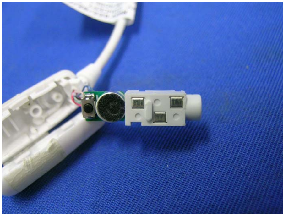
Power On/Off button, Mic, & 3.5mm Earphone Jack PCB front side
