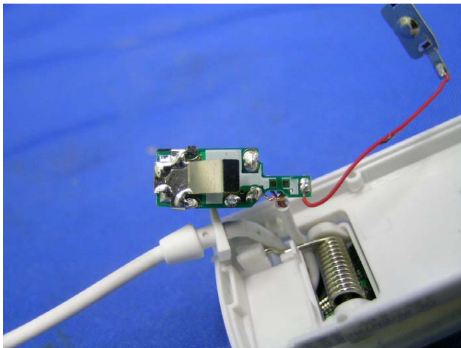
AC Jack PCB rear side
