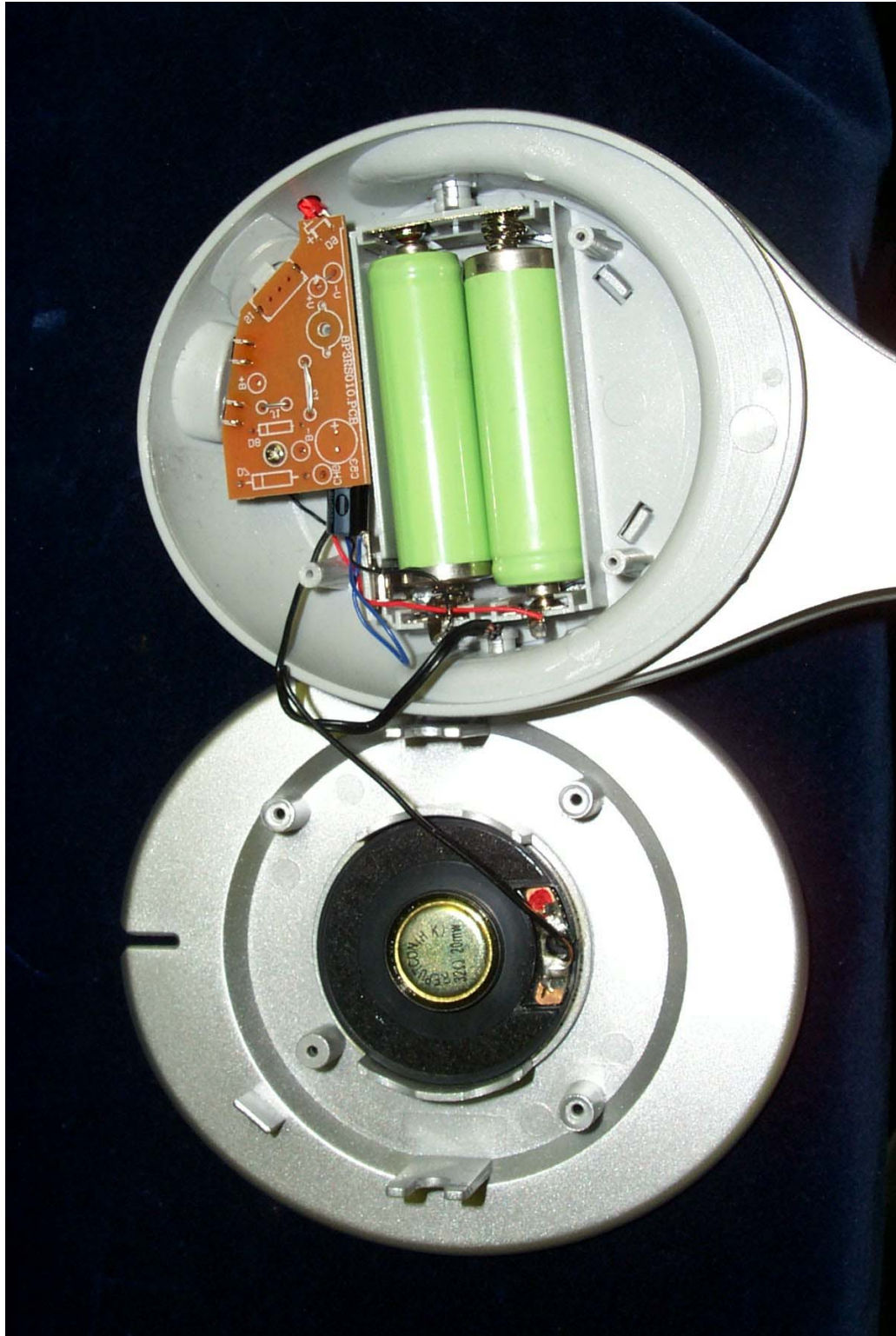
Figure 7.3 Left Side Open View
