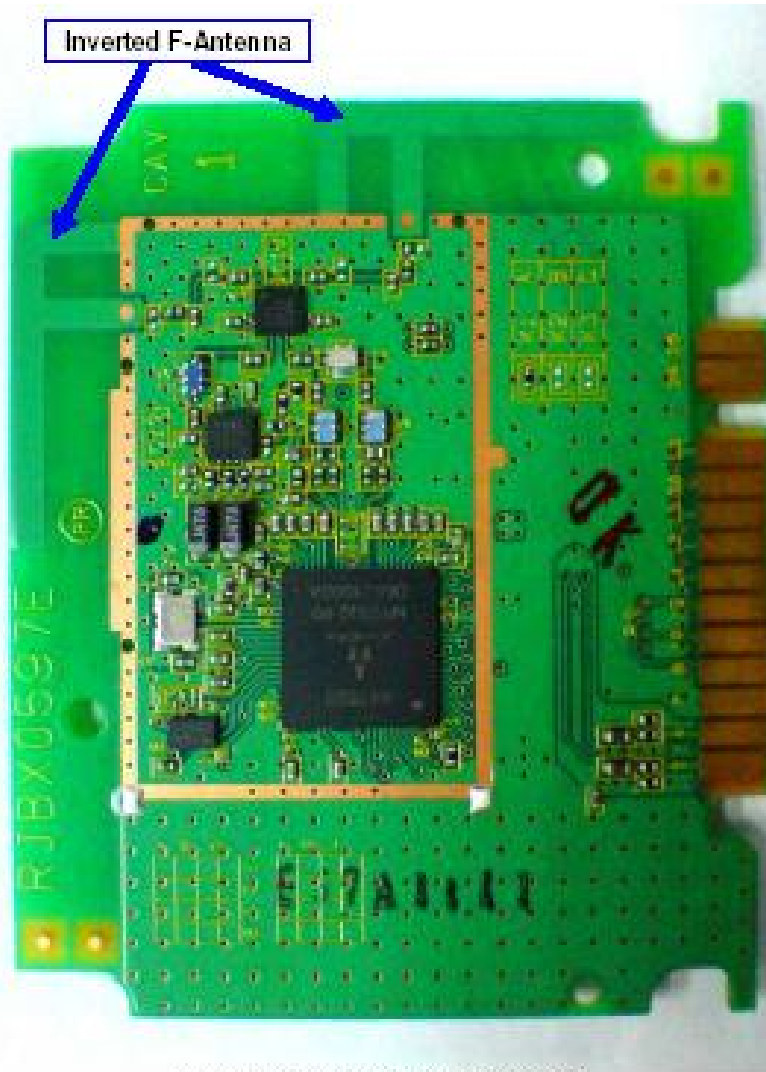
RF Module Circuit with RF Shield Removed
